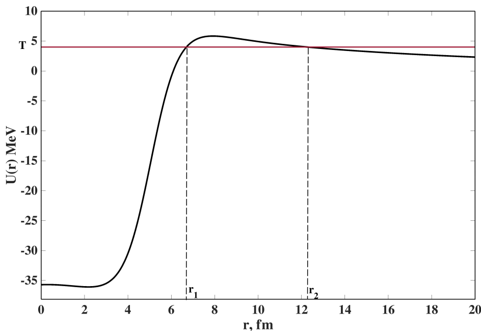
Figure 2.4: The combined Coulomb and nuclear potential of a nucleus [18].
