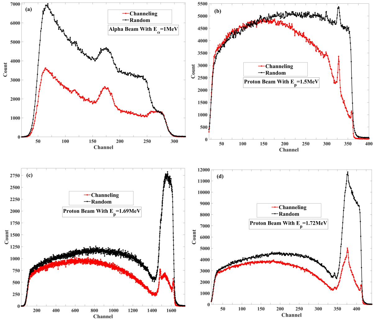
Figure 5.7: The comparison between channelling and random peak at different with a) alpha beam with E_\alpha = 1\text{ MeV} , and proton beam with b) E_p = 1.5\text{ MeV} , c) E_p = 1.69\text{ MeV} and d) E_p = 1.72\text{ MeV} .
