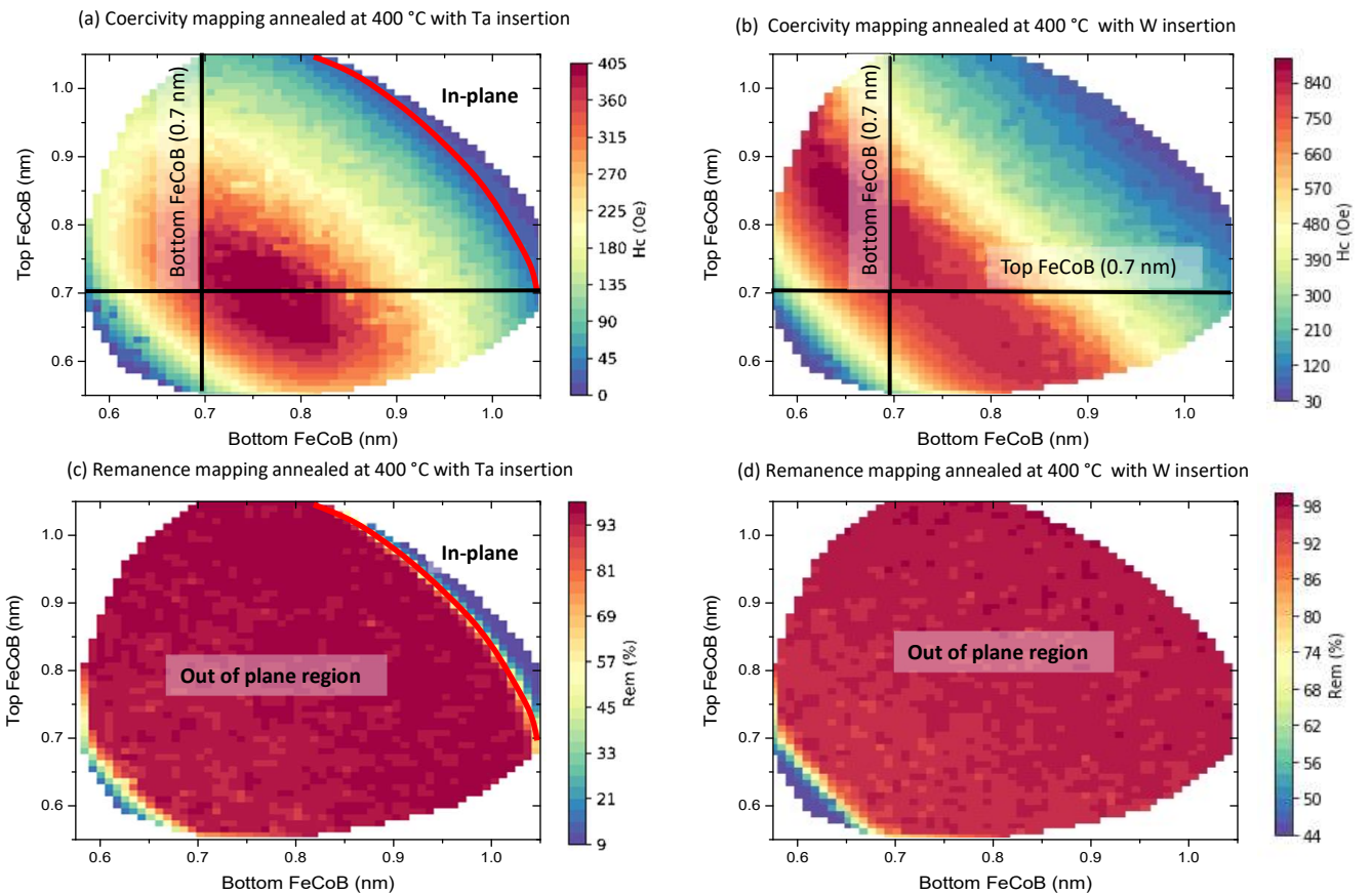
Figure. 4.6: (a)-(b) Coercivity and (c)-(d) remanent magnetization mappings-extracted for samples with composite free layer as in figure.4.5 after 400 °C annealing.
