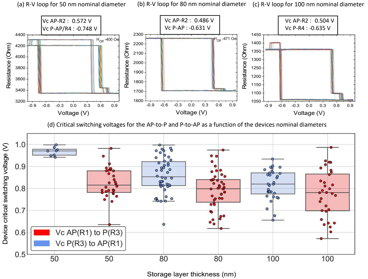
Figure. 4.22: Measured R-V loops for nominal diameters of (a) 50,(b) 80 and (c) 100 nm.(d) Critical switching voltages for the AP-toP and P-to-AP as a function of the devices nominal diameters.
