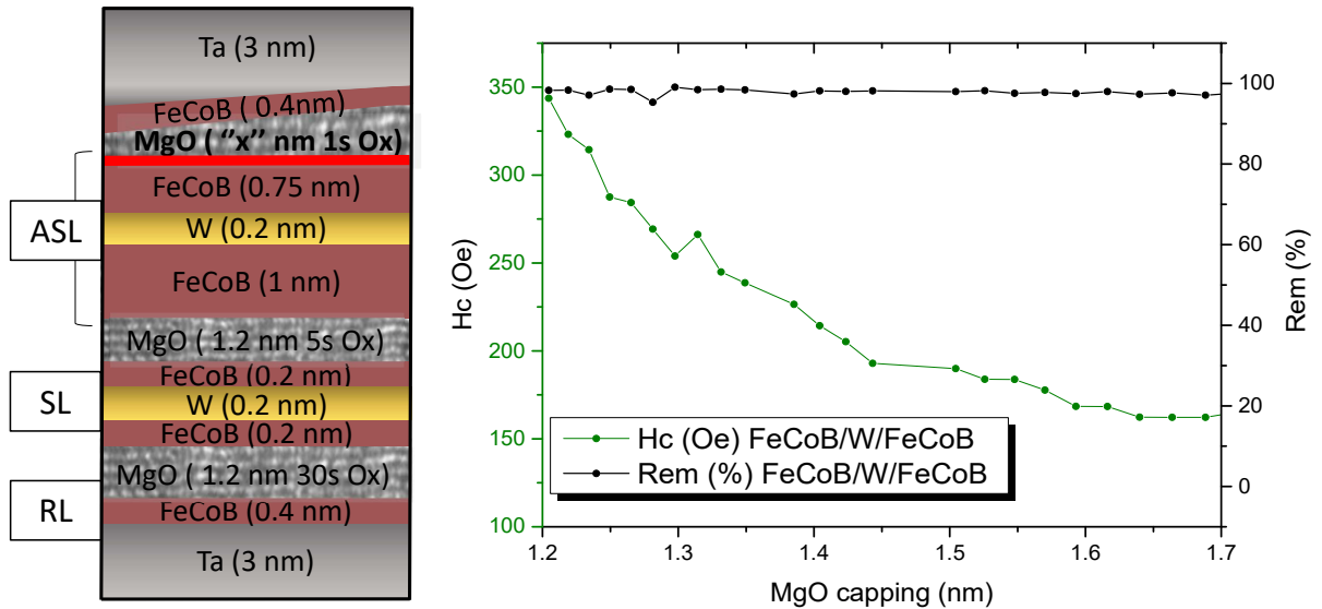
Capping MgO wedge in half ASL/SL MTJ stack and Remanence/Coercivity vs MgO capping thickness
