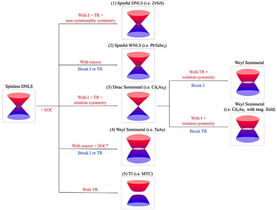
Fig. 1.3 – Diagram of the different topological states and their relationship with each other. The symmetries in red (blue) captions indicate the global symmetry or spatial/lattice symmetry elements that need to be preserved (broken) to obtain a different topological phase. From [72]
