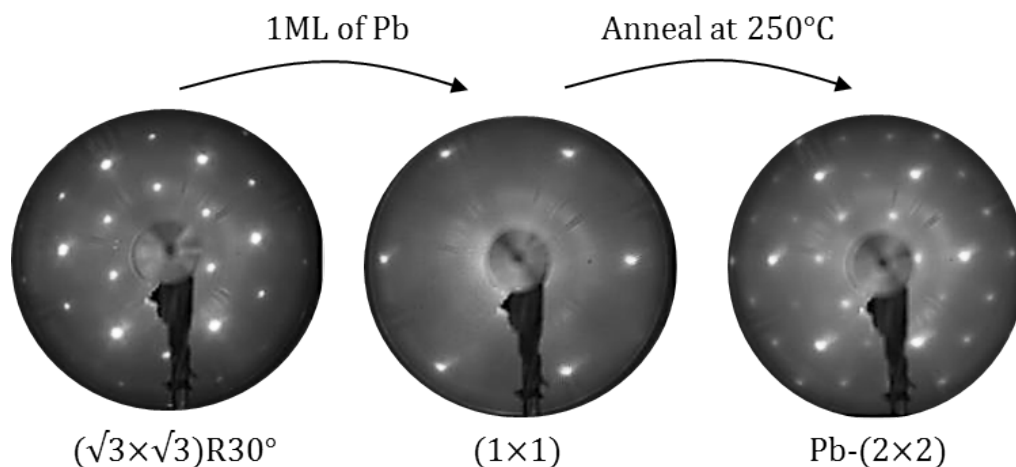
Fig. 5.5 – Phase diagram of Pb evaporation on SiC (\sqrt{3} \times \sqrt{3})R30^\circ . Evaporation of 1 ML at room temperature covers the surface reconstruction. After an anneal at 250^\circ\text{C} , a (2 \times 2) periodicity appears. Pictures taken at 100 eV, 80 eV and 110 eV respectively.
