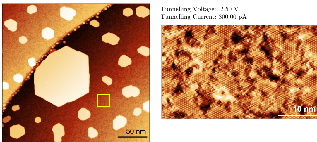
Fig. 5.7 – STM images of Pb/SiC (2 \times 2) reconstruction. On the large scale image, the formation of Pb 3D islands is observed. On the small scale image, measured in the yellow square area, we observe the atomic resolution of the Pb induced (2 \times 2) phase. Images provided by A. Malecot.
