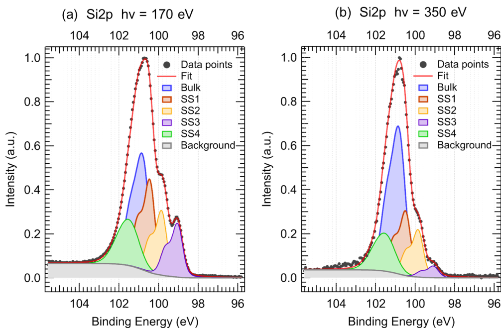
Fig. 5.12 – \text{Si}2p core level of ML of Pb on \text{SiC}-(\sqrt{3}\times\sqrt{3})R30^\circ measured at (a) h\nu = 170 eV, and (b) h\nu = 350 eV. New components are observed.
