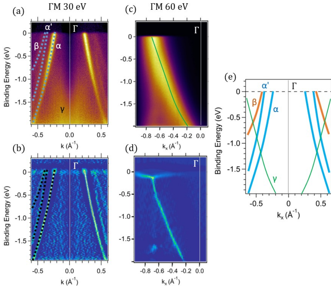
Fig. 3.22 – ARPES 2D cuts along the M - \Gamma - M direction in of Pb/Cu_2Si/Cu(111) . (a) and (b) show the measured spectra with h\nu = 30 eV and its curvature image respectively. The images are centred on \Gamma . Three bands are observed, labelled \alpha , \alpha' and \beta by identification with the band structure before Pb deposition. (c) and (d) show the measured spectra with h\nu = 60 eV and its curvature image respectively. Only one band, \gamma , is observed here. (e) represents schematically all the bands observed.
