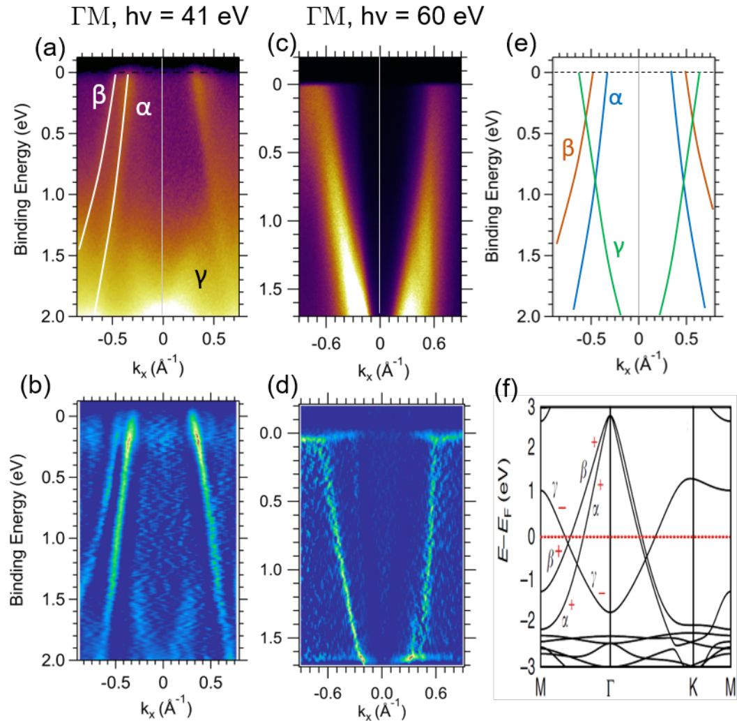
Fig. 3.19 – ARPES on \text{Cu}_2\text{Si}/\text{Cu}(111) , before any Pb deposition, along the \Gamma - M direction with LV-polarized light, centered around \Gamma . (a) and (b) show the spectrum measured with h\nu = 41 eV and its curvature image. Two hole-like bands are identified on the left-hand side of the images, labelled \alpha and \beta . A third band (electron-like) labelled \gamma is faintly distinguishable. It is better seen on (c) where the same region is measured with h\nu = 60 eV, and on (d), which shows the curvature of (c). (e) shows schematically the three bands observed. These are in good agreement with the DFT calculations for the free-standing \text{Cu}_2\text{Si} shown in (f) (from [1])
