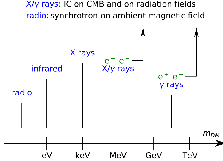
Fig. 2.2. The schematic shows which electromagnetic signal can be produced as a function of the DM particle’s mass.
