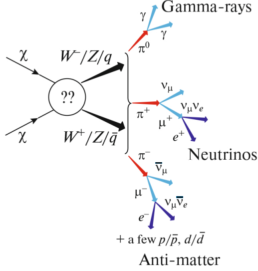
Fig. 2.1. Possible channels of DM annihilation with \gamma rays, neutrinos and charged cosmic rays as final products. Credit: adapted figure from [45].
