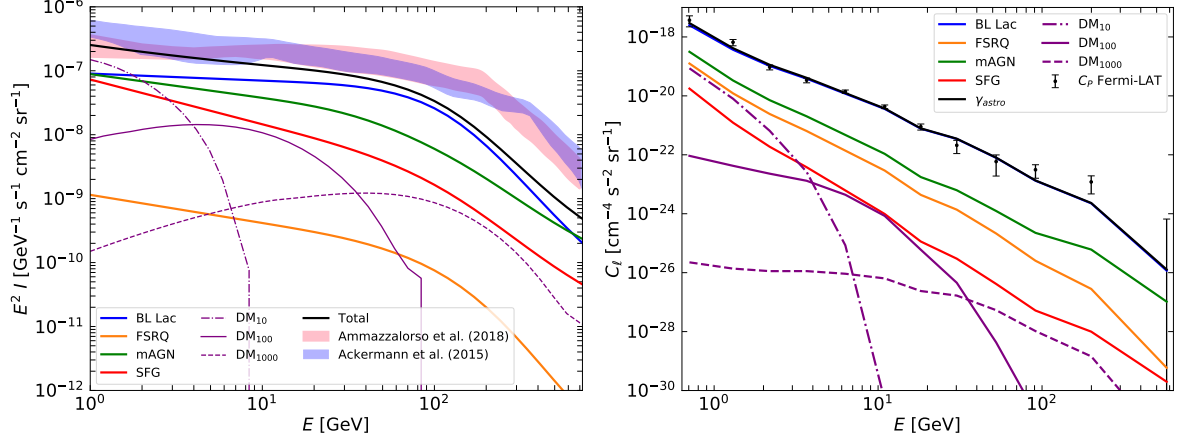
Fig. 5.2. Left: Measured total astrophysical flux (pink [343] and blue [430] shaded bands) together with the theoretical predictions for the contribution from BL Lac (blue), FSRQ (orange), mAGN (green) and SFG (red) as a function of the photon energy. The upper black line denotes the sum of all astrophysical components. The purple dash-dotted, solid and dashed lines show three predictions for a DM signal produced by particles with thermal cross-section and mass m_\chi = 10, 100, 1000 GeV, respectively. Right: Comparison between the theoretical estimation of the total auto-correlation APS of astrophysical origin, C_\ell^{\gamma\gamma} (black), and the latest measurement of the FERMI-LAT detector, C_P [393] (dots with error bars), as a function of the energy bins. The individual contributions from the astrophysical sources and the predictions for annihilating DM are also shown with the same colours and line styles of the left panel.
