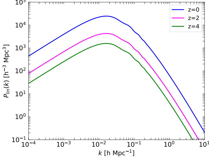
Fig. 3.1. Linear power spectrum as a function of the wavenumber for z = 0 (blue), z = 2 (magenta), z = 4 (green).
