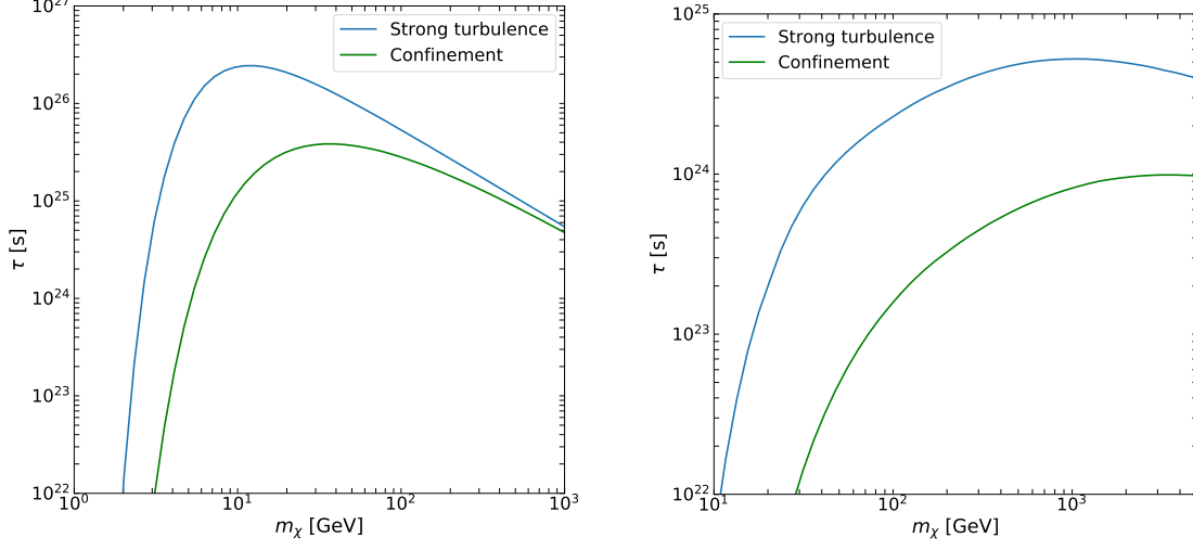
Fig. 8.5. Constraints on DM decay lifetime as a function of the DM mass, for the electron (left) and bottom quark channels (right). The blue line denotes the strong turbulence scenario while the green line refers to the partial confinement regime with k = 5 \cdot 10^4 . The magnetic field is assumed to be B = 100 nG.
