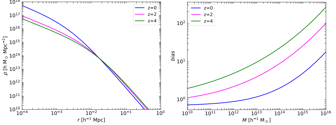
Fig. 3.4. Left: Navarro-Frenk-White density profile for M = 10^{10} M_{\odot} as a function of the distance r from the centre. Right: Halo bias as a function of the halo mass. Different colours denote different values of redshift: z = 0 (blue), z = 2 (magenta), z = 4 (green).
