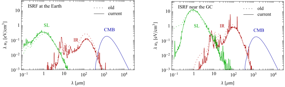
Fig. 7.7. Energy density as a function of the wavelength for the interstellar radiation fields in two locations: at the Earth (left) and near the GC (right). The different colours refer to the different component of the ambient bath: starlight (SL, green), infrared emission (IR, red), CMB (blue). The solid lines refer to more recent measurements, while the dashed curves refer to maps previously used in the literature. We note that the difference in the maps over a few years is not dramatic: it mostly consists of additional detected features, such as the spikes in the optical and infrared light. Credit: [460].
