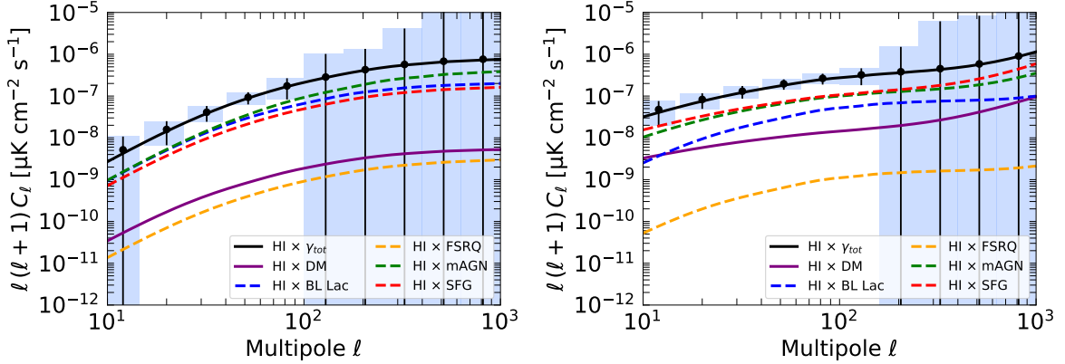
Fig. 5.6. The same as in Fig. 5.5, for the combination SKA1 \times FERMI-LAT. The left panel refers to the higher redshift SKA Band 1, the right panel to the lower redshift SKA Band 2.
