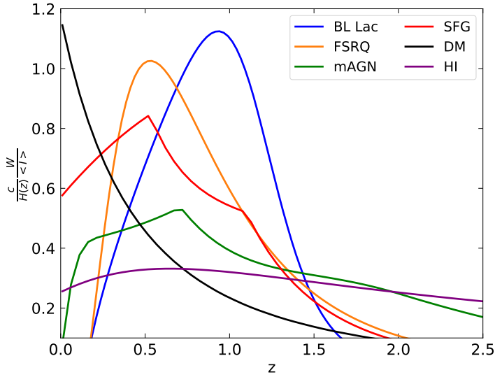
Fig. 5.1. Window functions as a function of redshift for the \gamma -ray emitters considered in our analysis, namely annihilating DM (black), BL Lac (blue), FSRQ (orange), mAGN (green), SFG (red), and HI (purple). The photon energy in the figure is set to E = 5 GeV.
