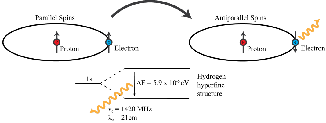
Fig. 4.2. Spin-flip transition of the neutral hydrogen, leading to the emission of a line with wavelength \lambda_e = 21 cm and frequency \nu_e = 1420 MHz.
