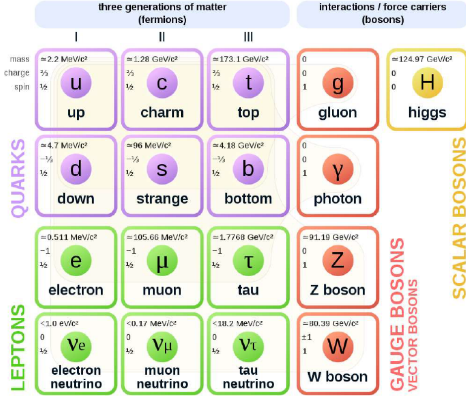
Fig. 1.13. Standard Model of particle physics. Credit: [23].
