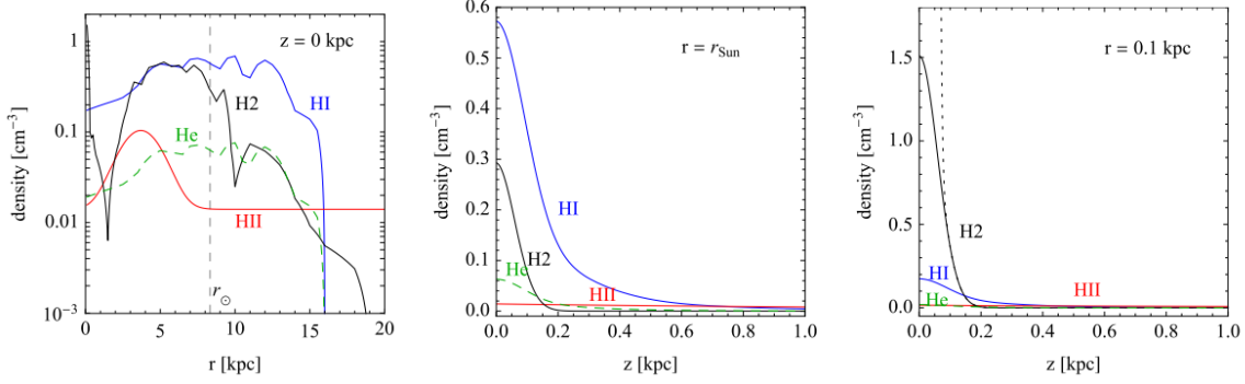
Fig. 7.6. Left: Density of the gas as a function of the distance from the GC. Centre and Right: Density of the gas as a function of the vertical distance from the GP in two different locations: in the position of the Sun (central panel), in a spot near the GC (right panel). Credit: [473].
