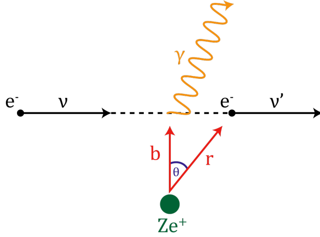
Fig. A.1. In the bremsstrahlung process a charged particle (usually an electron) is decelerated by another charged particle (e.g. an ion with charge Ze^+ ). For the conservation of energy, the outcome of this deceleration is the production of radiation. v and v' indicate the velocity before and after the photon emission. The impact factor b denotes the closest distance between the two particles, while r represents the generic separation and \theta is the angle between these two vectors.
