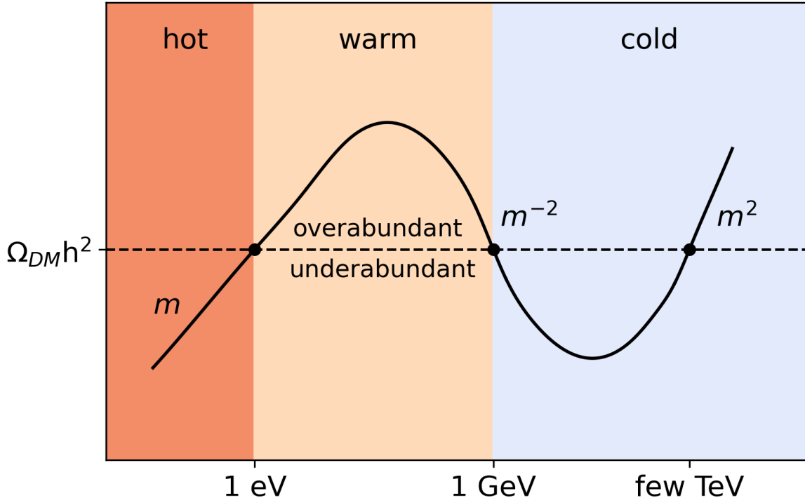
Fig. 1.12. Relic abundance of DM particles as a function of their mass. The red area refers to the hot regime, the orange region to the warm regime, the blue area refers to cold relics. The dashed line represents the DM density parameter, which sets the boundary between overabundance and underabundance species.
