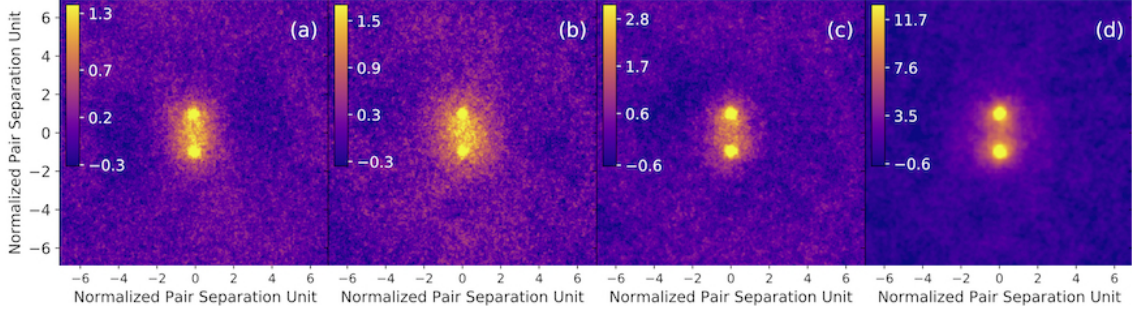
Fig. 8.1. Radio excess measured in nearby pairs of red luminous galaxies. From left to right the columns show the final stack images for: the GLEAM 154 MHz, GLEAM 118 MHz, GLEAM 88 MHz, OVRO-LWA 73 MHz. All the colour bars have units of temperature in K.
