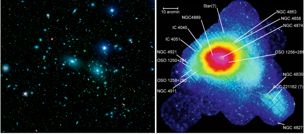
Fig. 1.2. Left: Central region of the Coma Cluster. Credit: Sloan Digital Sky Survey. Right: X-ray image of the Coma Cluster. Credit: XMM-Newton Observatory.
