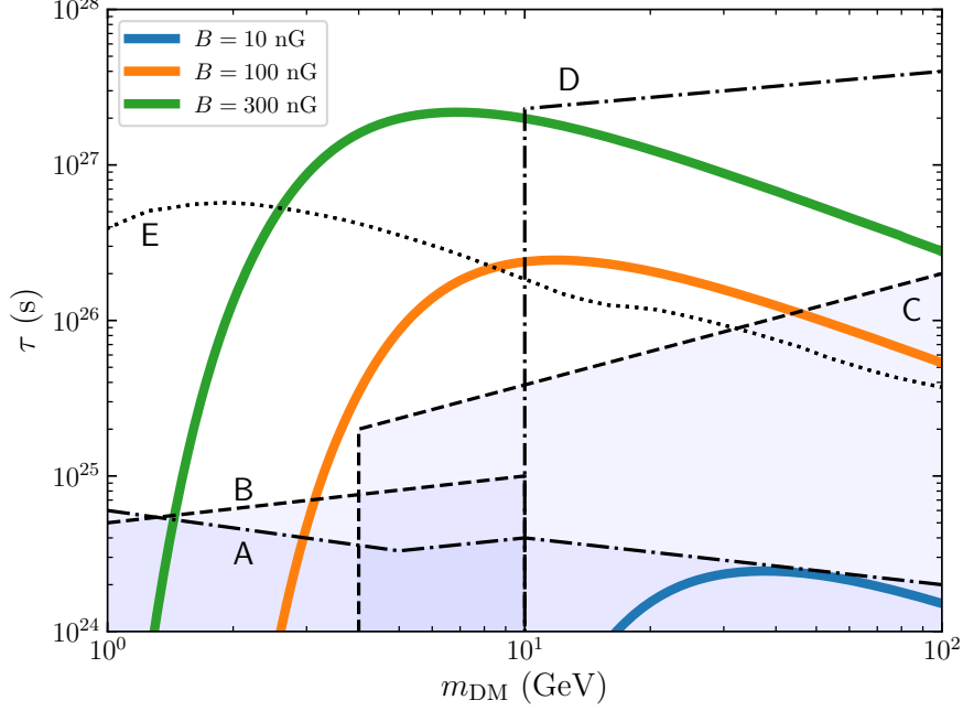
Fig. 8.6. Lower bounds at the 95per cent confidence level on the dark matter lifetime \tau as a function of the dark matter mass m_\chi , for decay into e^+e^- and for some representative values of the magnetic field B . Dashed, dotted and dash-dotted lines show the current bounds from [499] (curve A), [467] (B), [498] (C), [503] (D) and [494] (E).
