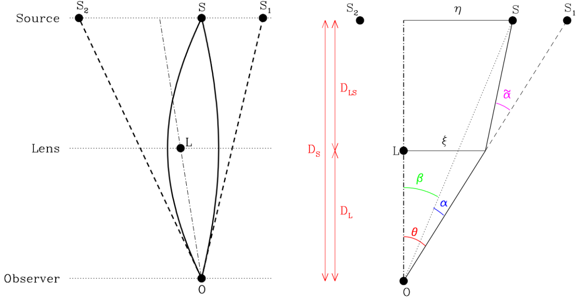
Fig. 1.4. Left: Schematic image of the gravitational lensing in the event that the observer O, the lens L and the background source S are not aligned. This would produce multiple images. Right: This figure includes the relevant angles and distances necessary to derive the lens equation and the Einstein radius. Credit: [12] .
