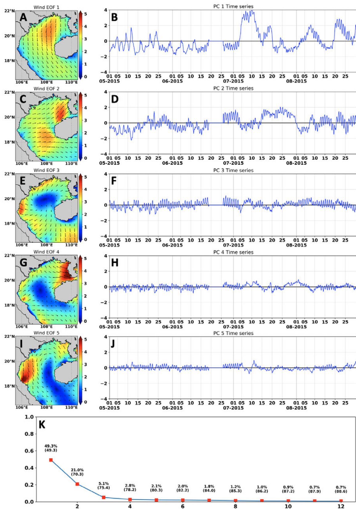
Figure V.2 (A) The spatial component of EOF 1. The colors and arrows present the surface wind velocity and direction, respectively. (B) The temporal component of EOF 1. (C, D), (E, F), (G, H), (I, J): same but for EOF 2, 3, 4, and 5, respectively. (K): Fraction of variability explained by the first 12 EOFs. The upper number is the ratio of the EOF variance to the total variance, while the lower number in the bracket is the cumulative variance.
