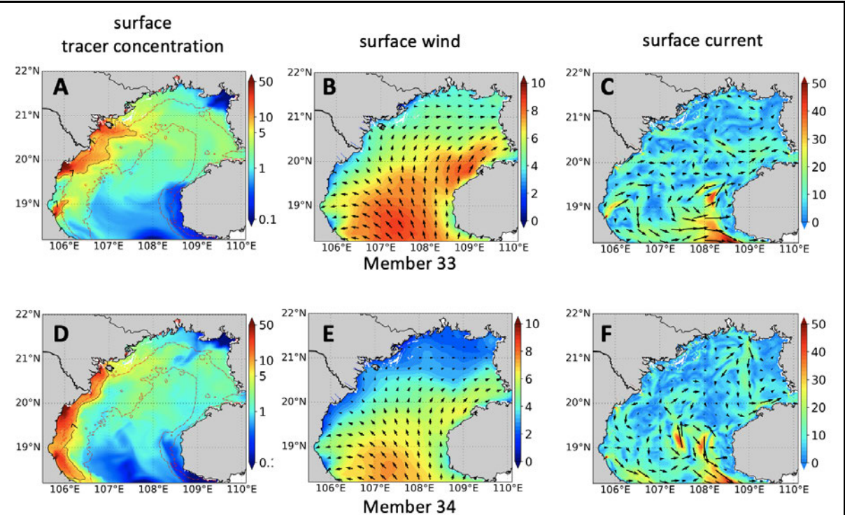
Figure V.17: same as Figure V.16 but computed from 15 - 20 July.
