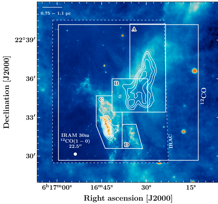
Figure 8.23 Background: Spitzer-MIPS (24.0 \mu\text{m} ) and Spitzer-IRAC (8.0 \mu\text{m} ) maps. White contours: peak brightness temperature map of the 12 CO J=2–1 line observed with the IRAM 30m (see also Fig. 6.10). The white boxes represent the area where the spectra corresponding to each structure (A, B, C, D) are extracted. The beam diameter of the IRAM 30m observations of 12 CO J=1–0 is shown in the bottom-left corner. The 10' \times 10' field of observations is indicated by a solid white box (indicated by the label ' 12 CO'), and the IRAC field of observation is indicated by a dashed white box (indicated by the label 'IRAC').
