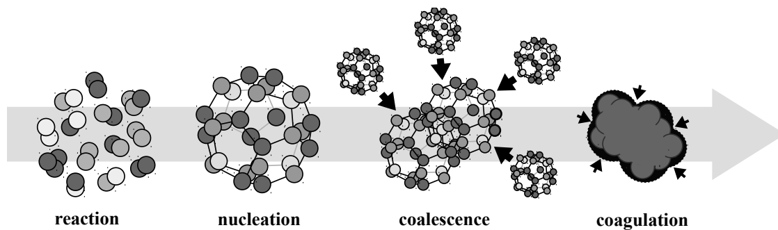
Figure 1.12 Schematic representation of the nucleation (reaction, nucleation) and condensation (coalescence, coagulation) chemical phases leading to the synthesis of molecules, precursor clusters and dust grains in the ejecta of young SNRs. For the sake of simplicity, only C_{28} clusters are represented, but many other clusters participate in the synthesis (Sarangi et al. , 2018).
