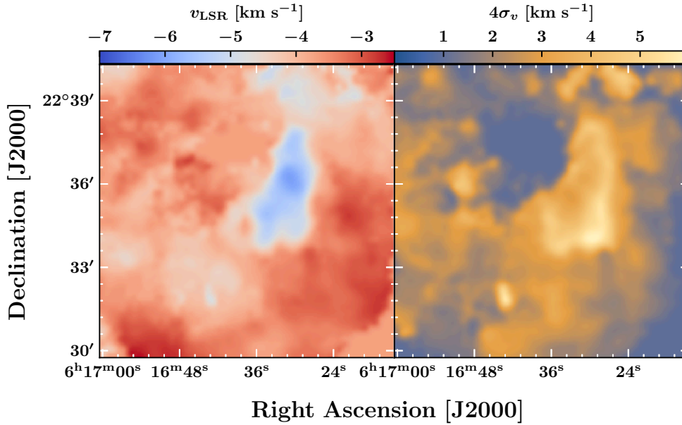
Figure 6.17 ‘Standard’ moment maps (see text). Left : first moment map of the IRAM 30m ^{13}\text{CO} J=1–0 data cube. Right : second moment map. The colorbar of the 1 st moment map is centered on the velocity of IC443 in the local standard of rest, v_{\text{LSR}} = -4.5 \text{ km s}^{-1} .
