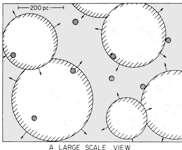
Figure 1.7 Large-scale structure of the interstellar medium ( McKee and Ostriker, 1977 ). The scale here is 20 times greater than in Fig. 1.6: the region is 600 \text{ pc} \times 800 \text{ pc} . Only clouds with a radius greater than 7 pc are shown (hatched circles). Evolved SNRs of size greater than 180 pc are represented by large expanding circles. Altogether about 9000 clouds, most with a radius \sim 2.1 \text{ pc} , would occur in a region this size.
