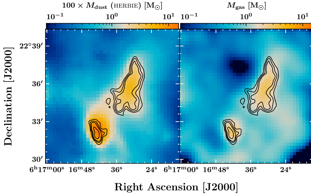
Figure 9.25 Comparison between the HerBIE dust mass (multiplied by the gas-to-dust ratio GDR = 100 , Hildebrand 1983) and ^{12}\text{CO} -inferred molecular gas mass maps in the 10' \times 10' shared field of observations (see Chapter 8). Black contours represent the IRAM 30m ^{12}\text{CO} J=2–1 peak map shown in Fig. 6.10 (contour levels: 0.25, 0.35, 0.45 and 0.75 times the maximum value across the map).
