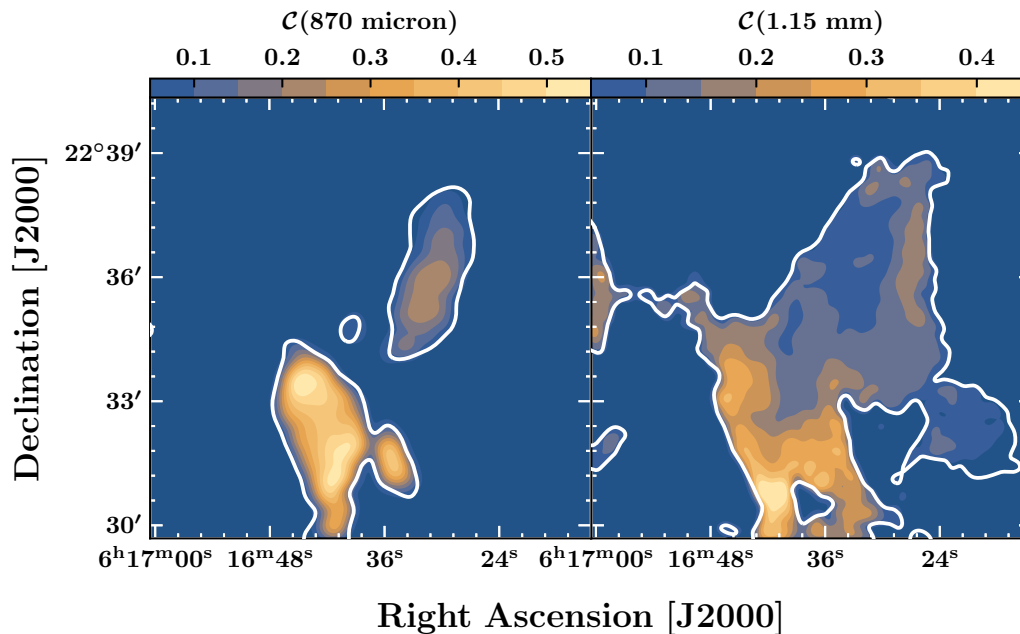
Figure 9.5 LABOCA (870 \mu\text{m} , left panel) and NIKA2 (1.15 mm, right panel) contamination maps. The quantity shown by filled contours is the pixel value of the proportion F_{\nu}^{\text{line}}/F_{\nu}^{\text{BB}} , where F_{\nu}^{\text{line}} is the ^{12}\text{CO} J=3–2 (for LABOCA) or J=2–1 (for NIKA2) line flux measured by the broadband instrument (see Eq. 9.5) and F_{\nu}^{\text{BB}} is the flux measured in the continuum map. White contours show the area where F_{\nu}^{\text{BB}} \geq 3\sigma , where \sigma is the noise.
