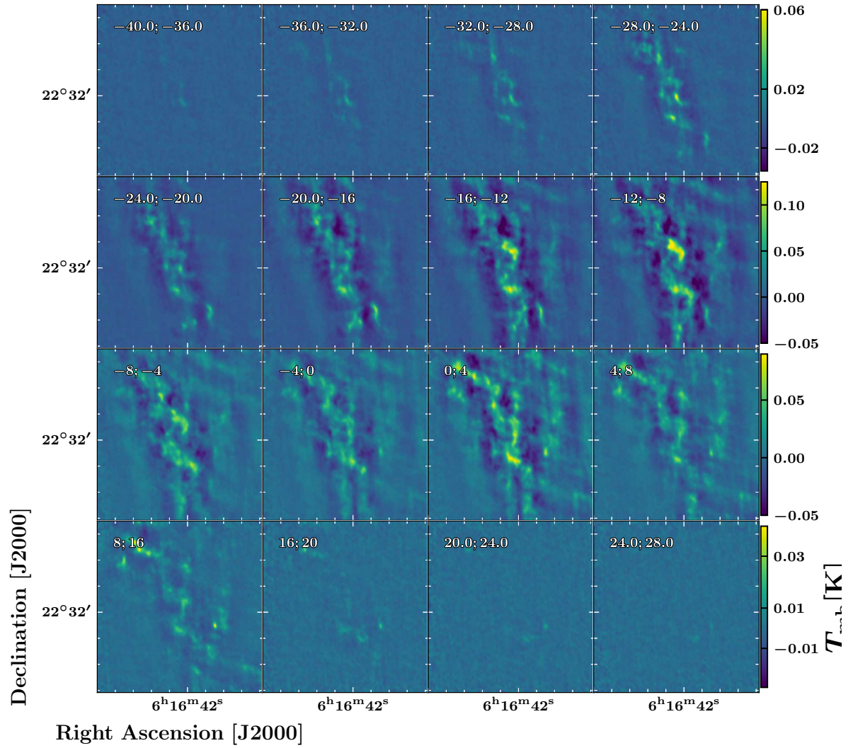
Figure D.2 Channel map of our \text{HCO}^+ PPV cube obtained with NOEMA observations. Each panel represents the velocity-integrated emission in the same area, between -40 \text{ km s}^{-1} and 28 \text{ km s}^{-1} . The boundaries of the velocity intervals (in \text{km s}^{-1} ) are indicated on the top left corner of each panel.
