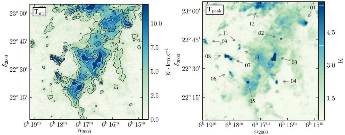
Figure 2.8 Left panel: ^{12}\text{CO} integrated temperature map in velocity range of -10 to 0 \text{ km s}^{-1} , mostly tracing the ambient gas (Lee et al. , 2012). Right panel: ^{12}\text{CO} peak temperature map over the same velocity interval. The numbers denote the labels and location of small molecular clumps identified by the authors.
