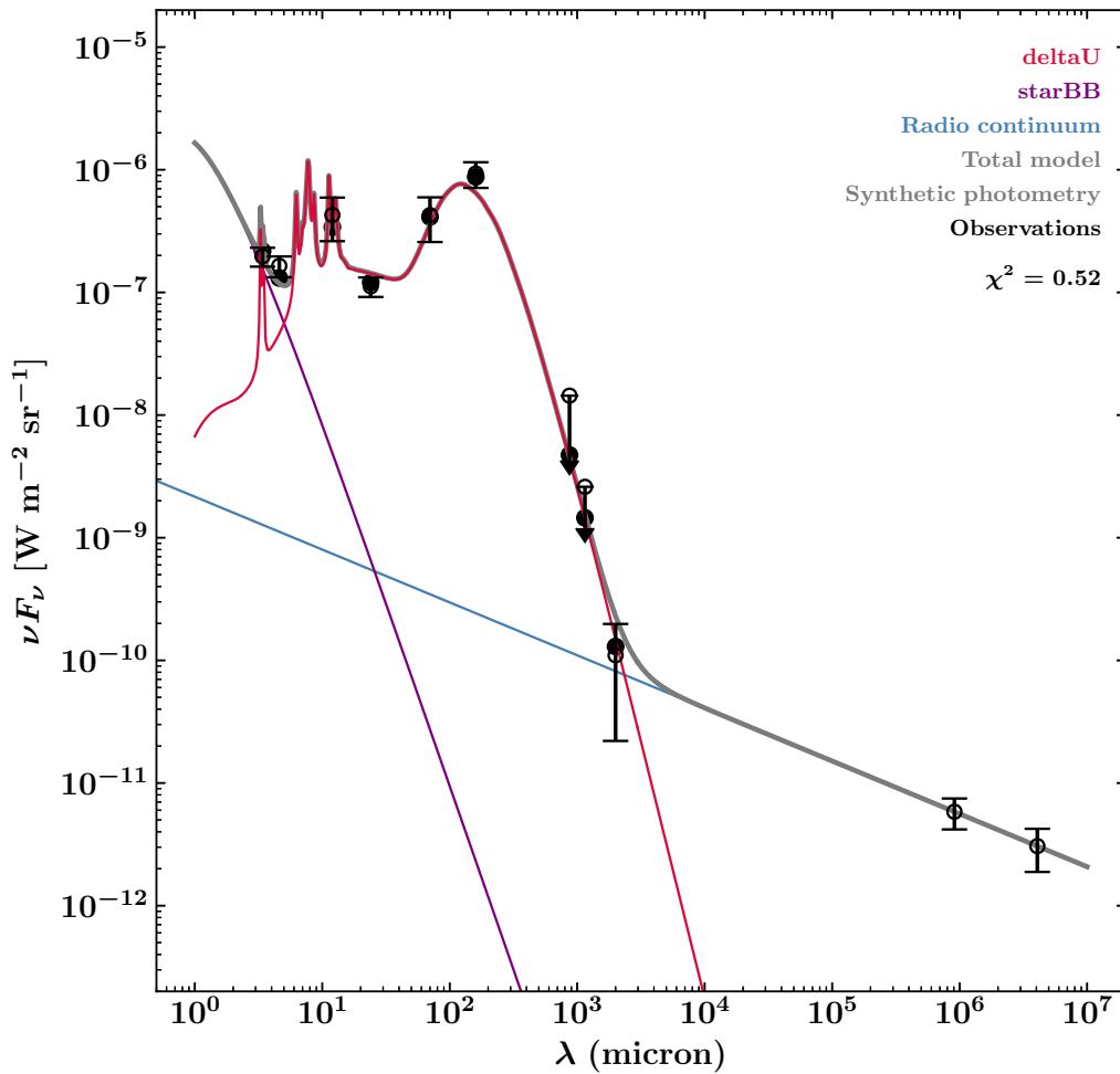
Figure 9.13 Average spectral energy distribution in the extended G region. Observations are shown in black, with \pm 1\sigma errorbars. The HerBIE models of the illuminated dust mixture \delta U , stellar continuum \text{starBB} and the power-law model of the radio continuum are shown respectively by red, purple and blue curves. The total model and synthetic photometric data points are shown in gray.
