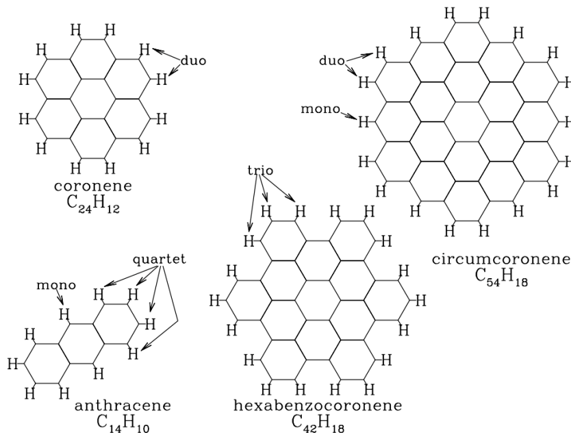
Figure 5.2 Structure of four PAHs. Examples of singlet, doublet, trio and quartet H atoms are indicated. Figure reproduced from Draine (2011) .
