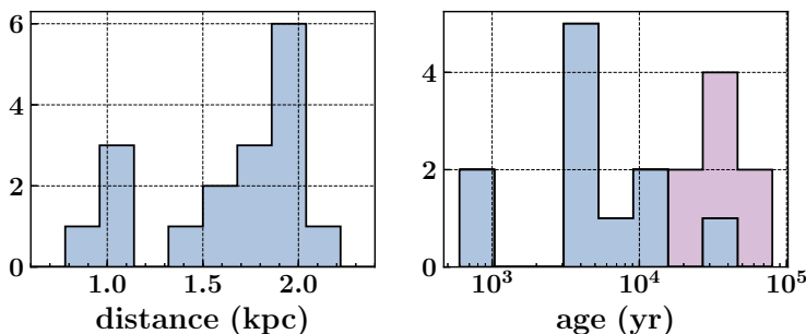
Figure 2.1 Distance ( left ) and age ( right ) measurements for the supernova remnant IC443. On the right panel, two colors are used to distinguish estimates from X-ray studies (in blue) from other methods of measurements (in pink).
