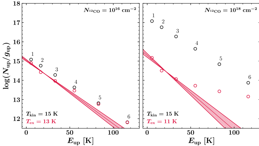
Figure 4.3 Synthetic population diagrams produced with RADEX using distinct total ^{12}\text{CO} column densities in the input. Left: N_{12\text{CO}} = 10^{16} \text{ cm}^{-2} . Right: N_{12\text{CO}} = 10^{18} \text{ cm}^{-2} . The other parameters remain fixed: T_{\text{kin}} = 15 \text{ K} , \Delta v = 1 \text{ km s}^{-1} , T_{\text{bg}} = 2.7 \text{ K} , n_{\text{H}_2} = 10^6 \text{ cm}^{-3} . The black data points correspond to the exact values of the upper level populations for J_u = 1 - 6 , whereas the red data points correspond to the upper level populations inferred from the modelled intensities of the transitions ( via Eq. 4.30, i.e. not corrected for line opacity). We indicate the excitation temperature inferred from a linear fit of the level populations J_u = 1 - 3 .
