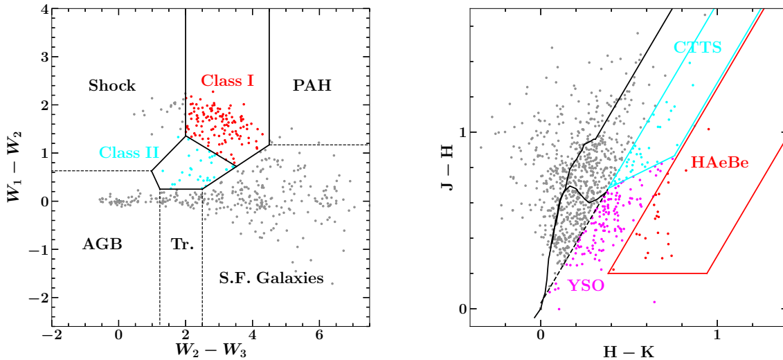
Figure 10.1 Left : WISE census of YSO candidates in our 16' \times 16' field of observations in the IC443 SNR. Cyan dots are Class II candidates, red dots are Class I candidates and gray dots are point sources detected by WISE and rejected by our color-color filtering based on photometric bands W_1 , W_2 and W_3 . Right : 2MASS census of YSO candidates in the same region. Cyan dots are CTTS candidates, red dots are HAeBe candidates, magenta dots are YSO candidates and gray dots are point sources detected by 2MASS and rejected by our JHK color-color filtering.
