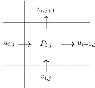
Figure 4.2: Staggered grid for fluid computation, representing a pressure centered computational cell. Here i & j are positive integers referring to the cell position. P_{i,j} represents the pressure and is estimated at the center of the cell i,j . The x -axis velocity, u is computed on the left and right cell's wall. Same for v the y -axis on the top and bottom.
