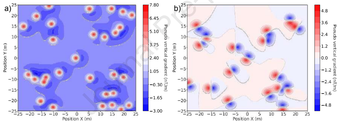
Figure 5: Induced magnetic anomaly maps included in our synthetic data set used for training. The dipole type anomalies correspond to variable declination values and an inclination of 30^\circ (a) and 0^\circ (b).
