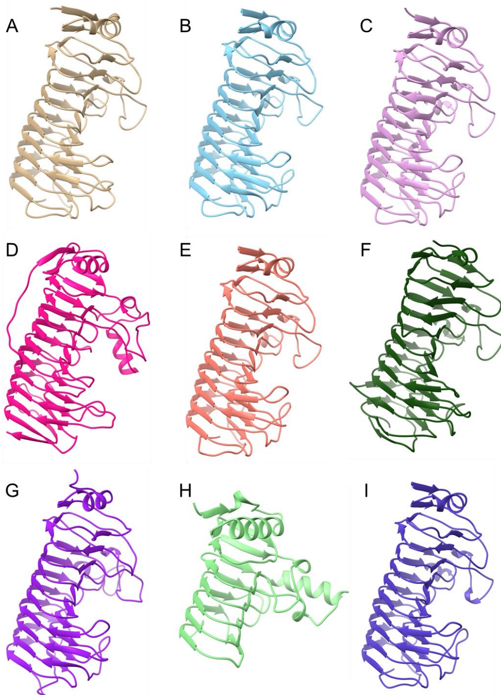
Figure 12. Endo-PG structures published in PDB
