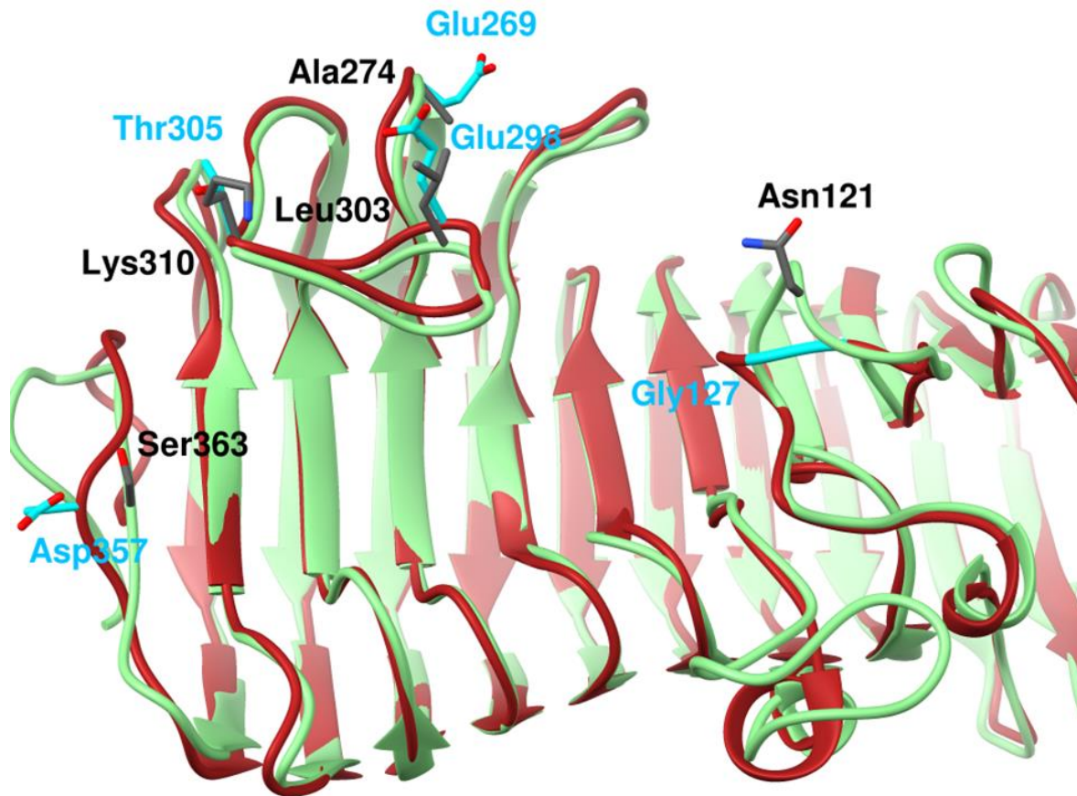
Figure S11. Structural determinants for the non-competitive inhibition of AnPG1 by PvPGIP AnPG1 structure (red with cyan-labelled AA) was superimposed to the structure of GfPG1 (green with black-labelled AA). The amino-acids (Asn121, Ala274, Leu303, Lys310 and Ser363) known to be of importance for the interaction between GfPG1 and PvPGIP2 (not shown here) are absent in AnPG1.
