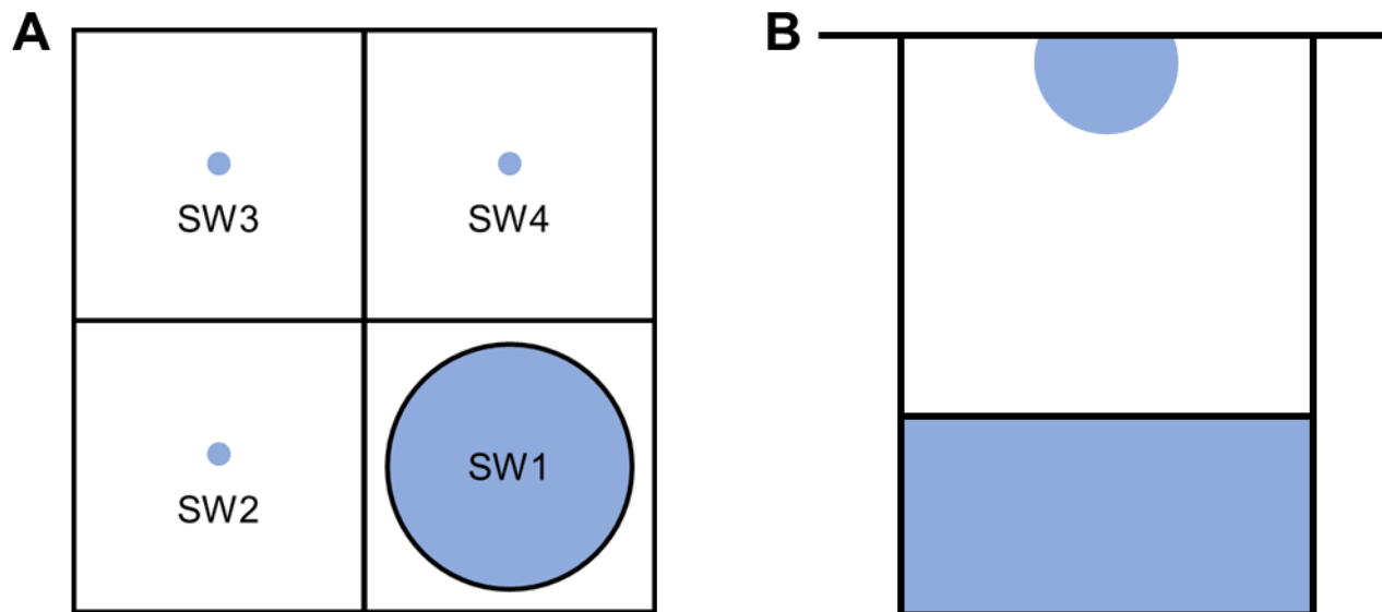
Figure 40. Schematic representation sitting and hanging drop vapour diffusion methods A) Sitting drop, 96 wells plate in each well containing 4 SW (SubWells). In the SW1 is filled with 50 \mu\text{L} of precipitation solution while the three different protein concentrations in SW2, SW3, and SW4 are 20 \text{mg ml}^{-1} , 10 \text{mg ml}^{-1} and 5 \text{mg ml}^{-1} , respectively B) Scale up well is filled with 200 \mu\text{L} of precipitation solution while 1 \mu\text{L} of the precipitant condition with 1 \mu\text{L} of protein is mixed in hanging drop vapour diffusion method.
