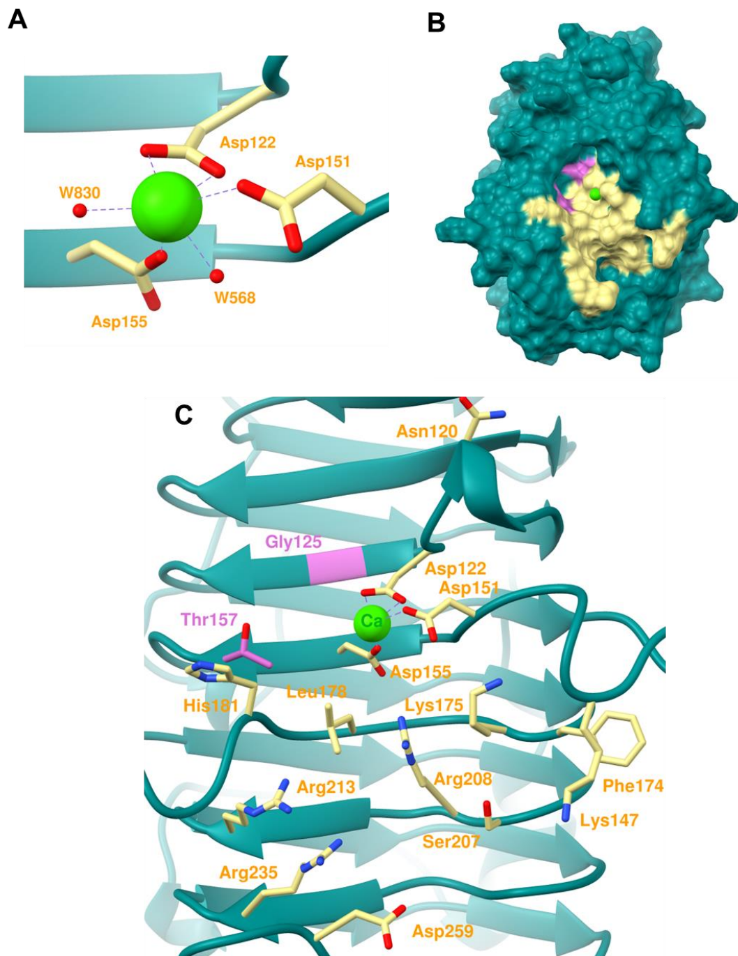
Figure 37. Structure determination of VdPelB
