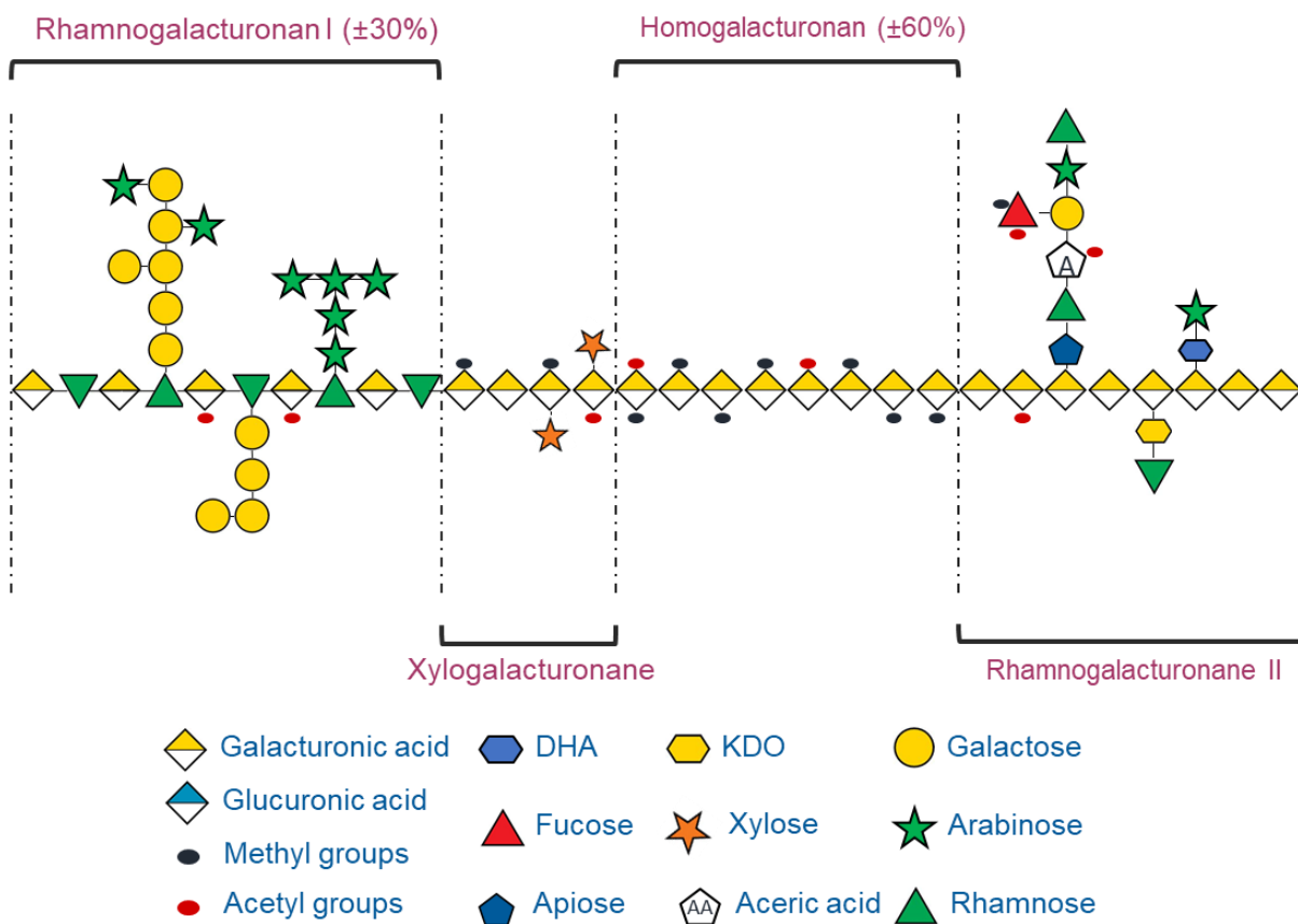
Figure 5. Schematic structure of pectic polysaccharides
