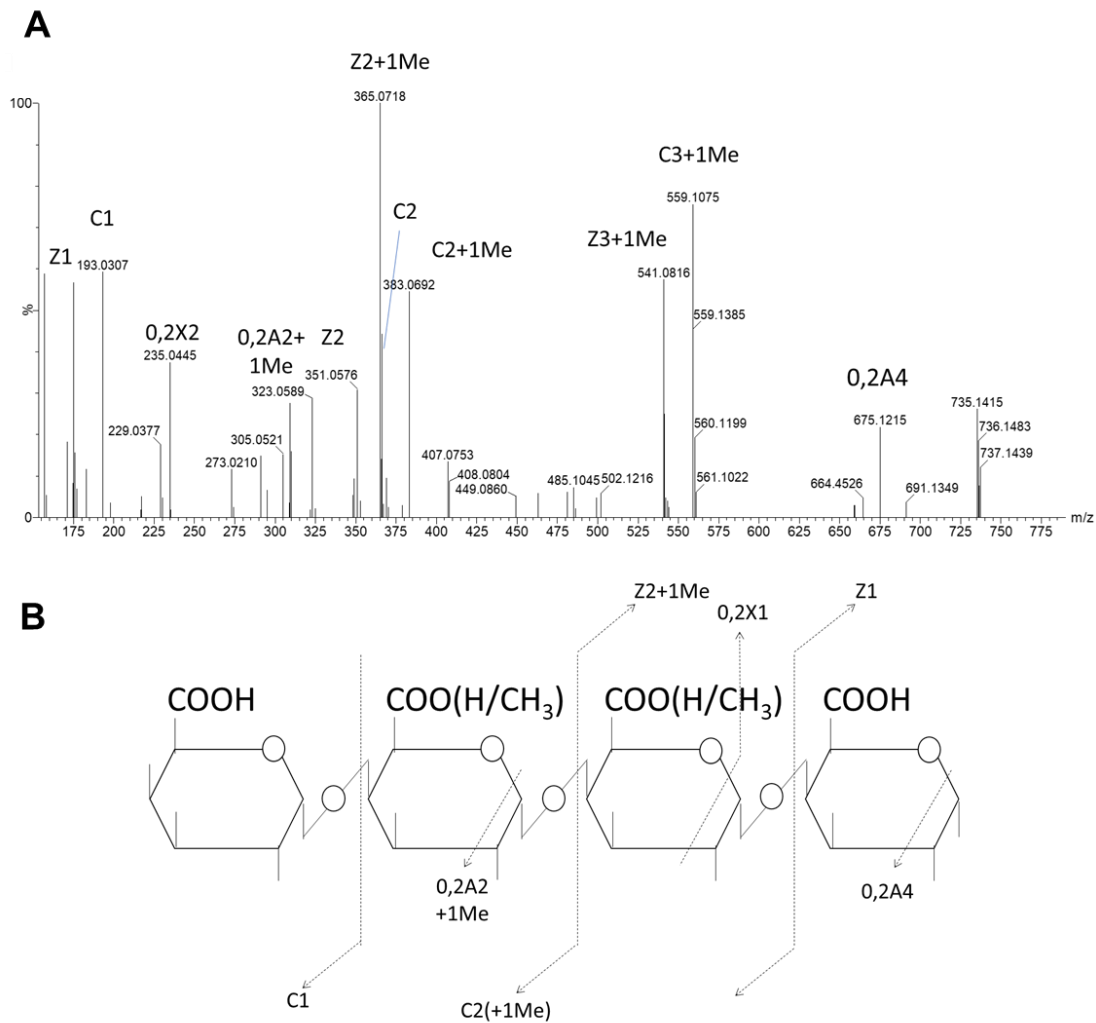
Figure S22. Example of MS 2 fragmentation pattern of GalA 4 Me 1 MS 2 fragmentation pattern of GalA 4 Me 1 oligomer (m/z 735,1472907) produced by VdPelB from pectin DM >85%. Subscript numbers indicate the degree of polymerization
