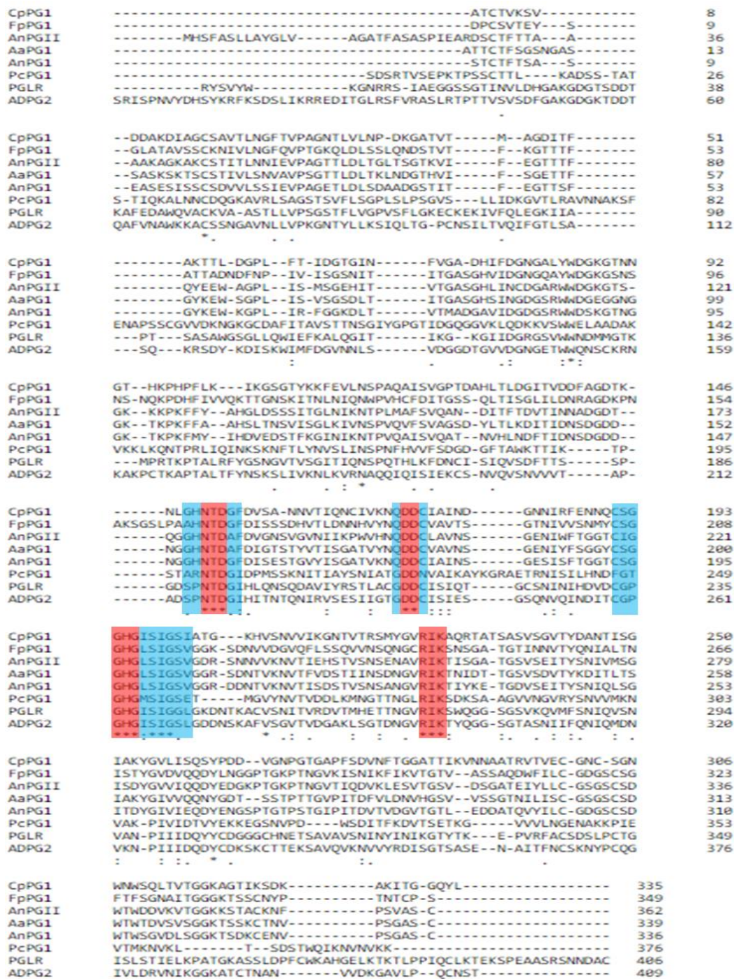
Figure S9. Sequence alignment of PGLR and ADPG2 with characterized and crystallized fungal PGs
