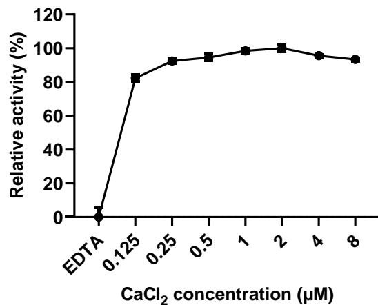
Figure S20. Effects on increasing concentrations of Ca 2+ on VdPelB activity Pectins DM>85% were digested using VdPelB for 12 min at 40°C and pH 7 with increasing concentrations of Ca 2+ or Ca 2+ and EDTA.
