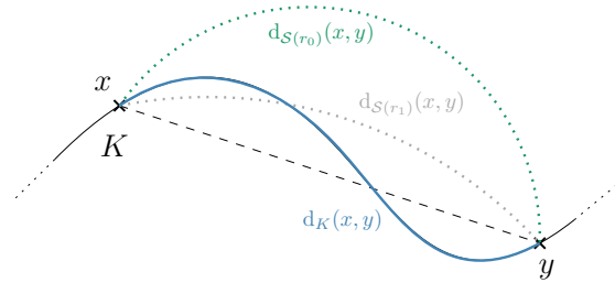
Figure 3.1 – A curve K in the plane. In blue is the shortest path between two points x and y , whose length is d_K(x, y) . In green (resp. grey) is the circle portion of radius r_0 (resp. r_1 ) going through x and y . The layout is chosen so that r_0 \leq r_1 and d_{S(r_1)}(x, y) \leq d_K(x, y) \leq d_{S(r_0)}(x, y) .
