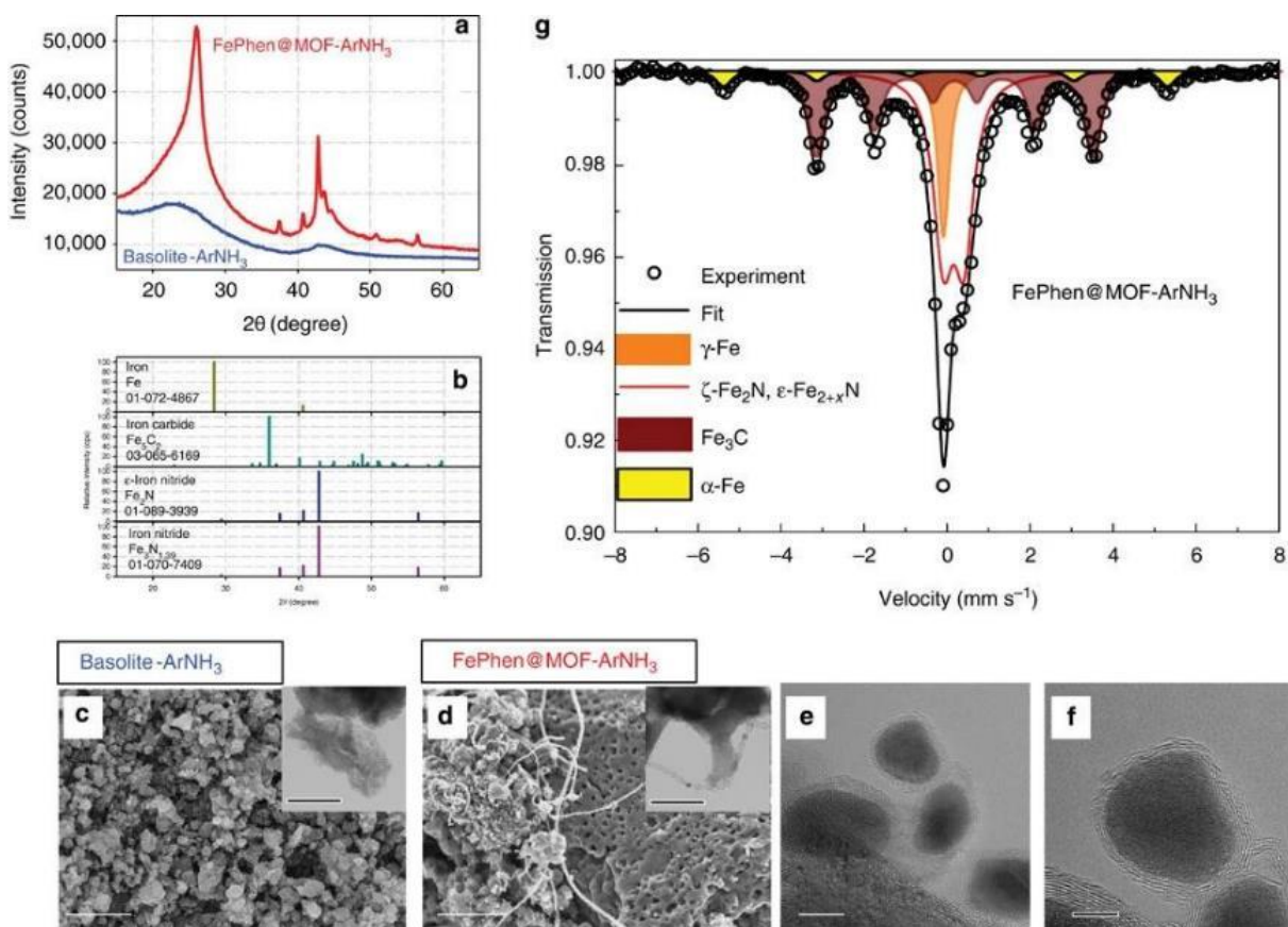
Figure 11. (a) X-ray diffraction pattern of FePhen@MOF-ArNH 3 and Basolite-ArNH 3 . (b) Diffraction patterns of iron, iron carbide and iron nitrides. (c) SEM image of Basolite-ArNH 3 . Scale bar, 2 \mu m. Inset TEM image of amorphous carbon. Scale bar, 100 nm. (d) SEM image of FePhen@MOF-ArNH 3 . Scale bar, 2 \mu m. Inset TEM image of bamboo-jointed CNT. Scale bar, 100 nm. (e) HR-TEM image of iron encapsulated in bamboo joints of CNT in FePhen@MOF-ArNH 3 . Scale bar, 10 nm. (f) HR-TEM image of Fe/Fe x C nanoparticle surrounded by graphite layers. Scale bar, 5 nm. (g) 57 Fe Mössbauer spectrum of FePhen@MOF-ArNH 3 measured at room temperature. Reproduced from Ref. [109]
