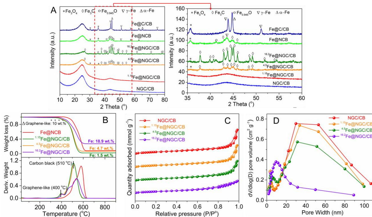
Figure 4. (A) The XRD profiles of all as-prepared catalysts; (B) The TGA (above) and DTG (below) curves of ^{1.15}\text{Fe@NGC/CB} , ^{4.5}\text{Fe@NGC/CB} , ^{16.2}\text{Fe@NGC/CB} , and \text{Fe/NCB} ; (C) \text{N}_2 adsorption-desorption isotherm plots of samples with variable Fe addition recorded at 77 K along with (D) the respective pore size distributions (BJH method) based on desorption branch.
