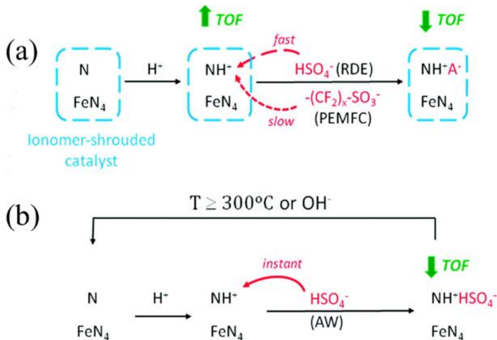
Figure 9. Change of the chemical state of protonable N-groups and simultaneous change of the turnover frequency (TOF) for the ORR of \text{FeN}_4 catalytic sites when the \text{Fe}/\text{N}/\text{C} catalyst is shrouded by proton-conducting ionomer (a) or directly in contact with an aqueous acidic solution (b). In case (b), the acid-washed catalyst can be reactivated either thermally or chemically. Reproduced from Ref. [106]
