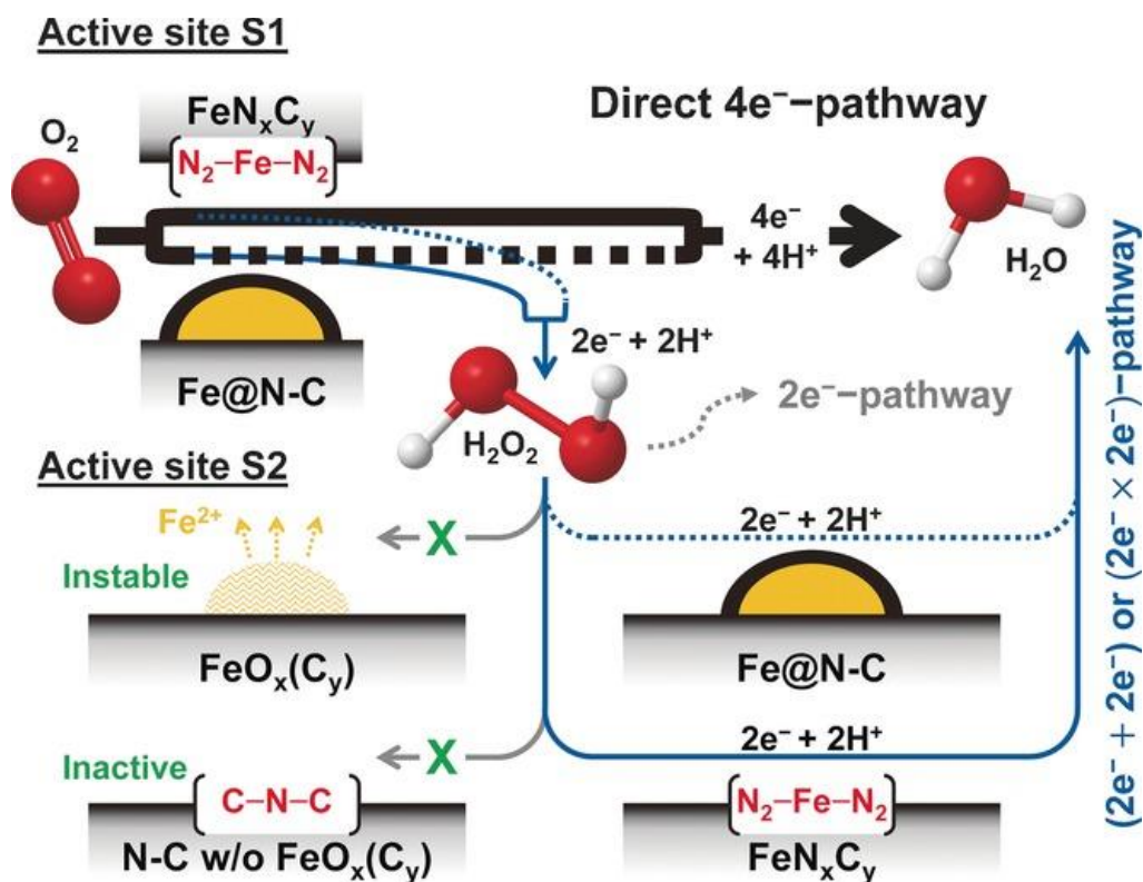
Figure 8. ORR mechanisms on Fe-N-C catalyst in acid medium. The site S1 is \text{FeN}_x\text{C}_y moieties or Fe@N-C. \text{FeN}_x\text{C}_y mostly catalyzes direct 4e^- ORR, along with a minor fraction of \text{H}_2\text{O}_2 . Fe@N-C produces higher fraction of \text{H}_2\text{O}_2 in comparison to \text{FeN}_x\text{C}_y . The released \text{H}_2\text{O}_2 is then reduced to \text{H}_2\text{O} on site S2, either \text{FeN}_x\text{N}_y or Fe@N-C. Surface-exposed Fe particles and N groups without subsurface Fe are PRR inactive. Reproduced from Ref. [99]
