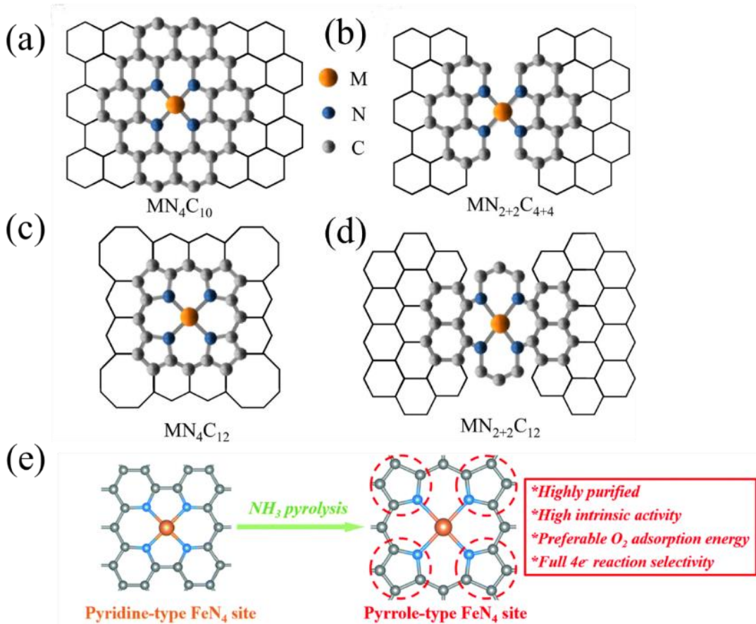
Figure 13. Proposed active site structures for Fe-centered moieties. (a) Pyridinic in-plane \text{FeN}_4\text{C}_{10} moiety, (b) pyridinic armchair edge \text{FeN}_{2+2}\text{C}_{4+4} moiety, (c) porphyrinic in-plane \text{FeN}_4\text{C}_{12} moiety, (d) porphyrin zig-zag edge \text{FeN}_{2+2}\text{C}_{12} moiety, (e) schematic illustration of preparation of high-purity pyrrolic-type \text{FeN}_4 site. Reproduced from Ref. [178, 179]
