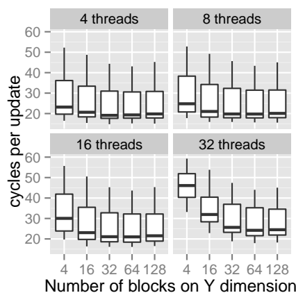
Figure 4.11: Performance of different Y blocking configurations. For a high number of threads, reducing the Y block size improves performance.
