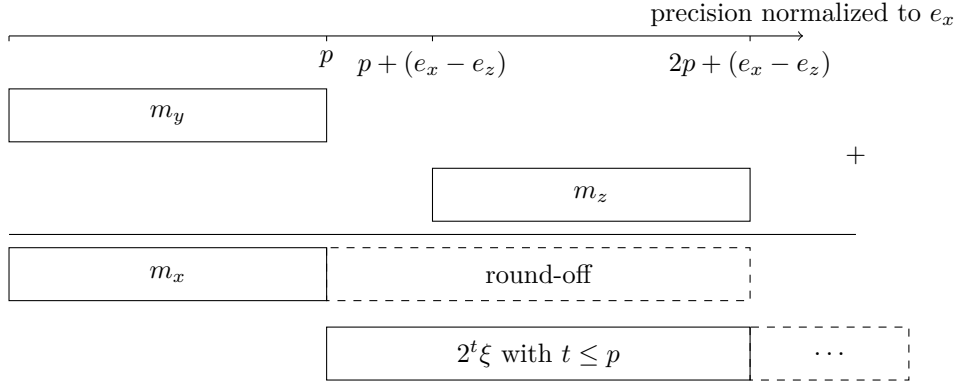
Figure 6.5: MCA computation \text{inexact}(x) = \text{inexact}(y + z) with e_x = e_y .
