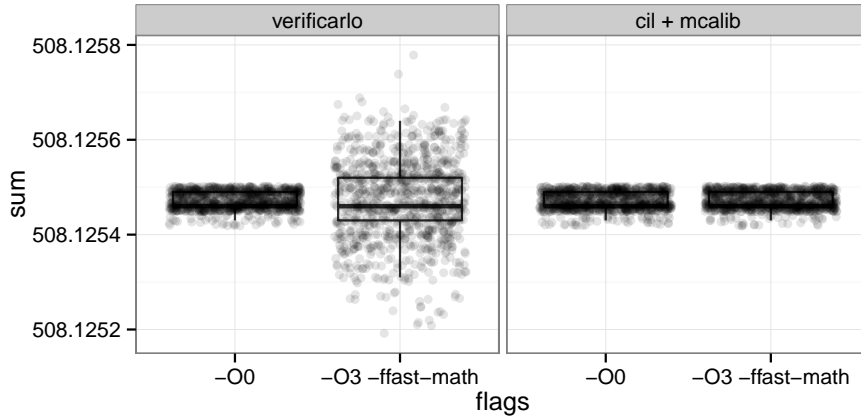
Figure 6.4: One thousand MCA RR samples of Kahan summation: CIL+MCALIB is unable to capture the compiler effect on Kahan’s summation because it operates at the source level. On the other hand verifcarlo operates after compiler optimizations and correctly shows that the -O0 version is more precise than the -O3 -ffast-math version thanks to the compensation term c.
