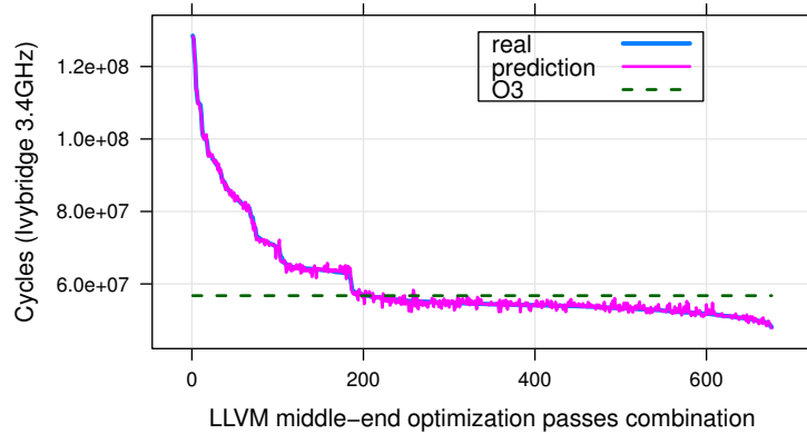
Figure 4.2: NAS SP ysolve region execution time across 1000 schedules of random compiler combinations passes based on O3 . Compilation sequences are sorted according to their original execution time. We remove compilation sequences that produce the same binary. real and predicted respectively represents the original execution time and the codelet prediction based on representative invocations replay. The codelet faithfully predicts the region execution time across the different compiler optimizations.
