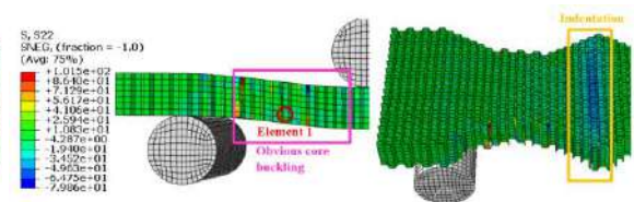
(III) Normal stress S22.
