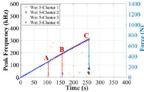
(c) 120% MC specimen Wet 5.
