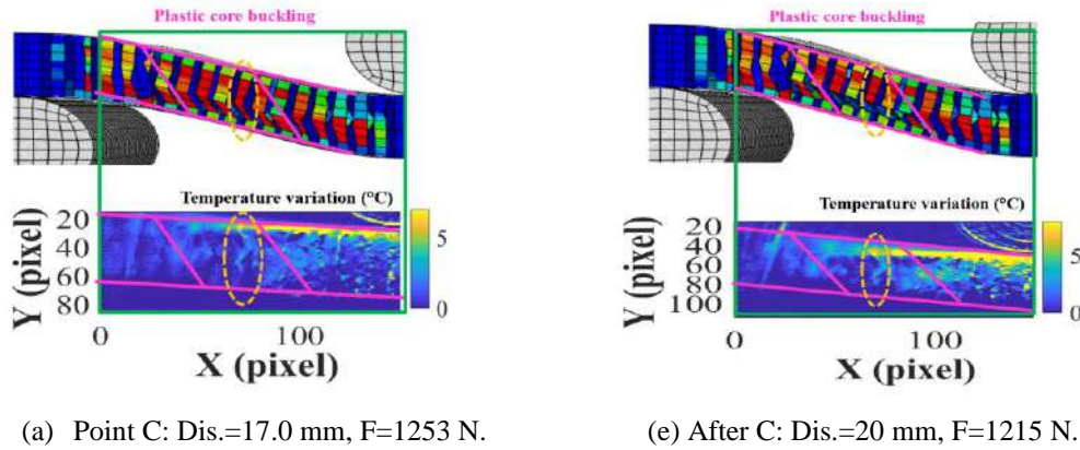
Fig. 4-20. Damage evolution prediction of wet sandwich by Abaqus simulation model Wet HS3.
