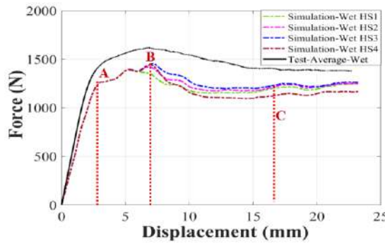
(c) Different groups of wet sandwich (6.5% MC).
