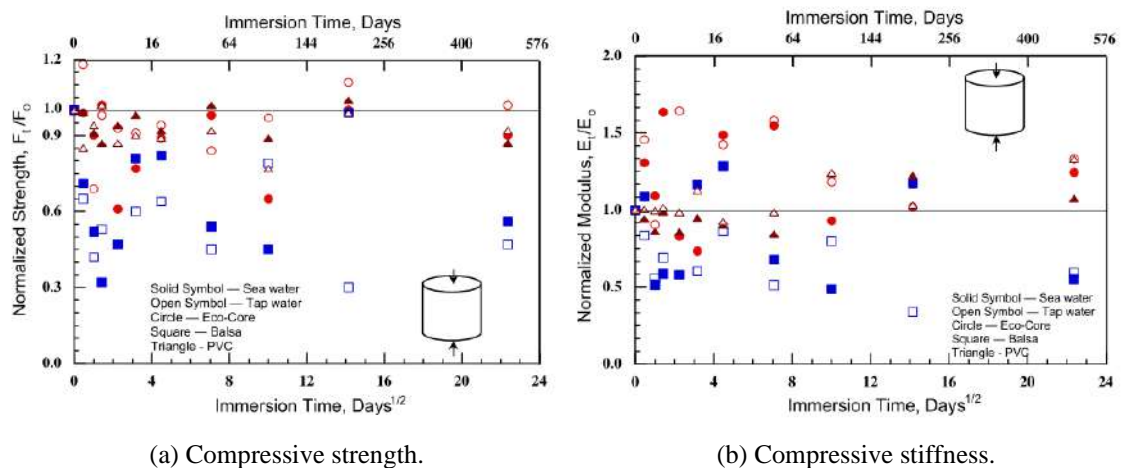
Fig. 1-18. Normalized compressive property change after immersion in sea and tap water [55].
