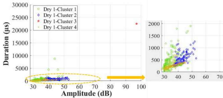
(a) Specimen Dry 1.
