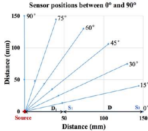
Fig. 2-10. Positions of sensors and source on the tested panel between 0° and 90°.
