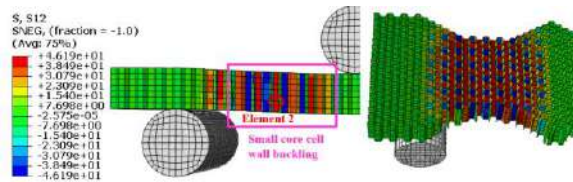
(I) Shear stress S12.
