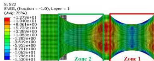
(II) Normal stress S22.
