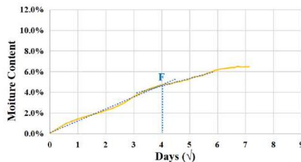
(c) Moisture Content (MC) increase vs. square root of immersion days.
