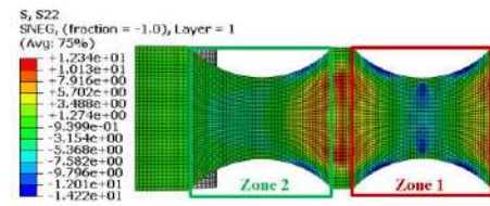
(II) Normal stress S22.
