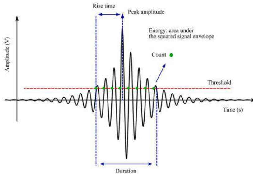
Fig. 1-23. Characteristics of one hit of acoustic emission wave [104].
