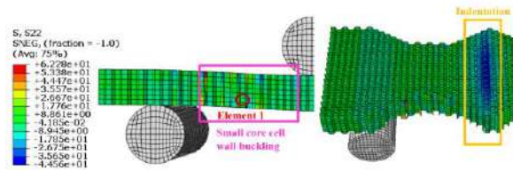
(III) Normal stress S22.
