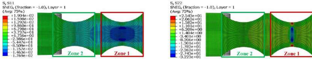
(I) Normal stress S11.
