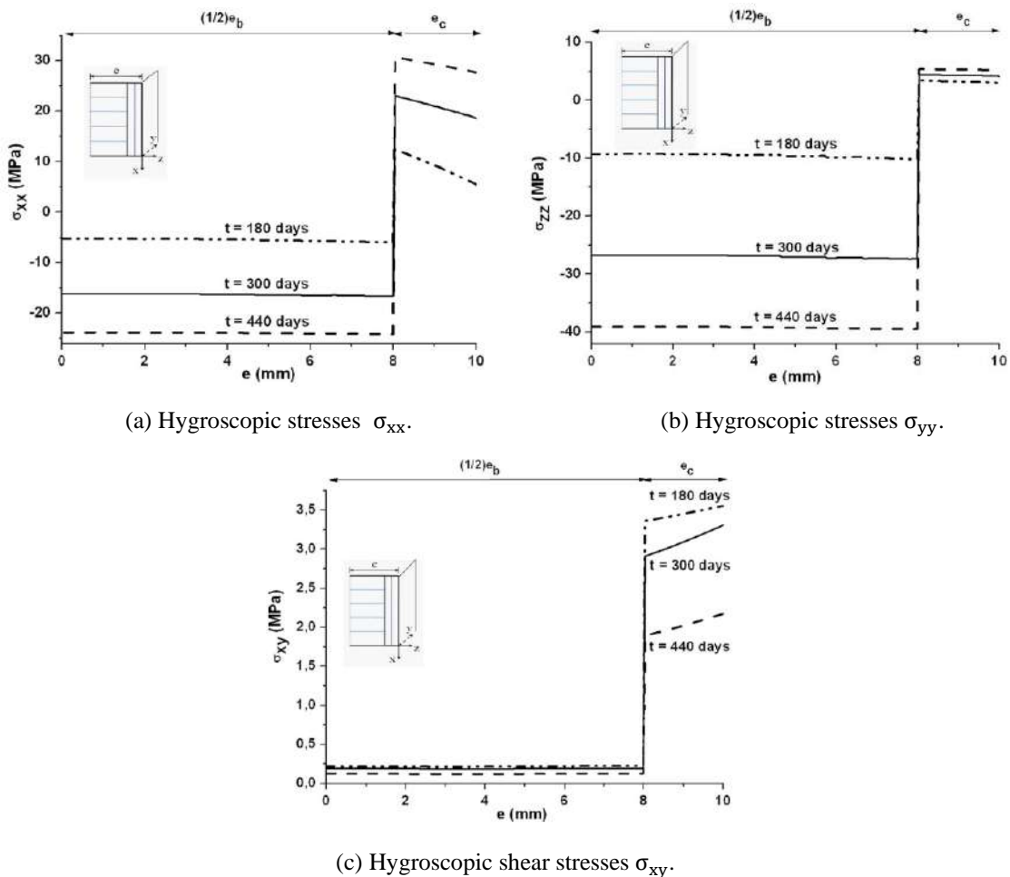
Fig. 1-20. Variation of hygroscopic stresses through the thickness of the sandwich plate [36].
