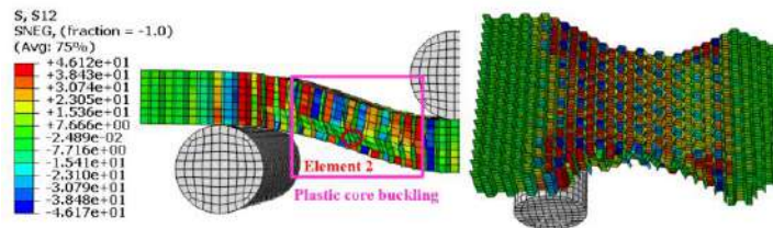
(I) Shear stress S12.
