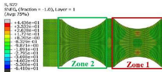
(II) Normal stress S22.
