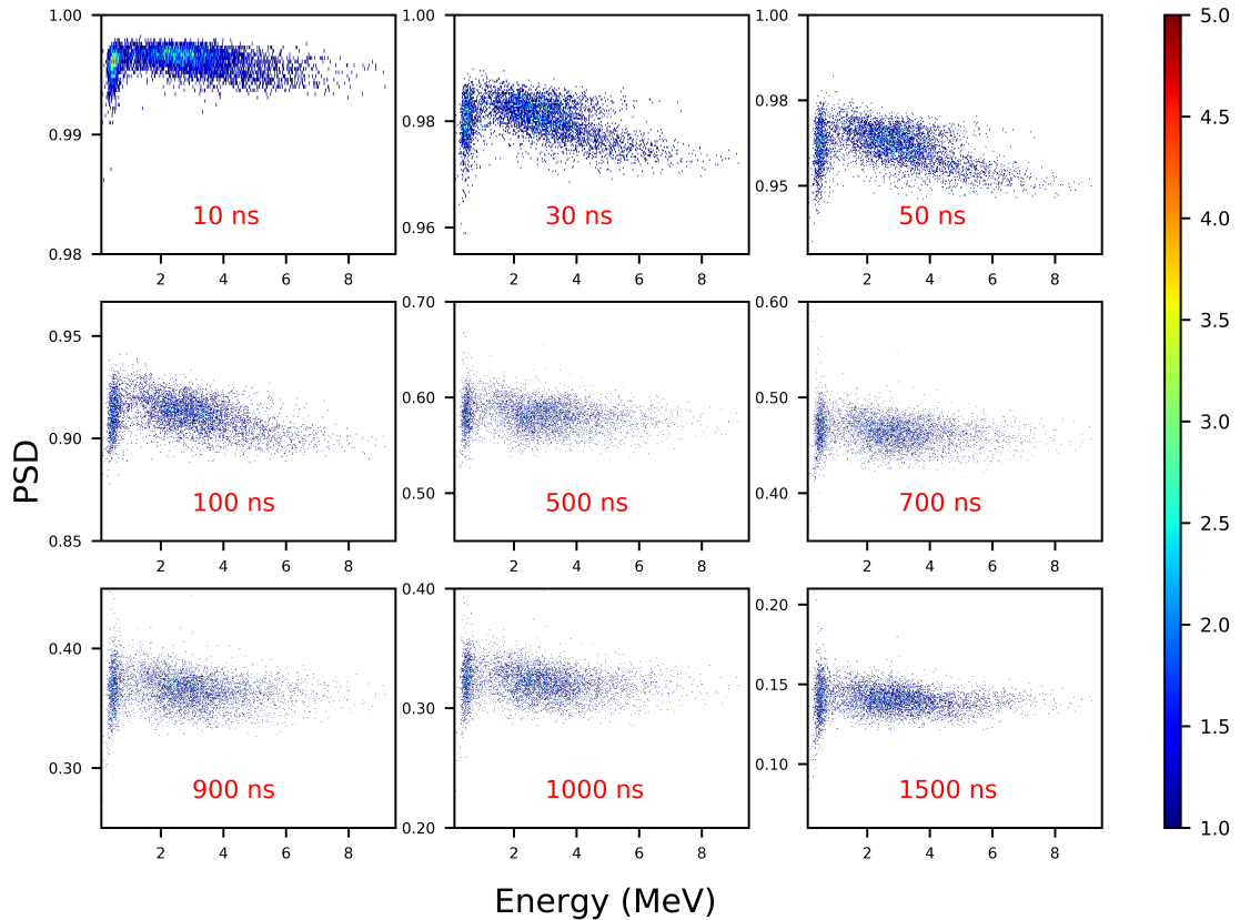
Figure 4.14: 2D histogram plots of the PSD versus energy for CLYC-7 of the neutron signals from an Am-Be source at different t_{prompt} . The value of t_{prompt} is indicated in each plot, whilst t_{delay} is constant ( 2 \mu s ).
