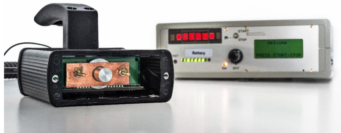
Figure 1.4: On the left, the active probe of one of the first prototypes of the B-RAD without the front cover to show the LaBr 3 crystal; on the right, the control unit.
