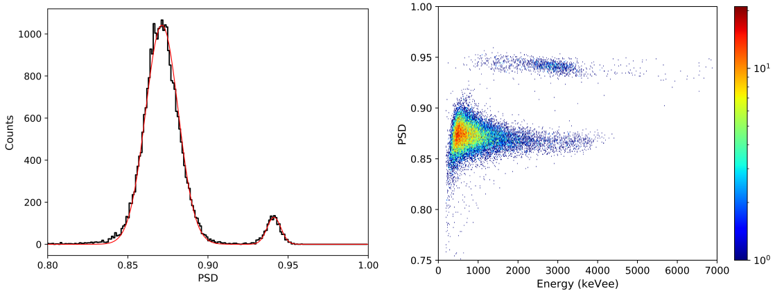
Figure 4.11: Left: the 1D PSD histogram plot acquired with CLYC-7 irradiated with 2.5 MeV neutrons from a D-D generator. The red line is the Gaussian fit to the \gamma -ray (left peak) and neutron (right peak) distributions. Right: the 2D PSD plot for the same measurement.
