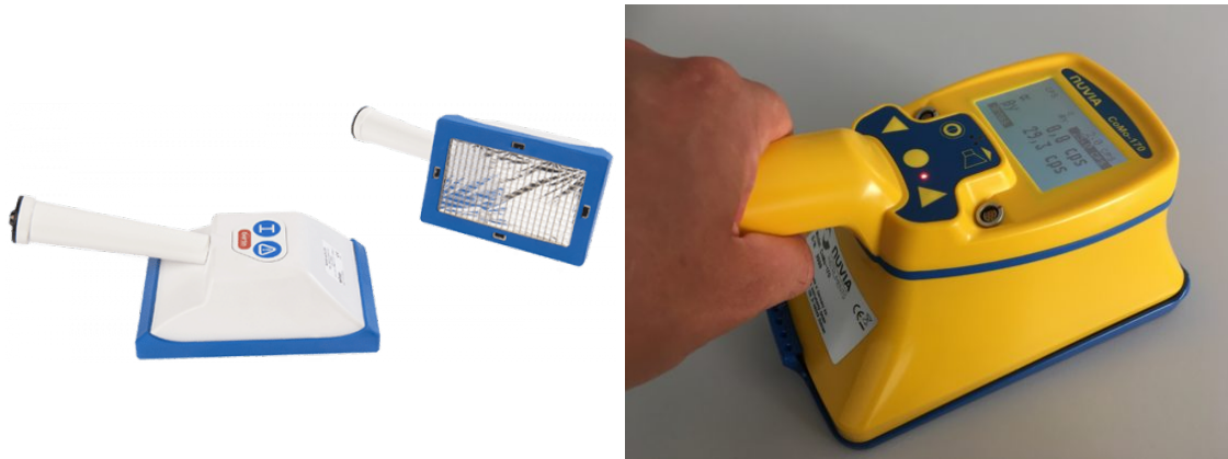
Figure 1.2: Two commercial devices for \alpha/\beta particle detection: the SaphyRAD A-B 170 probe from Bertin Technologies (on the left) and the CoMo 170 from NUVIATech Instruments (on the right).
