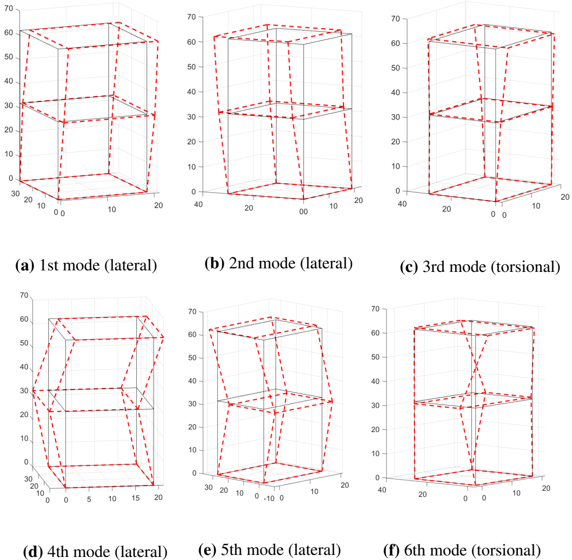
Fig. 25. The identified mode shapes of the frame
