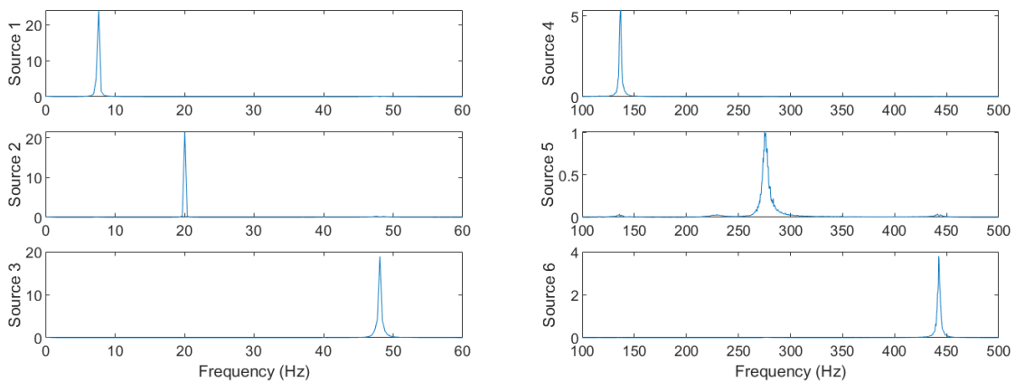
Fig. 16. Separated auto-PSD functions in the case of random noise accompanied by harmonic excitation
