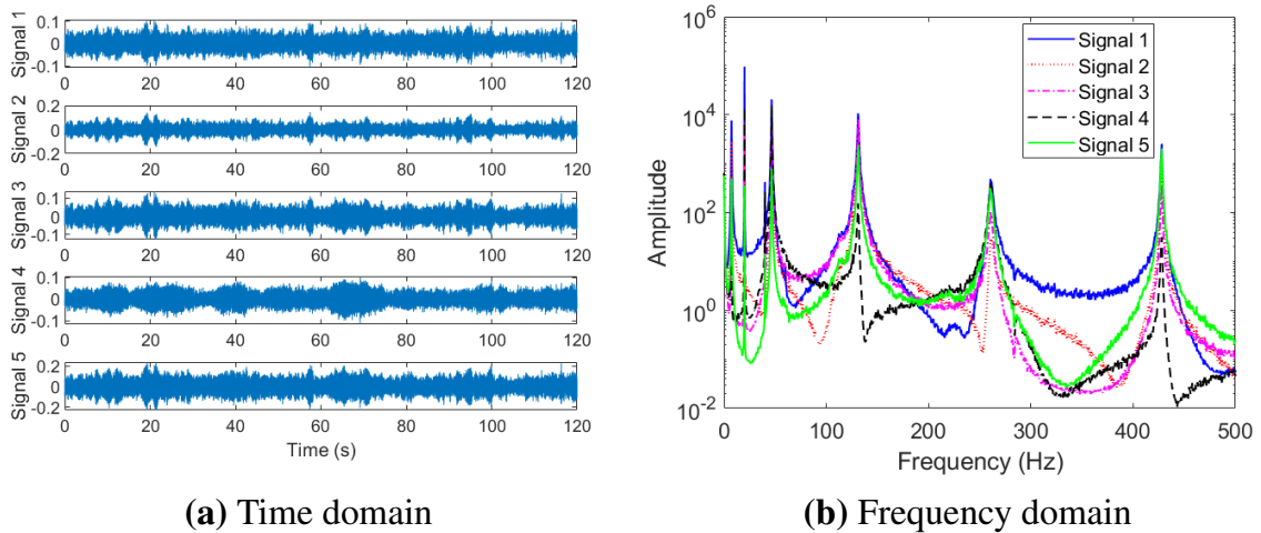
Fig. 14. Five measurement signals of the cantilever beam
