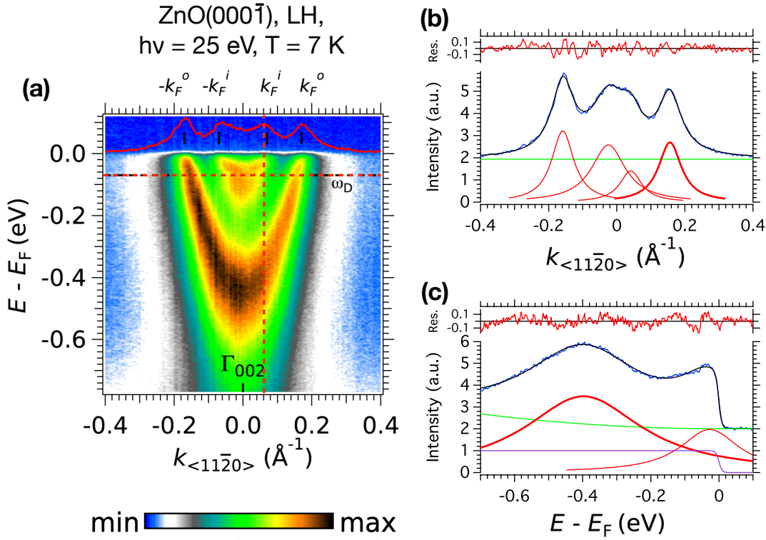
FIGURE 2.6: (a) Energy-momentum ARPES intensity map around the bulk \Gamma_{002} point along the in-plane k_{<11\bar{2}0>} direction, measured with linear-horizontal light polarization at h\nu = 25 eV and T = 7 K [82]. The red curve is the MDC over E_F \pm 5 meV. The black vertical bars show the Fermi momenta k_F^i and k_F^o of the inner and outer subbands. The Fermi liquid is coupled to phonons with a characteristic Debye energy \omega_D \approx 70 meV shown by the horizontal, dashed red line. (b) An example of a momentum-distribution curve (MDC) taken at binding energy E_{bind} = -\omega = (70 \pm 2) meV indicated with the horizontal dashed red line in panel (a). (c) A typical energy-distribution curve (EDC) taken at k = (0.06 \pm 0.002) \text{ \AA}^{-1} corresponding to the vertical dashed red line in panel (a). From the Lorentzian peak fit, the peak positions and the corresponding half widths at half maximum (HWHM) can be extracted and further used to determine the self-energy. Blue: experimental data; black: overall fit; red: Lorentzian peaks used; green: quadratic or constant background; purple: the Fermi-Dirac distribution with an effective temperature 50 K.
