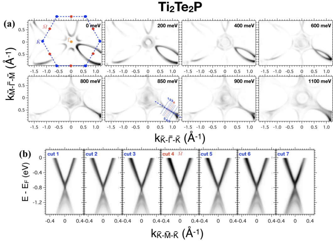
FIGURE 4.14: Experimental observation of the Dirac-node arc in \text{Ti}_2\text{Te}_2\text{P} by normal ARPES. (a) Constant energy mappings at various binding energies. (b) Dispersion maps along the \bar{K}-\bar{M}-\bar{K} direction along the cut directions indicated in the 850 meV constant energy contour panel where the nodal arc is presented. All data were collected at the CASSIOPEE high-resolution ARPES endstation at synchrotron Soleil with LH polarised h\nu = 50 eV photons at a temperature of T = 5 K.
