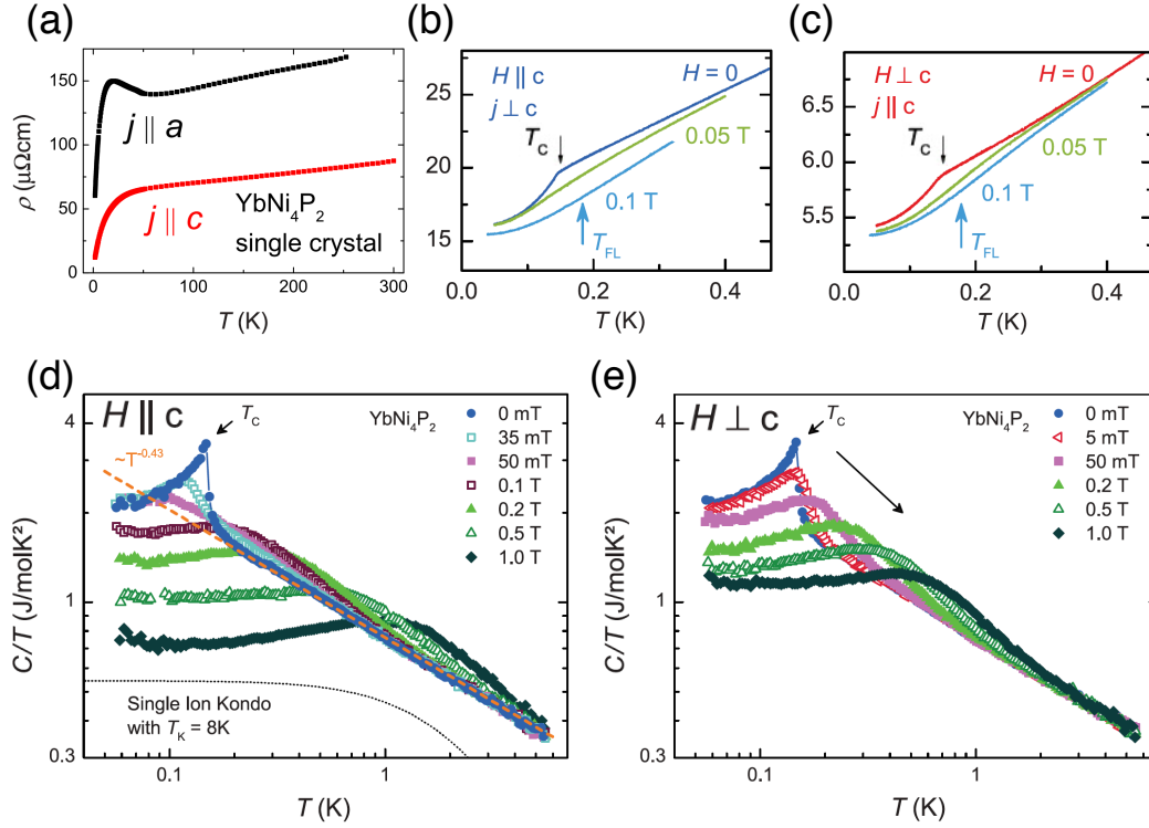
FIGURE 5.4: (a) Temperature dependence (above 1.8 K) of the electrical resistivity \rho with the current along the a (black) and the c (red) direction. The resistivity along c ( j \parallel c ) is distinctively smaller than along a in the whole investigated temperature range. Both directions display a pronounced drop towards lower temperatures due to the onset of coherent Kondo scattering. A pronounced Kondo maximum at T = 20 K is visible only for j \parallel a . Taken from Ref. [208]. (b, c) Temperature dependence (below 0.5 K) of the electrical resistivity \rho measured with current j (b) perpendicular and (c) parallel to the crystallographic c axis. The kinks at T_c disappear at fields \mu_0 H \geq 0.05 T in both field directions. At a field of 0.1 T, both resistivities follow a temperature dependence close to T^2 below T_{FL} (arrows). (d,e) C/T versus T of \text{YbNi}_4\text{P}_2 measured at magnetic fields (d) H \parallel c and (e) H \perp c . The dashed orange line emphasizes the T^{-0.43} power law behavior observed above 0.2 K up to about 6 K. The dotted black line is the specific-heat contribution calculated within the single ion S = 1/2 Kondo model in Ref. [218], with T_K = 8 K and C/T scaled by a factor of 0.5 for better visibility. In (d) and (e), the nuclear Schottky contribution has been subtracted from the raw specific-heat data. Taken from Ref. [52].
