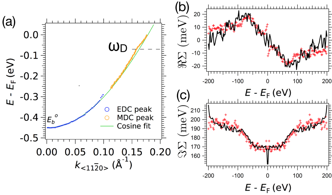
FIGURE 2.7: (a) Maxima of the EDC (blue circles) and MDC (orange circles) peaks for the outer subband of the 2DES at the \text{Al}(2\text{\AA})/\text{ZnO}(000\bar{1}) interface [82]. Only data for the right branch (positive momentum region) are shown. The continuous green curve is a cosine fit to the data representing the non-interacting electron dispersion of this subband. (b, c) The self-energy extracted from the left branch. The red markers are the results of \Re\Sigma ( \Im\Sigma ) determined directly from the experimental data, and the black lines are the results of Kramers-Kronig transform from the corresponding \Im\Sigma ( \Re\Sigma ).
