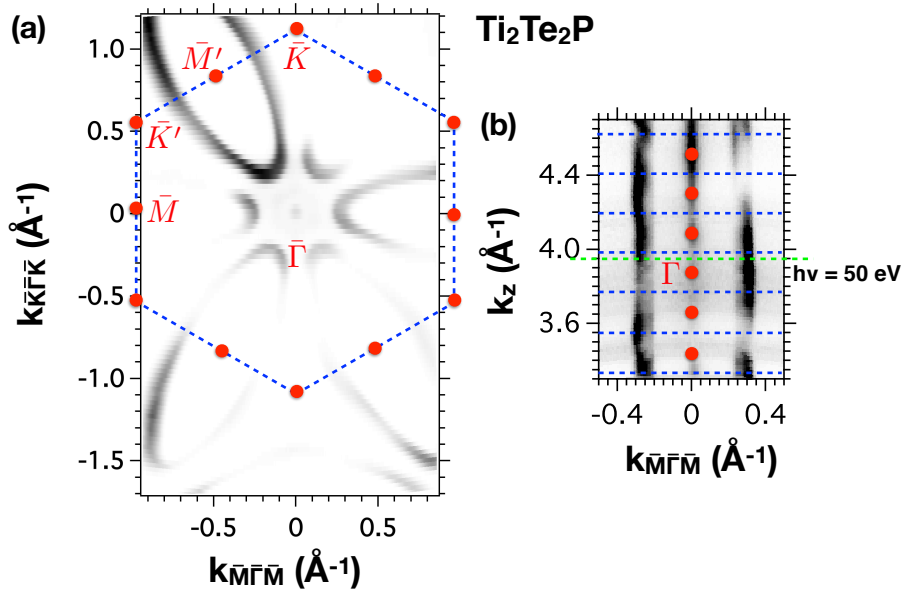
FIGURE 4.4: (a) In-plane Fermi surface of \text{Ti}_2\text{Te}_2\text{P} measured with LH polarised h\nu = 50 \text{ eV} photons. (b) Out-of-plane Fermi surface of \text{Ti}_2\text{Te}_2\text{P} measured at normal emission with linear vertical polarised photons by varying the photon energy from 40 eV to 84.5 eV with a step of 0.5 eV. All these data were obtained at T = 6 \text{ K} . A V_0 = 12 \text{ eV} inner potential is used in panel (b). In both panels, dashed blue lines represent the Brillouin zone boundaries.
