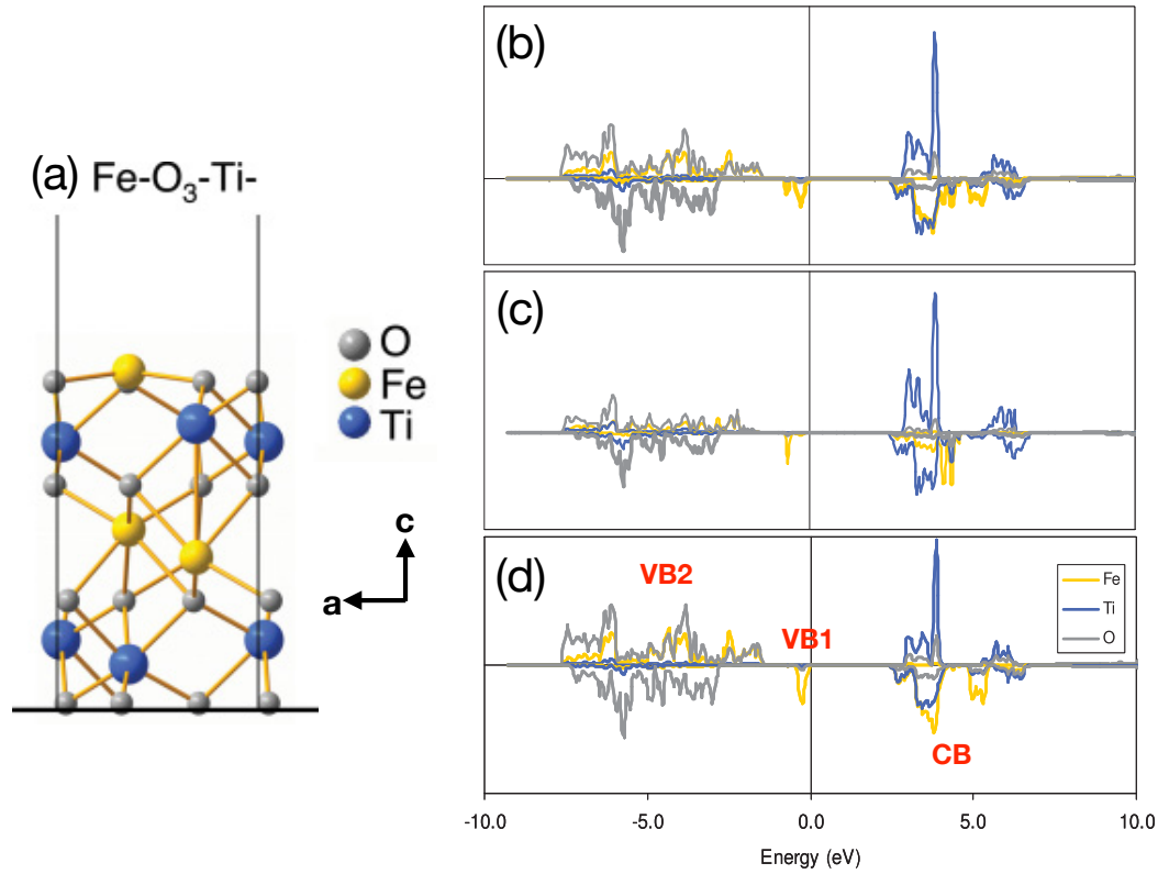
FIGURE 3.18: (a) Relaxed geometry of the \text{Fe-O}_3\text{-Ti-} terminated surface. (b-d) Electron DOS for the \text{Fe-O}_3\text{-Ti-} surface at ground state, calculated by using the hybrid density functional B3LYP. Total DOS decomposed to Fe (yellow), Ti (blue), and O (grey) is shown in panel (b), while panel (c) shows a decomposition of just the surface Fe, Ti, and O, and panel (d) shows the decomposition of the other layers. The top of the valence band is set to zero in energy. Taken from Ref. [173]
