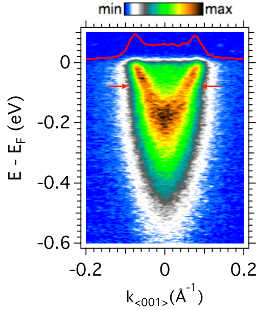
FIGURE 3.4: The energy-momentum dispersion of the 2DES measured at the \text{SnO}_2(110) surface with LH polarised photons at h\nu = 88 eV and T = 16 K. Electron-phonon interaction induces the observed deviations (red arrows) from a simple parabolic shape. The red curve above E_F is an MDC integrated over E_F \pm 10 meV.
