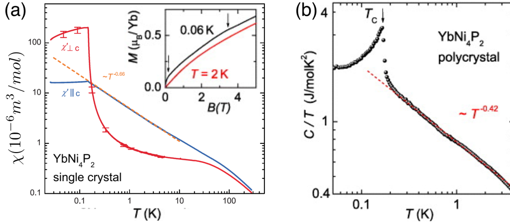
FIGURE 5.3: (a) Real part of the magnetic susceptibility \chi' plotted as a function of temperature, measured perpendicular ( \chi'_{\perp} ) and parallel ( \chi'_{\parallel} ) to the c axis in a \text{YbNi}_4\text{P}_2 single crystal. The orange dashed line emphasises the T^{-0.66} behavior of \chi'_{\parallel} versus T below 10 K. Taken from Ref. [52]. Inset: the field dependence of the magnetisation M(B) below (black line) and above (red line) T_C measured in a \text{YbNi}_4\text{P}_2 polycrystal. The arrow on the left-hand side indicates the step-like increase due to the small ordered ferromagnetic moment, M_{ord} \cong 0.05 \mu_B , obtained by extrapolating the linear curve between 0.1 and 0.2 T to zero field. In determining the ordered moment, we assume that in the polycrystal the fully aligned moment dominates the magnetisation at these low fields. The right-hand arrow marks an anomaly at a higher field representing either the rotation of the ferromagnetic moments along the magnetic hard direction or complete suppression of the Kondo screening. (b) The temperature dependence of the zero-field specific heat divided by temperature ( C/T ) in a double logarithmic representation clearly reveals a power law divergence, C/T = T^{-0.42} , indicated by the red dashed line, measured in a \text{YbNi}_4\text{P}_2 polycrystal. At the transition temperature T_c = 0.17 K, this specific heat curve shows a sudden jump resulting in a \lambda shape indicating a 2nd order phase transition. Taken from Ref. [51].
