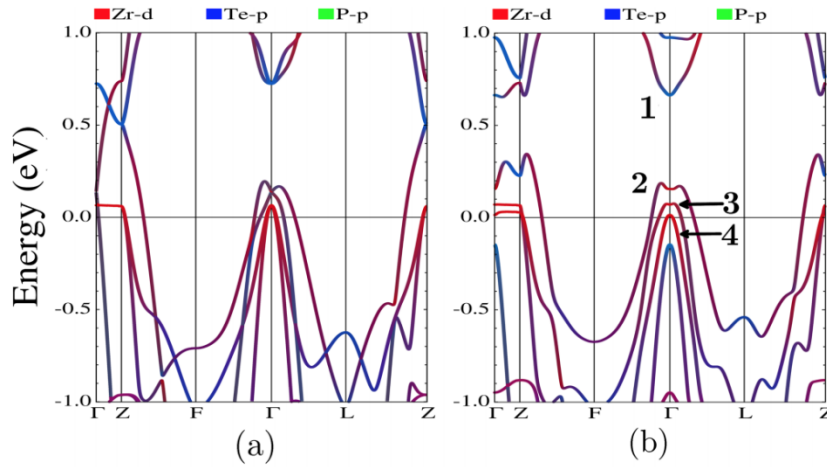
FIGURE 4.11: The Band structures of \text{Zr}_2\text{Te}_2\text{P} in the rhombohedral unit cell along the TRIM points (a) without the inclusion of the spin-orbit coupling (SOC) and (b) with the inclusion of SOC [189]. The colours used indicate the orbital character of the bands: red, blue, and green colours correspond to Zr d , Te p , and P p orbitals, respectively.
