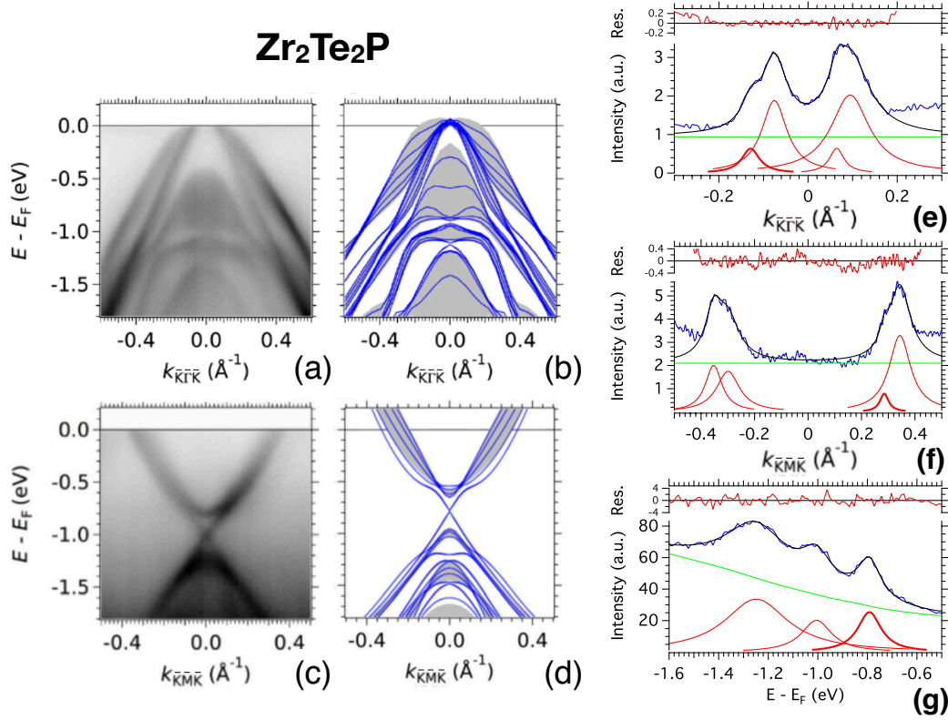
FIGURE 4.6: (a-d) Comparison between ARPES measurements and band structure calculations for \text{Zr}_2\text{Te}_2\text{P} for dispersions along the \bar{K} - \bar{\Gamma} - \bar{K} direction at \bar{\Gamma} (upper panels) and along the \bar{K} - \bar{M} - \bar{K} direction at \bar{M} (lower panels) [189]. (a) and (c) are ARPES determined band dispersions, while (b) and (d) are DFT calculated bands. Fermi level E_F is indicated by the horizontal black line. Blue solid lines are bands obtained from a 5-layer slab calculation and therefore represent surface states. The grey ribbons represent the surface-projected bulk bands. (e) Momentum distribution curve (MDC) at E_F (integrated over \pm 10 meV) of states around \bar{\Gamma} in panel (a). (f) Momentum distribution curve (MDC) at E_F (integrated over \pm 10 meV) of states around \bar{M} in panel (c). (g) Energy distribution curve (EDC) at \bar{M} (integrated over \pm 0.005 \text{ \AA}^{-1} ). These MDCs and EDCs (blue curves) are fitted with Lorentzian peaks (red peaks) and a quadratic (MDC) or Shirley (EDC) background (the green curve). The overall fits are the black curves, while the red line in each top inset is the fitting residual. These ARPES data were measured in PF, KEK, Japan with LH polarised photons at h\nu = 120 \text{ eV} and T = 20 \text{ K} .
