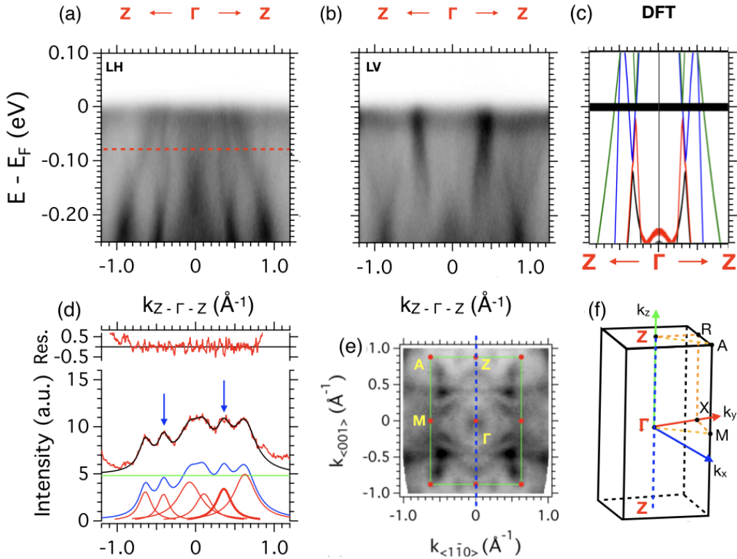
FIGURE 5.20: (a, b) Energy - momentum dispersions along Z - \Gamma - Z measured at h\nu = 90 eV and T = 16 K with (a) linear horizontal and (b) linear vertical polarised photons. The red dashed line in panel (a) indicates where the MDC shown in panel (d) was taken. (c) DFT calculated bands along Z - \Gamma - Z . The red band corresponds to FS 1, the 3D ellipsoid centred at \Gamma . The blue band corresponds to FS 2, the most typical quasi-1D Fermi sheets with small closed pockets slightly above and in the middle of the sheets. So from \Gamma to Z , there are 3 branches of blue band crossing the Fermi level: first the quasi-1D sheet, then the two boundaries of small closed pockets. The green band corresponds to FS 3, the other quasi-1D Fermi sheet together with small cylindrical Fermi surfaces crossing the A - Z - R planes. (d) An MDC taken at binding energy 80 meV within an integration range \pm 2 meV. The blue arrows indicate the momentum positions ( \approx \pm 0.4 \text{ \AA}^{-1} ) of the quasi-1D sheets shown in panel (e). (e) Symmetrised in-plane constant energy map at binding energy 80 meV, identical to Fig. 5.14(a), measured with the detector slit aligned along \langle 001 \rangle direction, as indicated with the blue dashed line. (f) Sketch of the first Brillouin zone. The blue dashed line indicates the detector slit.
