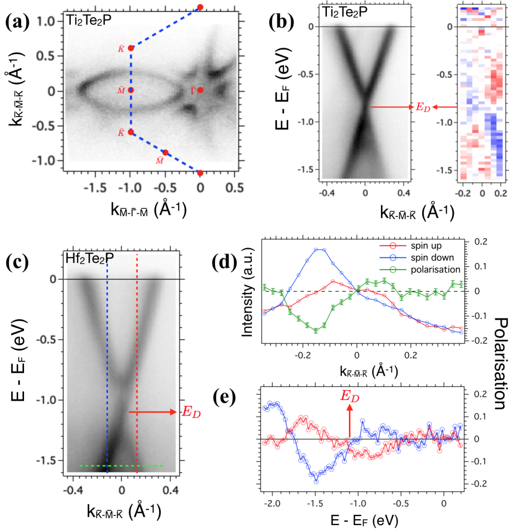
FIGURE 4.16: (a) In-plane Fermi surface map of Ti 2 Te 2 P showing a 3-fold symmetry. (b) Energy-momentum dispersion of Ti 2 Te 2 P at \bar{M} point along \bar{K} - \bar{M} - \bar{K} direction showing a Dirac crossing point around 0.85 eV below E_F , and the corresponding spin-resolved energy-momentum dispersion showing a clear spin polarisation of the non-trivial Dirac surface state (red: pointing towards readers; blue: pointing away from readers). (c) The energy-momentum dispersion of states of Hf 2 Te 2 P at \bar{M} point along \bar{K} - \bar{M} - \bar{K} direction showing a Dirac crossing point around 1.1 eV below E_F . (d) The spin-resolved MDC taken at binding energy indicated by the green dashed line in (c). (e) The spin-resolved EDCs indicated in (c) with the blue and the red dashed lines. All data were collected at the ESPRESSO spin-ARPES endstation in synchrotron HiSOR with LH polarised h\nu = 55 eV photons at a temperature of T = 20 K. The effective Sherman function used to obtain the spin polarisation is 0.18, as calibrated for h\nu = 55 eV with Bi(111) during the beam time in HiSOR in 2017.
