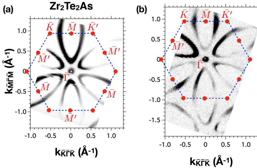
FIGURE 4.5: (a-b) In-plane Fermi surfaces of \text{Zr}_2\text{Te}_2\text{As} measured with (a) LH, and (b) LV polarised h\nu = 50 \text{ eV} photons. All these data were obtained at T = 6 \text{ K} . In both panels, dashed blue lines represent the Brillouin zone boundaries.
