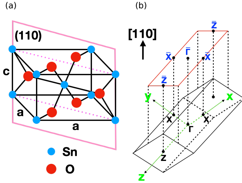
FIGURE 3.1: (a) 3D unit cell of \text{SnO}_2 with a = 4.737 \text{ \AA} and c = 3.185 \text{ \AA} ; (b) Corresponding 3D Brillouin zone of rutile \text{SnO}_2 (black parallelepiped) together with the surface Brillouin zone projected on the (110) plane (red rectangle).
