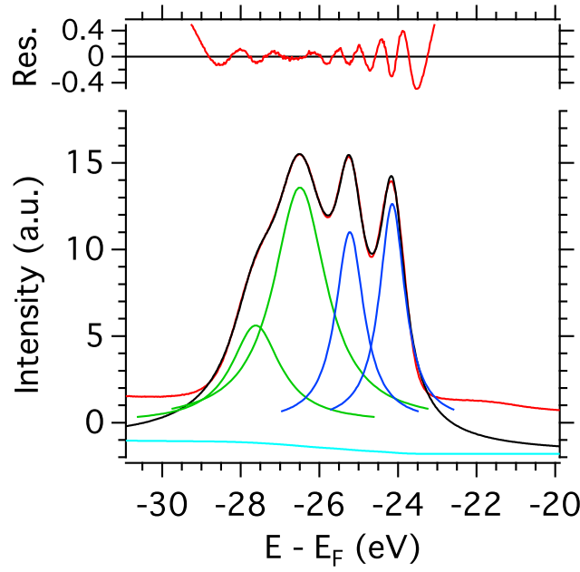
FIGURE 3.13: Numerical fit of the Sn 4d core levels in the binding energy range from 23 eV to 29 eV. Red: the experimental line-shape measured after 1 ML of Eu deposition at \text{SnO}_2(110) surface. Black: the final fitting result. Green: \text{SnO}_x 4d peaks. Blue: metallic Sn 4d peaks. Sky blue: the Shirley background. The red line in the inset above is the fitting residual.
