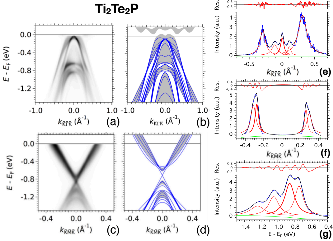
FIGURE 4.8: (a-d) Comparison between ARPES measurements and band structure calculations for \text{Ti}_2\text{Te}_2\text{P} for dispersions along the \bar{K} - \bar{\Gamma} - \bar{K} direction at \bar{\Gamma} (upper panels) and along the \bar{K} - \bar{M} - \bar{K} direction at \bar{M} (lower panels) [189]. (a) and (c) are ARPES determined band dispersions, while (b) and (d) are DFT calculated bands. Fermi level E_F is indicated by the horizontal black line. Blue solid lines are bands obtained from a 5-layer slab calculation and therefore represent surface states. The grey ribbons represent the surface-projected bulk bands. (e) Momentum distribution curve (MDC) at E_F (integrated over \pm 10 meV) of states around \bar{\Gamma} in panel (a). (f) Momentum distribution curve (MDC) at E_F (integrated over \pm 10 meV) of states around \bar{M} in panel (c). (g) Energy distribution curve (EDC) at \bar{M} (integrated over \pm 0.005 \text{\AA}^{-1} ). These MDCs and EDCs (blue curves) are fitted with Lorentzian peaks (red peaks) and a quadratic (MDC) or Shirley (EDC) background (the green curve). The overall fits are the black curves, while the red line in each top inset is the fitting residual. These ARPES data were measured in CASSIOPEE in SOLEIL, France with LH polarised photons at h\nu = 50 eV and T = 6 K.
