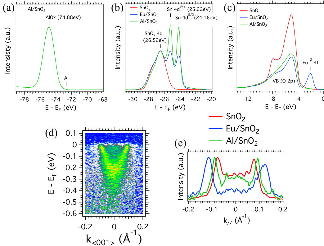
FIGURE 3.10: (a-c) XPS profiles of (a) Al 2p core level after Al deposition; (b) Sn 4d core levels at bare, Al capped and Eu capped surface of \text{SnO}_2 ; (c) valence bands of \text{SnO}_2 and \text{Eu}^{2+} 4f core level. (d) Energy-momentum dispersion of the 2DES at the Al/ \text{SnO}_2 (110) interface obtained after deposition of 2 Å Al, measured with LH photons at h\nu = 88 eV. (e) Comparison of the MDCs at E_F (integrated over \pm 10 meV) of the 2DESs at the bare (red), Eu-capped (blue) and Al-capped (green) \text{SnO}_2 surface. All the measurements were carried out at T = 16 K.
