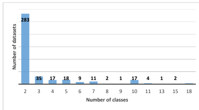
Figure C.1: Histogram of the number of classes in our datasets.
