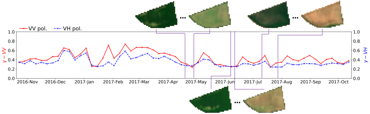
Figure 2.11: Average \gamma_{VV} and \gamma_{VH} time series over the Mâcon alfalfa grassland previously studied. Increased coherence values are observed after the three management practices. This is due to a high temporal stability of ground cover compared to vegetation.
