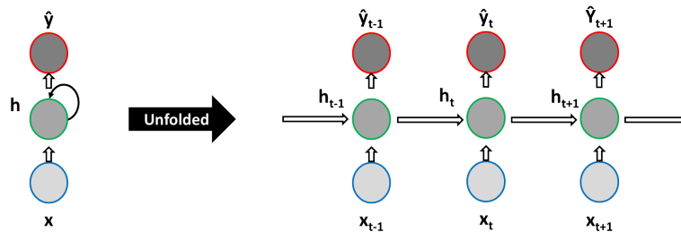
Figure 3.4: Schematic representation of a folded RNN on the left, and unfolded on the right. x are the inputs, h are the hidden states, \hat{y} are the outputs and t the time steps.
