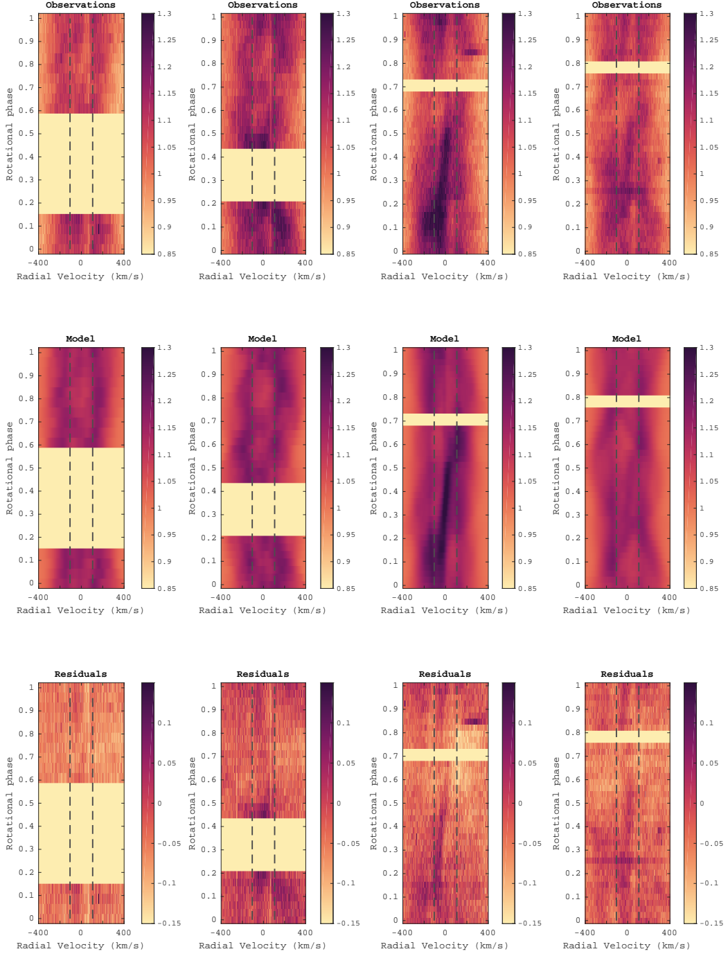
Figure 3.6.4: Dynamic spectrum for H \alpha , including the observations (Top), the tomography models (Middle), the residuals between observation and model (Bottom). From left to right, the figure show the data of 17, 18, 22, 23 Oct 2018, with color scale by the normalized flux. Rotational phases are computed according to Eq. 3.2.1. Vertical dash lines show the position of v \sin i .
