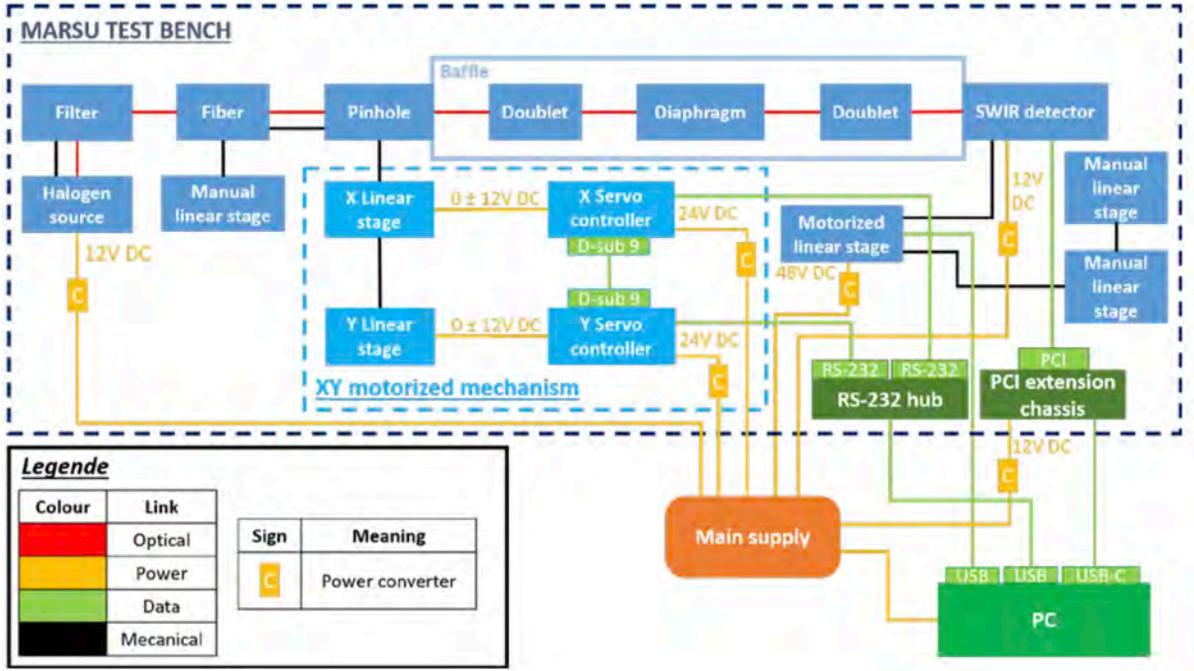
Figure 4.5.1: Principle of the MARSU bench
