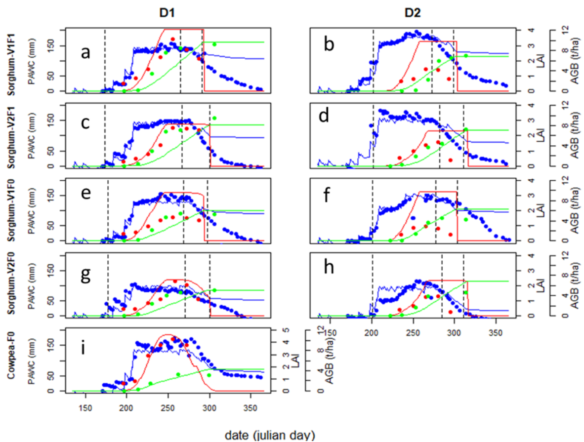
Fig. 3: Observed plant available soil water to maximum measurement depth (PAWC) (blue dots), LAI (red dots), and aboveground biomass (green dots) for the eight sole sorghum simulation units and one sole cowpea simulation unit used for model calibration. The lines are model simulations: blue for soil water to maximum measurement depth, red for LAI and green for AGB. Local variety (V1), improved variety (V2), early sowing (D1), late sowing (D2), no fertilizer (F0), 38 kgN ha -1 (F1) at Ntarla research station in 2018. Vertical dotted bars indicate from left to right sowing date, beginning of grain filling and physiological maturity.
