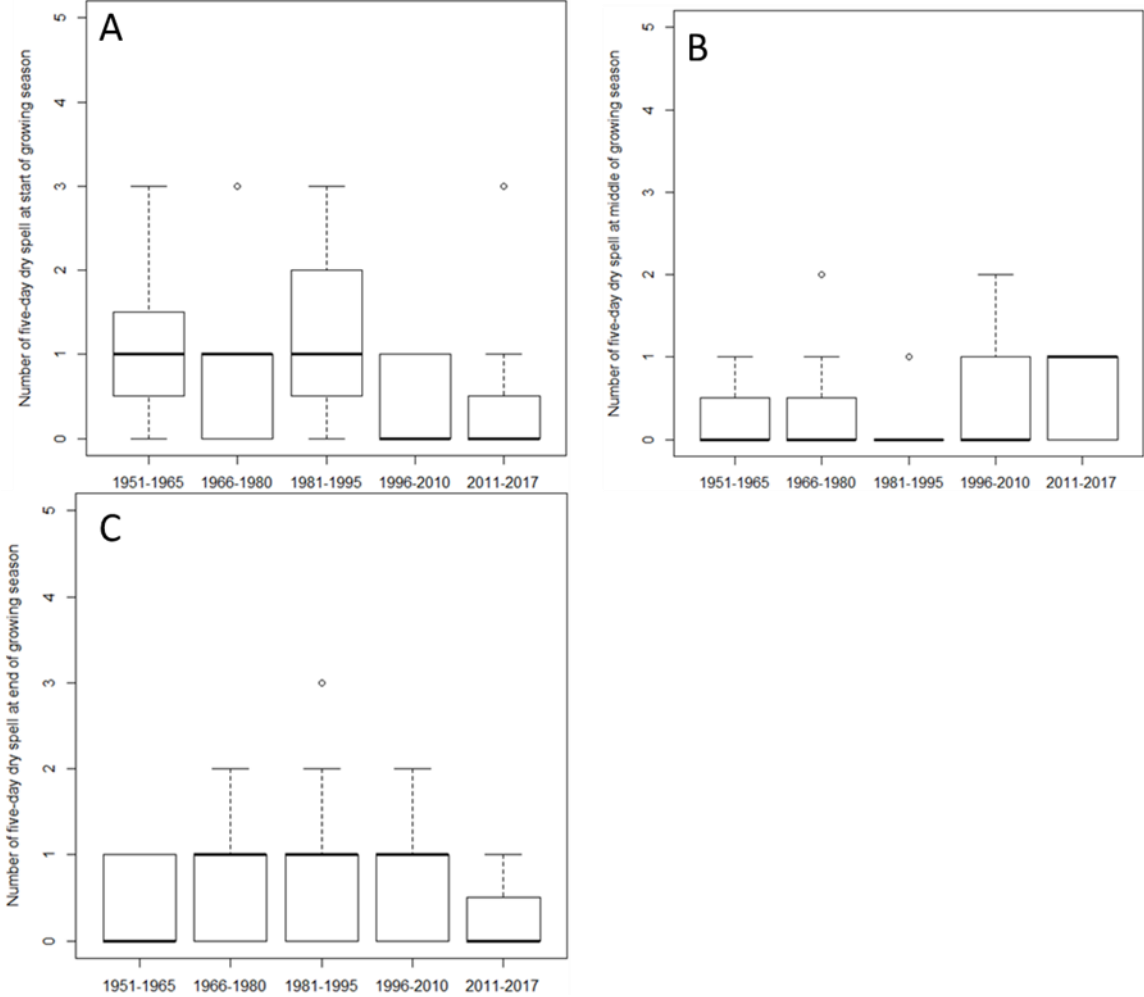
Figure 5: Number of five-day dry spells at the start (A), middle (B) and end (C) of the growing season for five periods from 1951 to 2017 at N'tarla weather station in Mali. The line in the box and the width of the box are the median and the interquartile range respectively. The whiskers extend from the edge of the box to the most extreme data point below 1.5 interquartile range.
