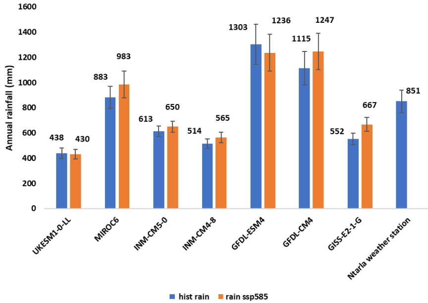
Figure S2: Observed (Ntaria weather station) and simulated (seven CMIP6 climate models) average annual rainfall for historical (1980-2010) and future (2035-2065) period. The bars represent the standard deviation of the average.
