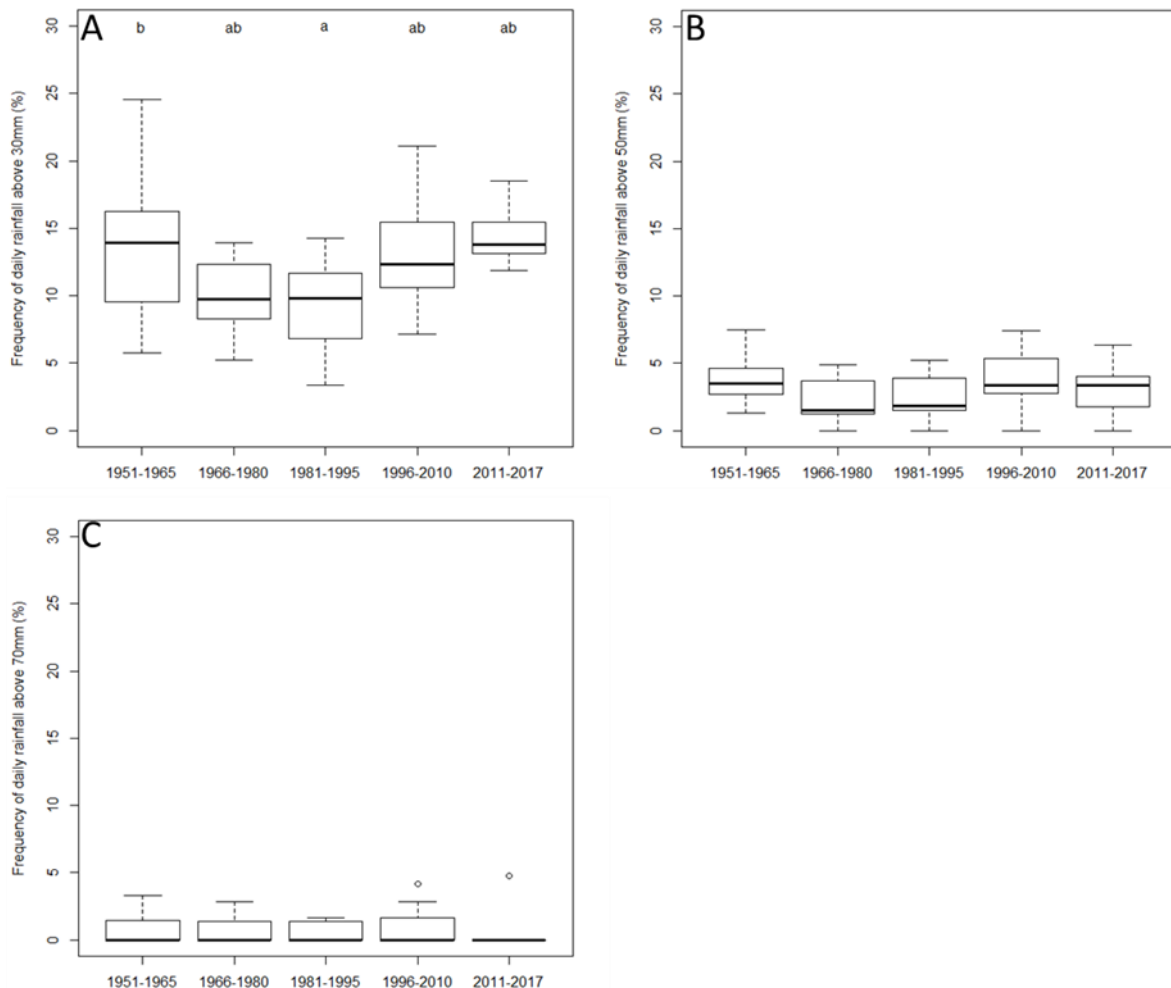
Figure 4: Frequency of intense rainfall events, >30mm (A), >50mm (B) and >70 mm (C), during the growing season for five periods from 1951 to 2017 at N'tarla weather station in Mali. Significant ( P<0.05 ) differences between periods are indicated with letters on top of boxplots. The line in the box and the width of the box are the median and the interquartile range respectively. The whiskers extend from the edge of the box to the most extreme data point below 1.5 interquartile range.
