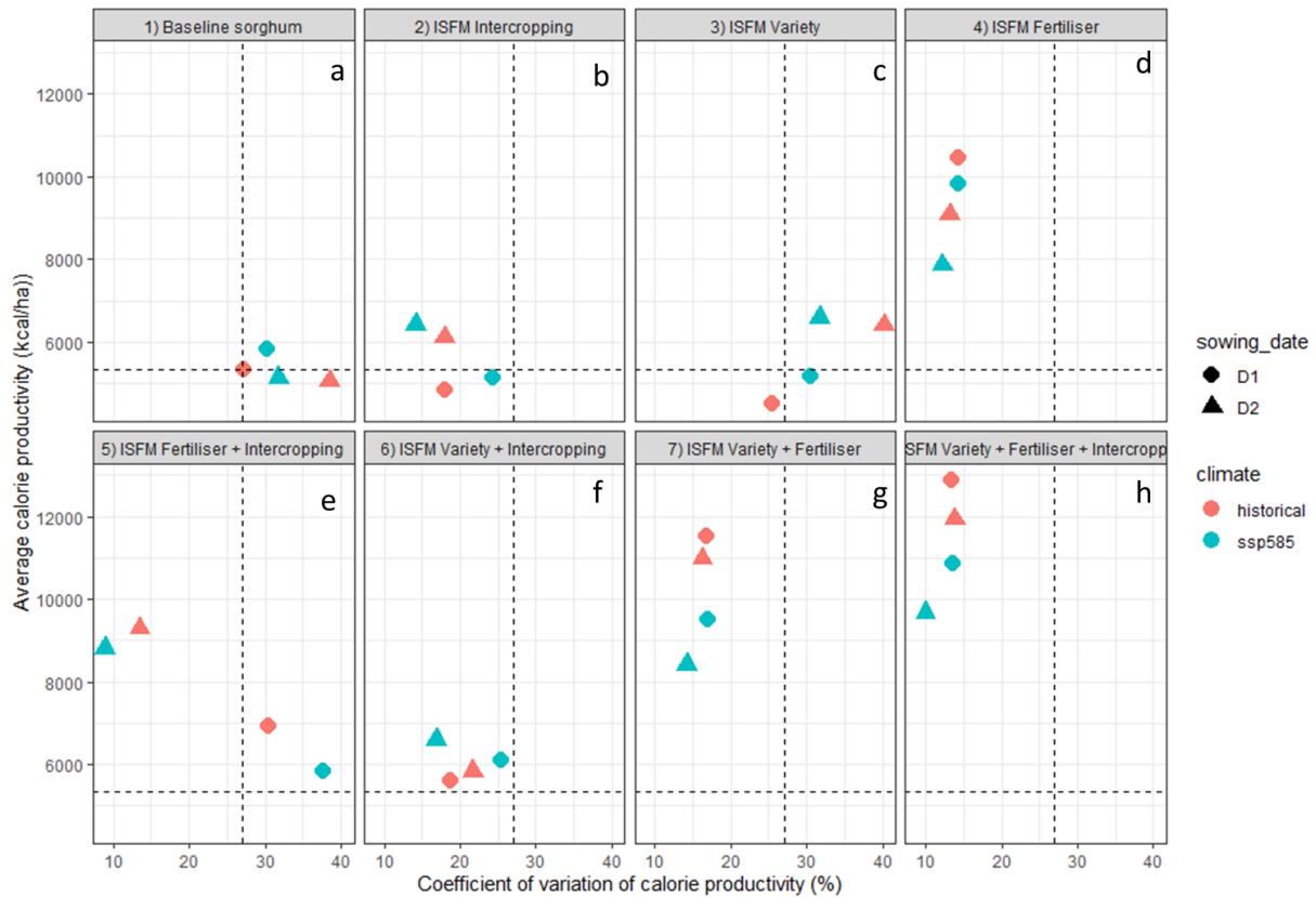
Figure 2: Average calorie productivity (kcal/ha) of seven crop management options and their interannual variability for early sowing and late sowing. ssp585 = more pessimistic climate scenario, ISFM = integrated soil fertility management. The horizontal dotted line in Figure 2 shows the average calorie productivity of the “baseline sorghum” option with current climate, and the vertical dotted line shows the coefficient of variation of this option with current climate. D1=early sowing, D2=late sowing.
