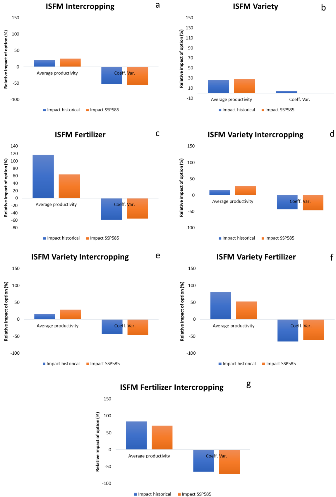
Figure S5: Relative impact (compared with the “baseline sorghum” option) of seven options on average calorie productivity and its coefficient of variation (Coeff. Var.) for historical and future climate in late sowing date.
