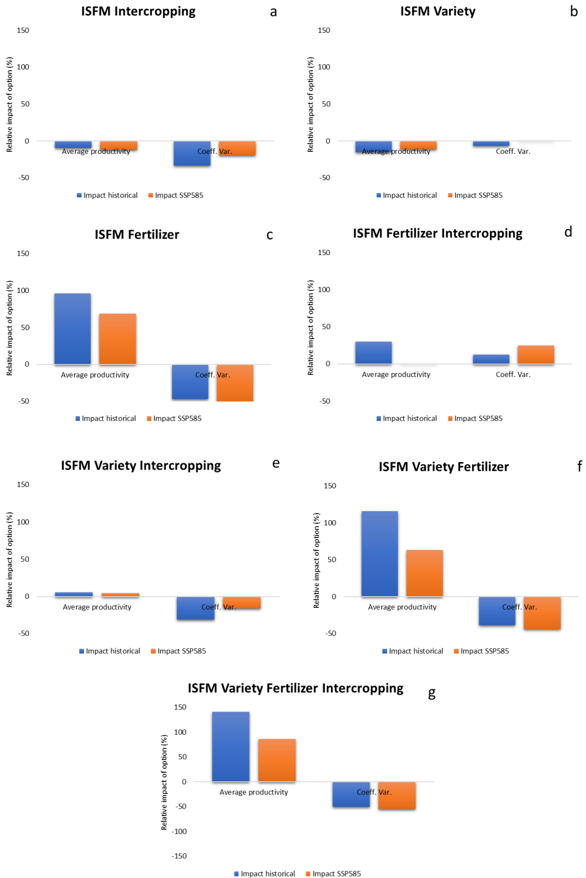
Figure S4: Relative impact (compared with the “baseline sorghum” option) of seven options on average calorie productivity and its coefficient of variation (Coeff. Var.) for historical and future climate in early sowing date.
