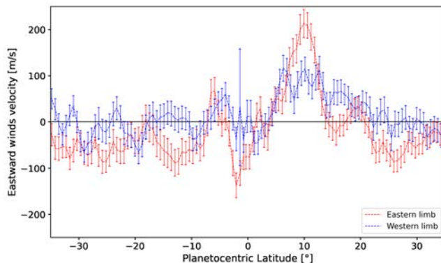
Fig. 1. Eastward wind velocities at 1 mbar as measured with ALMA on 22 March 2017, on the eastern and western limbs of Jupiter (adapted from Cavalié et al. 2021).
