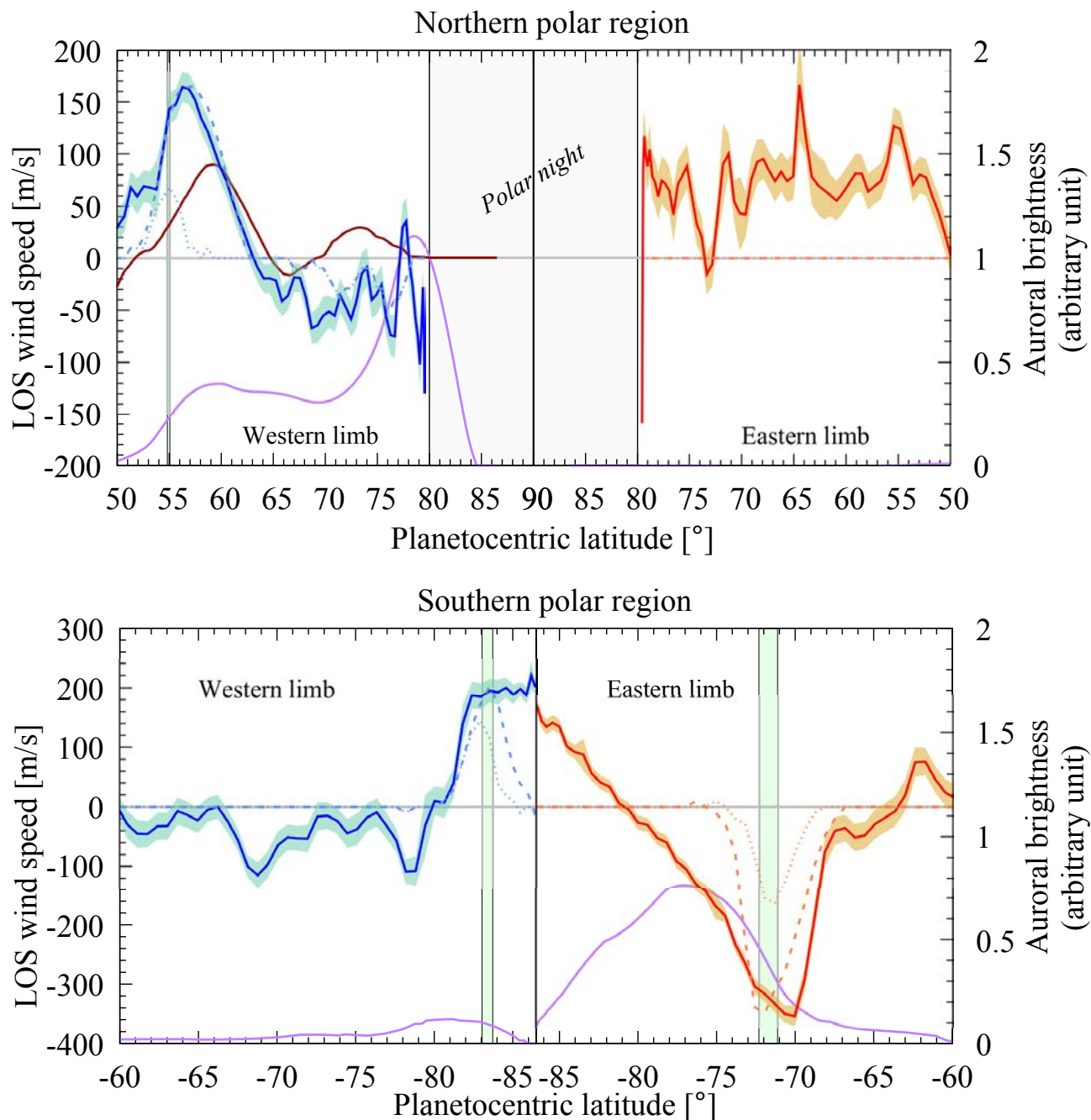
Fig. E.1. Comparison of models with observations: comparison between LOS velocities measured at 0.1 mbar with ALMA (same color code as in Fig. 2, top) and simulation results. A model with constant counterrotation winds within the ovals as defined by Bonfond et al. (2012) results in too narrow wind peaks, as shown with the dotted light blue and orange lines, regardless of the wind speed. The dashed light blue and orange lines are produced with constant counterrotation winds within the auroral ovals of 300 \text{ m s}^{-1} (north) and 370 \text{ m s}^{-1} (south) in the case of extended ovals, as described in the main text. The latitudes swept by the M = 30 footprints of the Connerney et al. (2018) magnetic field model are plotted with green stripes. The wind peaks are found within 1\text{--}2^\circ of these footprints. The statistical UV brightness model (purple line) derived from the observations of Clarke et al. (2009) and the ionospheric winds (brown line; speeds divided by five on the plot for an easier comparison) derived from the H 3 + infrared observations of Johnson et al. (2017) are also included for a qualitative comparison with our measured wind speeds. Both UV brightness and H 3 + wind curves have been degraded to the ALMA spatial resolution. The data from Johnson et al. (2017) are taken from their Fig. 8f. The northern auroral region is in the top panel, and the southern auroral region is in the bottom panel.
