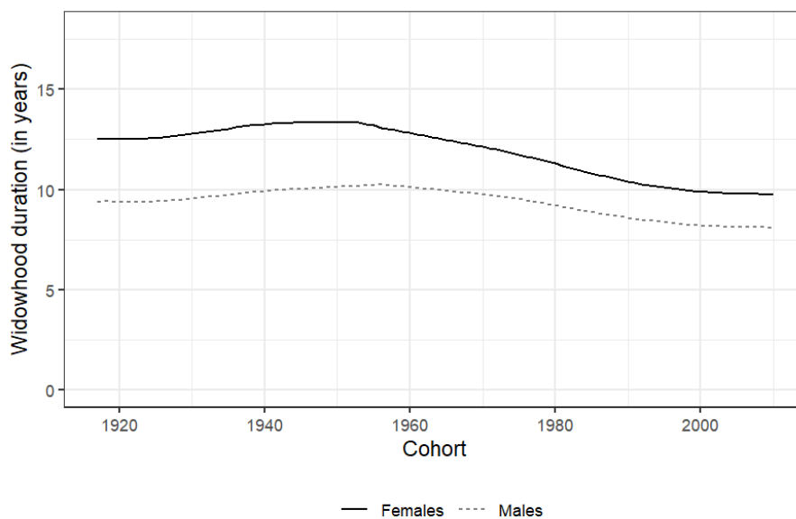
Figure 2.B.1: Widowhood duration variation over cohorts
