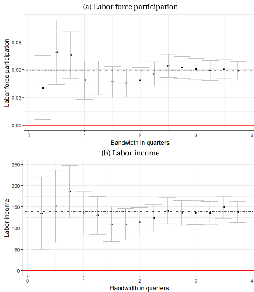
Figure 5.B.3: Effect of the reform: sensitivity to bandwidth
