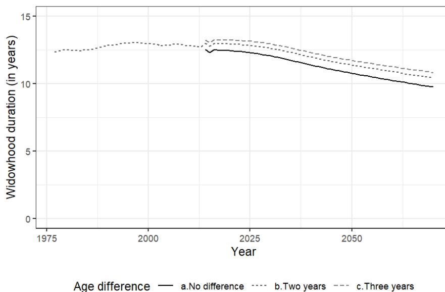
Figure 2.3: Female widowhood duration according to age difference between spouses
