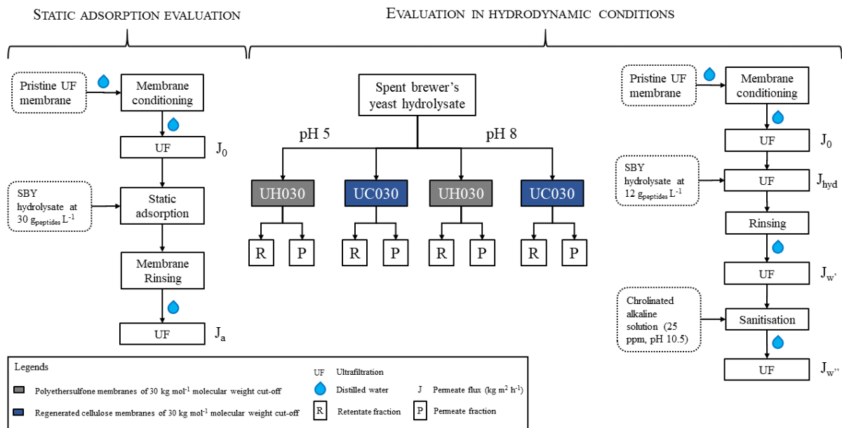
Figure 1: Experimental strategy to evaluate membrane performance during ultrafiltration of spent brewer's yeast (SBY) hydrolysate at static and hydrodynamic conditions.
