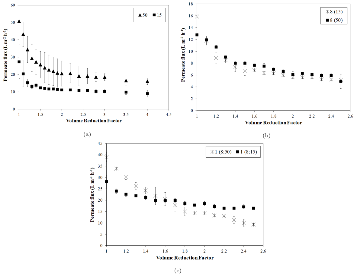
Figure 4: Permeate flux of spent brewer's yeast hydrolysate at fractionation steps 1 (50 or 15 kg \cdot mol^{-1} molecular weight cut-off, MWCO) (a), 2 (8 kg \cdot mol^{-1} MWCO) (b) and 3 (1 kg \cdot mol^{-1} MWCO) (c)
