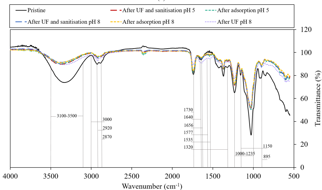
Figure 8: FT-IR spectra of pristine, after static adsorption, ultrafiltration and sanitisation in membranes with molecular weight cut-off of 30 kDa, made of polyethersulfone (a) and regenerated cellulose (b).
