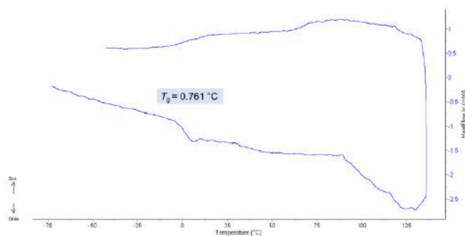
Figure 4.34 – DSC thermogram (heating rate of 10 °C \text{min}^{-1} , second heating cycle –80 to 140 °C) of: syndiotactic \text{PBPL}^{\text{OTBDMS}} ( P_r 0.83) synthesized by ROP of \text{rac-BPL}^{\text{OTBDMS}} with 2b / i PrOH (Table 4. 8; entry 4).
