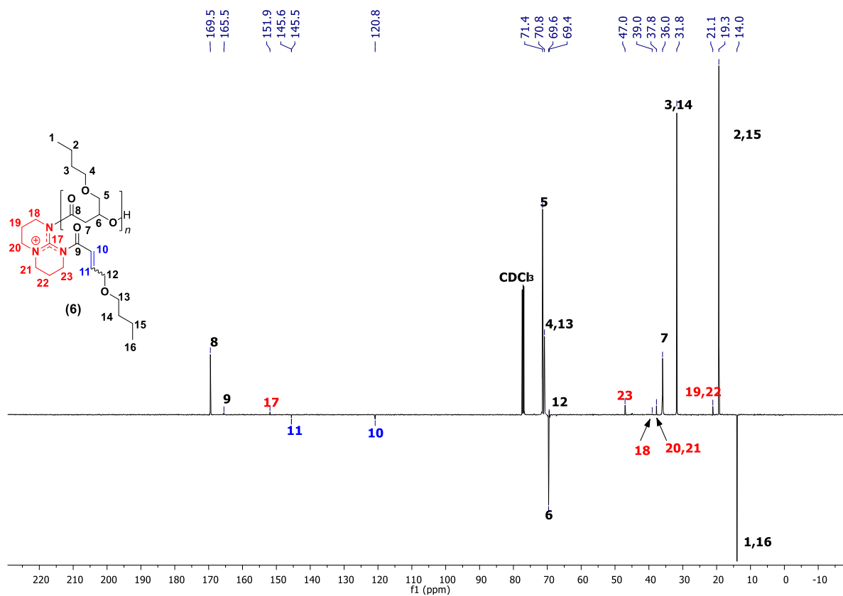
Figure 3. 16 – ^1\text{H} (500 MHz, \text{CDCl}_3 , 25 ^\circ\text{C} ) (top) and J-MOD (125 MHz, \text{CDCl}_3 , 25 ^\circ\text{C} ) (bottom) NMR spectra of PBPL n Bu recovered from the ROP of rac -BPL n Bu mediated by TBD (Table 3. 4); depicting only one ( I , Scheme 3. 19 – ( 13 )) out of the two populations ( I and II , Scheme 3. 19 – ( 13 ), ( 15 )) observed by MALDI-ToF MS (Figure 3. 19).
