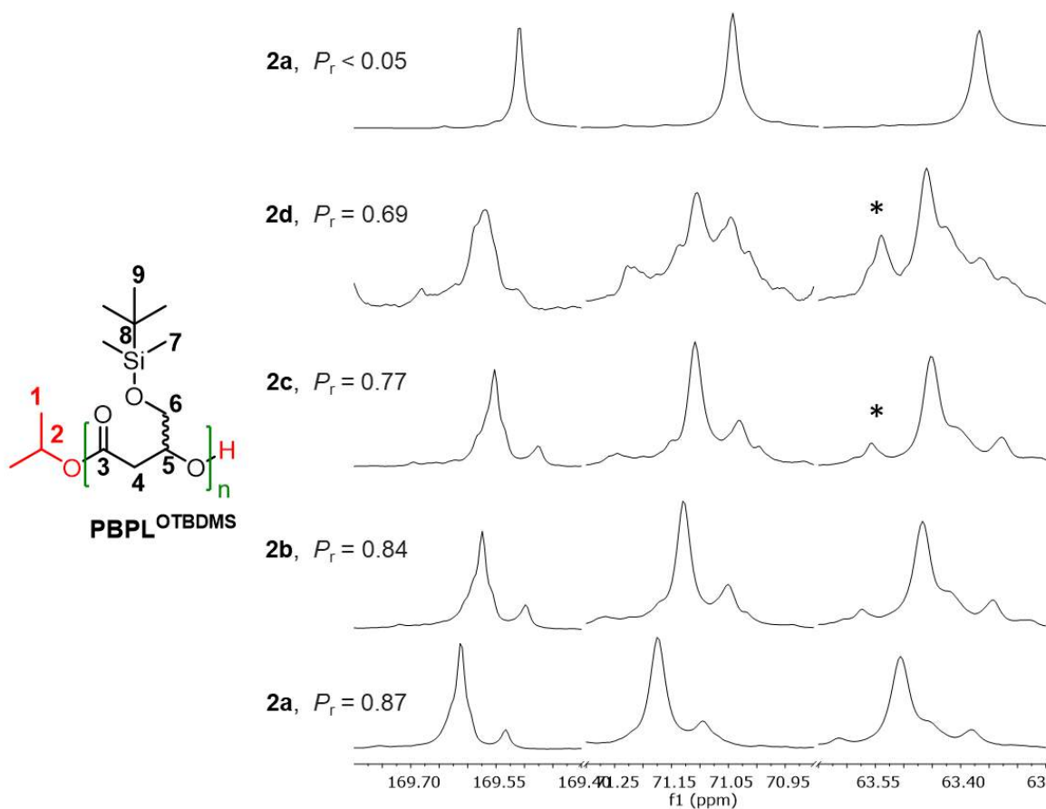
Figure 4.33 – Regions of the ^{13}\text{C}\{^1\text{H}\} NMR spectra (125 MHz, \text{CDCl}_3 , 23 °C) of \text{PBPL}^{\text{OTBDMS}} prepared by ROP of \text{rac-BPL}^{\text{OTBDMS}} , except for the top spectra: of enantiopure ( S )- \text{BPL}^{\text{OTBDMS}} (Table 4. 8, entry 8), mediated by 2a , 2b , 2c , or 2d / i PrOH (Table 4. 8, entries 1,3,5,7); * residual monomer.
