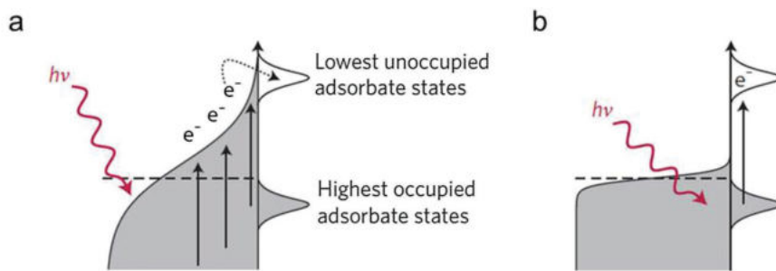
Figure 2.9 Schematic representation of HEA processes (a) photoexcited electron from the metal tunnels into the LUMO state of the molecule (b) Surface plasmon decay provoke electronic transition from the HOMO to the LUMO state. Extracted from [77].
