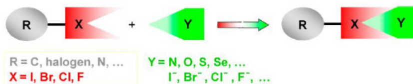
Figure 4.3 Schematic representation of halogen bond [135].
