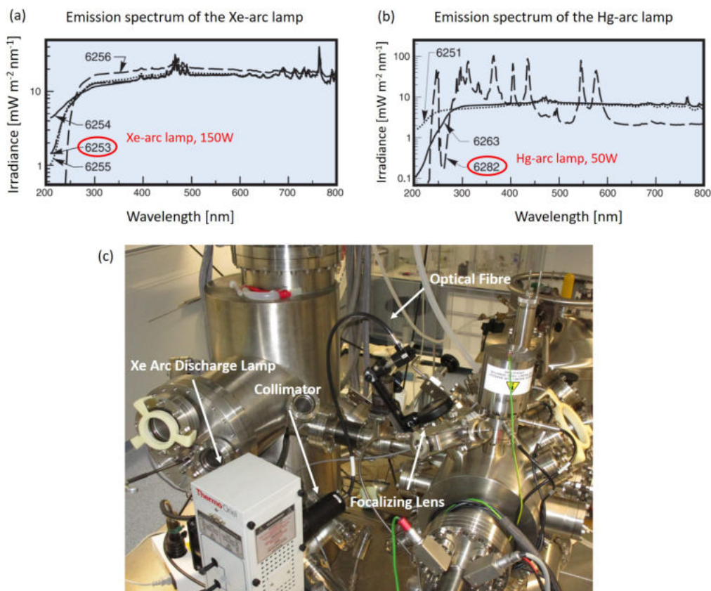
Figure 2.18 Emission spectra of the Xe (a) and Hg (b) arc-lamp. The spectrum corresponding to the lamp we have used is marked by red circle [93], (c) Experimental setup for UV-light irradiation; the light, emitted by the Xe arc-lamp, is collimated into the optical fibre entrance and guided in front of the window of the vacuum chamber. It was then focused onto the sample inside the chamber, probably some tens of mW optical power reached the sample.
