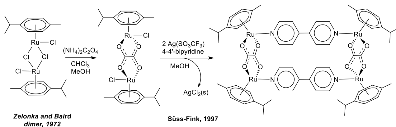
Scheme 1. Synthesis of rectangle metallacage by Süss-Fink and co-workers in 1997.
