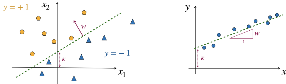
(a) Classification: Two-dimensional linear classification with dimensions d = 2 , k = 1 , n = 14 . \hat{y} = \text{sign}(\mathbf{w}^\top \mathbf{x} + \kappa)
