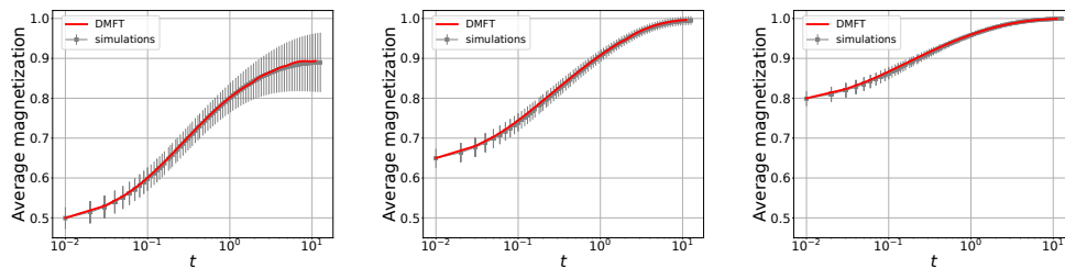
(a) Average magnetisation as a function of training time t for the full-batch GD algorithm. We consider \alpha = n/d = 2 and three different initialisations: m_0 = 0.5 (left), m_0 = 0.65 (center), m_0 = 0.8 (right). The grey dots represent numerical simulations ( d = 1000 , dt = 0.01 ), averaged over 1000 seeds (generating a new dataset and signal for each seed). The full red line marks the theoretical prediction from DMFT obtained in the high-dimensional limit of gradient-flow.
