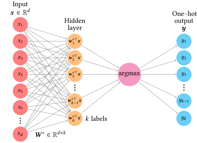
(a) Multi-class teacher-student perceptron.
