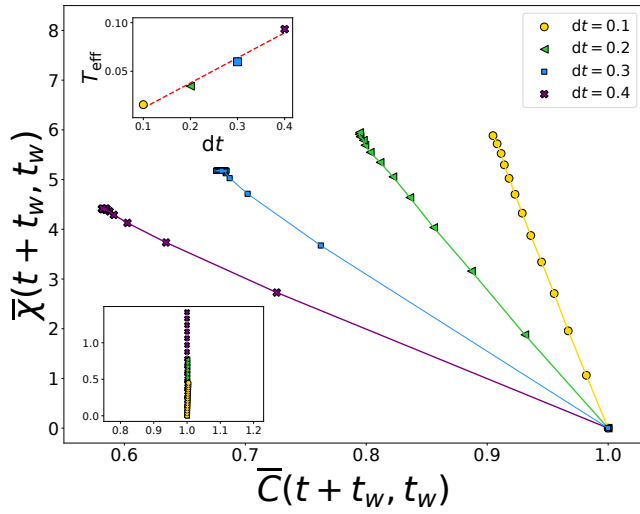
Figure 2.3.1 – FDT plot for vanilla-SGD . Top panel: the different curves represent different choices of learning rate dt = 0.1, 0.2, 0.3, 0.4 . The main plot is obtained in the UNSAT phase ( b = 0.1, \alpha = 6, \Delta = 1, \lambda = 1, t_w = 1 ), while the lower inset depicts the SAT phase ( b = 0.5, \alpha = 2, \Delta = 0.5, \lambda = 0 ). In the upper inset, we plot the behaviour of the effective temperature as extracted from the main plot. Bottom panel: the same analysis at fixed learning rate dt = 0.1 and different batch sizes b = 0.1, 0.2, 0.4, 0.8, 0.99 .
