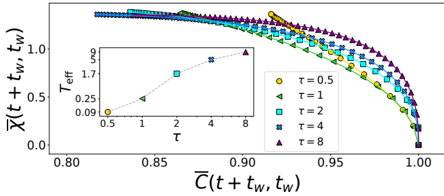
Figure 2.3.2 – FDT plot for p-SGD . We consider \alpha = 8, \Delta = 1, \lambda = 1 , where the classification problem is UNSAT and we use dt = 0.05 . We consider different persistence times \tau = 0.5, 1, 2, 4, 8 and fixed batch size b = 0.3 ( top panel ), and different b = 0.1, 0.2, 0.4, 0.8, 0.99 and fixed \tau = 2 ( bottom panel ). The insets display the effective temperature, numerically estimated, as a function of the persistence time ( top panel ) and batch size ( bottom panel ).
