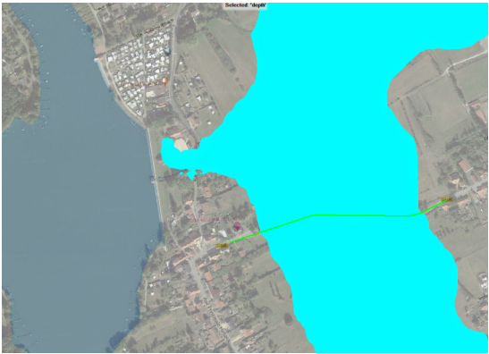
Figure C.6: HEC-RAS simulation with the filled DEM.
