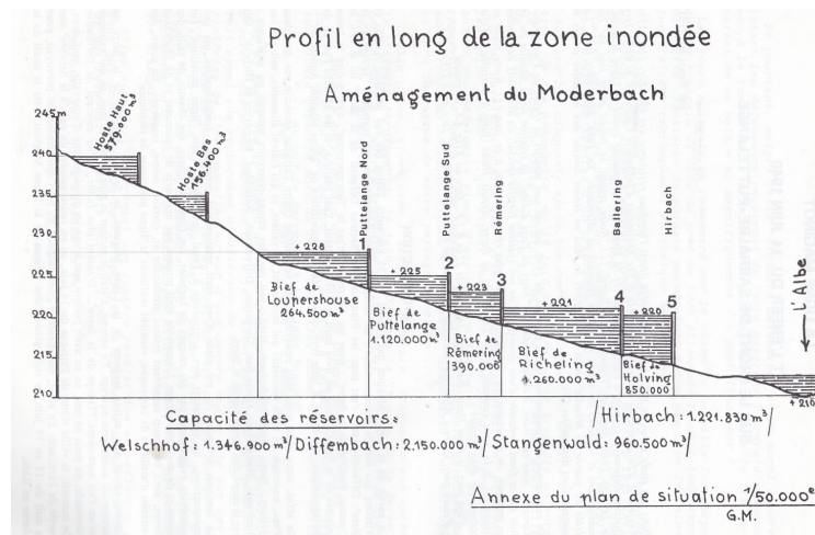
Figure 5.18: Dams and ponds of the Maginot line in the Moderbach basin (Marque, 1989).
