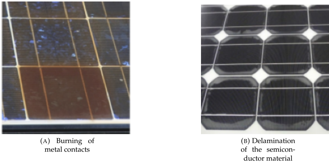
FIGURE 2.9: Effects of thermal stress in a PV cell
