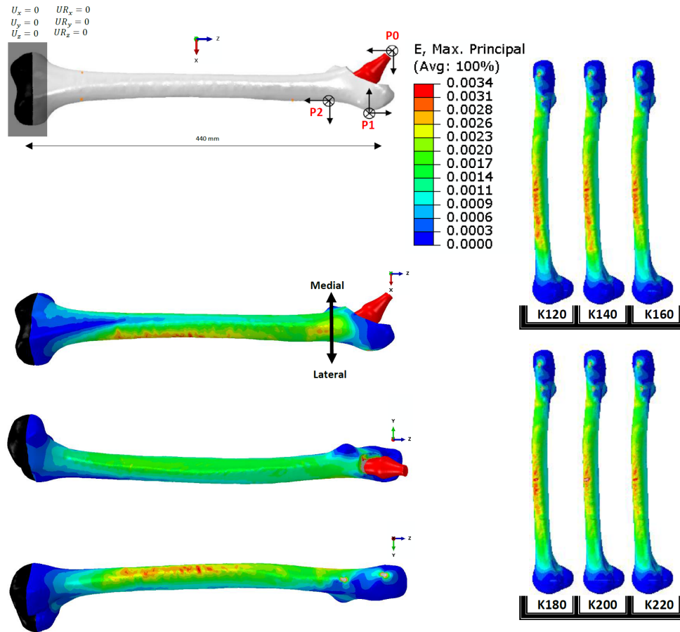
Figure 3.4.7: Max principal strain distribution obtained in the several modes during the gait cycle during walking activity.
