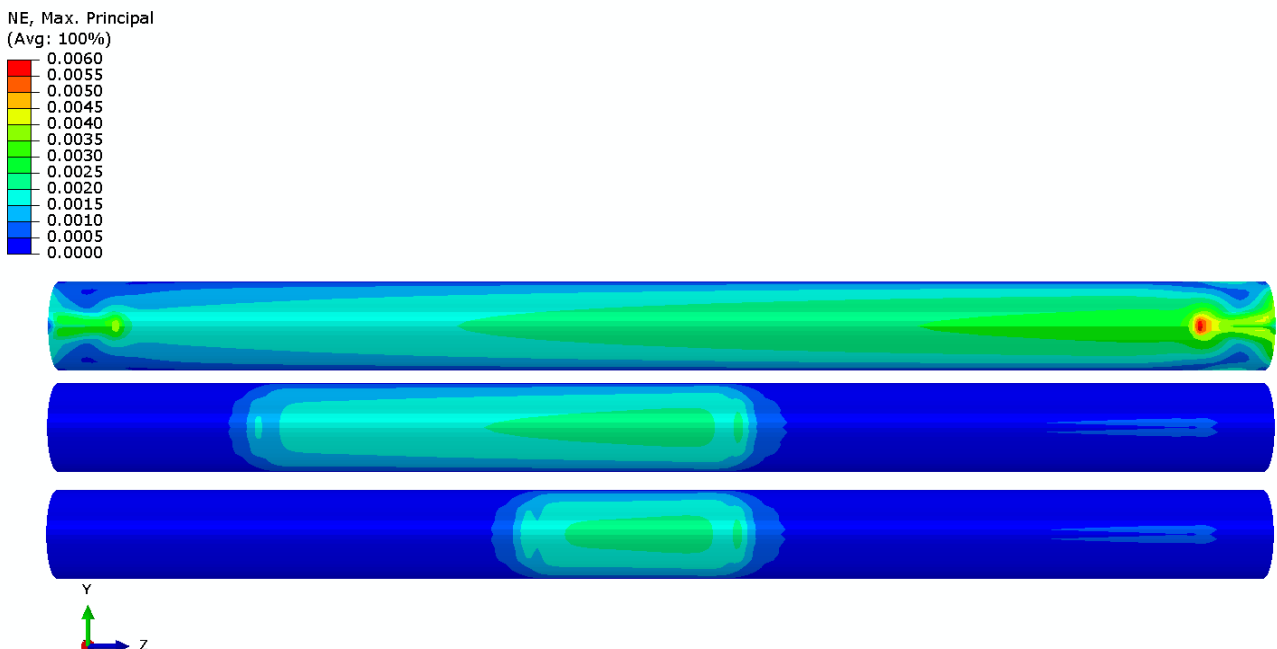
Figure 4.5.1: Maximum principle strains distribution under the two-point bending test : (A) represent the cylindrical tube model without any prostheses, (B) represent the cylindrical tube model with the presence of hip prosthesis and knee prosthesis of 70 mm in length, (C) represent the cylindrical tube model with the presence of hip prosthesis and knee prosthesis of 145 mm in length
