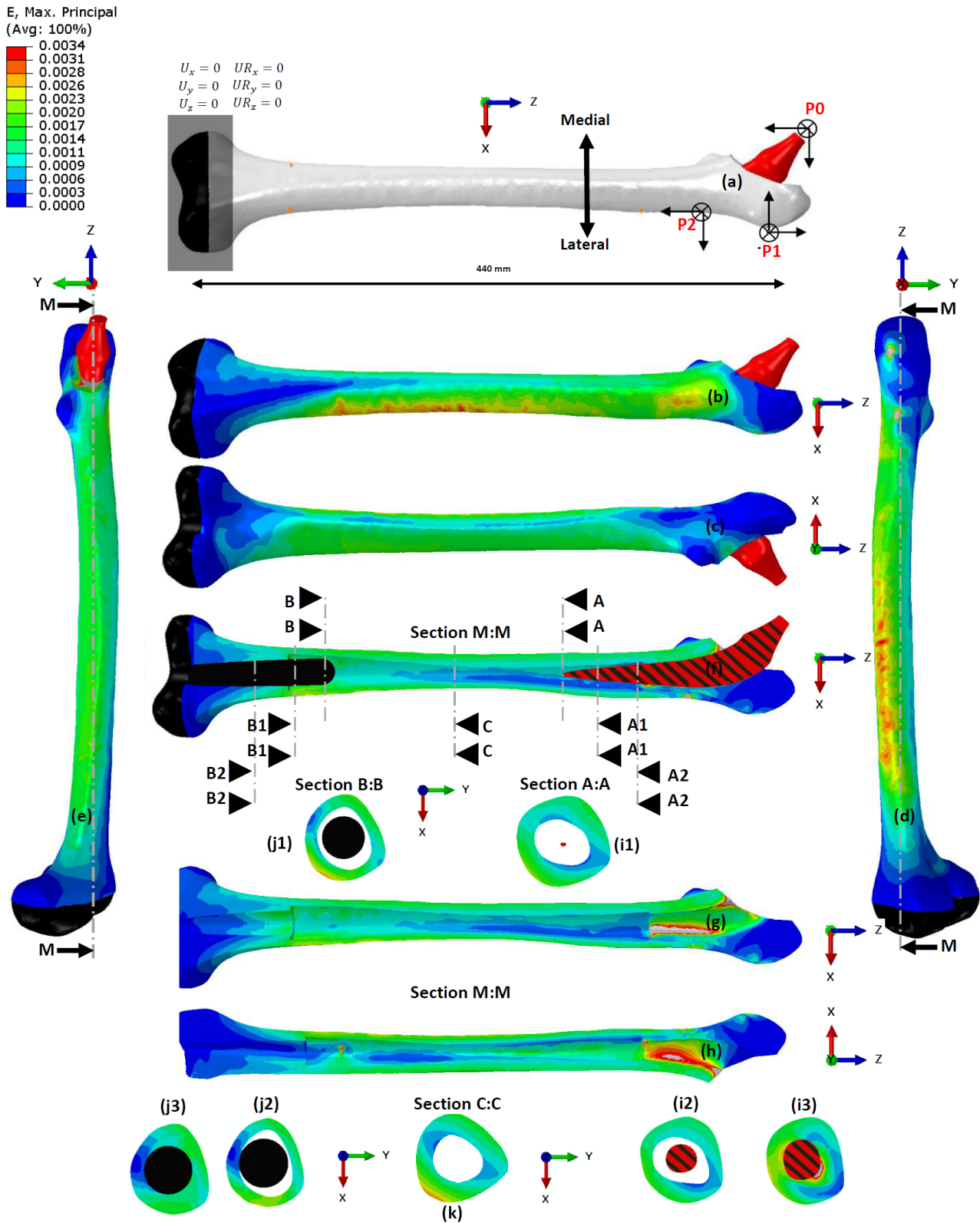
Figure 3.4.8: Maximum principle strain values on the lateral side of the femur (Four-point bending test with a constant moment throughout the total femur). (a) represents the boundary conditions of the four-point bending test with a constant moment throughout the femur diaphysis. (b) represents the maximum principle strain on both of the femur and prostheses. (c) represents the maximum principle strain distribution on the femur only, while the colors for hip and knee prostheses do not follow the deformation legend. (d) represents the deformed femur after the four-point bending test while the cuts to represent the three different parts of the femur: deformation of the proximal side, middle shaft and distal side. (f1) a cross-section represents the deformation on the tip of the hip prosthesis. (f2) a cross-section represents the deformation on the cortical bone due to the existence of the hip prosthesis. (f3) a cross-section represents the full contact between the proximal femur and the hip prosthesis. (g1) a cross-section represents the deformation on the tip of the knee prosthesis. (g2) a cross-section represents the deformation on the cortical bone due to the existence of the knee prosthesis. (g3) a cross-section represents the full contact between the distal femur and the knee prosthesis. (h) represents the maximum deformation on the femur shaft. (i1, i2) represents the deformation on the lateral and medial sides of the femur
