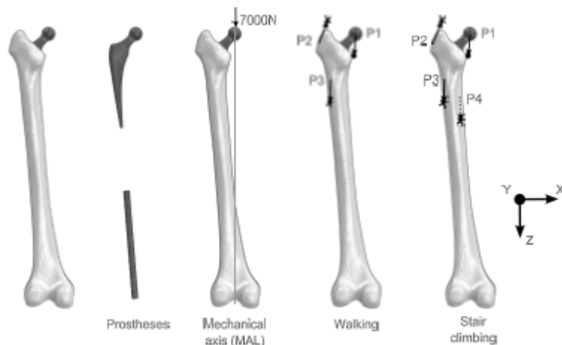
Figure 1.9.3: : Finite element models representing three different loadings; load along the mechanical axis of the femur, walking and stair climbing by [Quiryneen, 2016]
