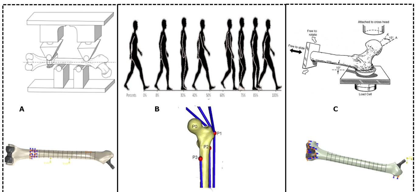
Figure 1.9.2: Finite-element model represent the experimental setup for "A. four-point bending, B. gait cycle loading and C. sideways falling test by [Soenen et al., 2013]"
