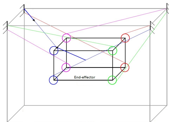
FIGURE 2.12 – RPC suspendu redondant MiCaRo [WEBER, 2016]
