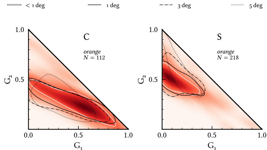
Figure 7.4: Effects of insufficient phase curve coverage on the phase curve coefficients G_1 , G_2 . The red distributions show the 2D Kernel Density Estimation distributions fitted to the G_1 , G_2 parameters of complete phase curves of C- and S-type asteroids. The white contours give the 1-level of kernel density estimators. The solid black (dash dotted, dotted) contour gives the 1-level of the fitted probability densities corresponding to the G_1 , G_2 parameters of the phase curves truncated at 1 deg (3 deg, 5 deg). Published in Mählke et al. (2021).
