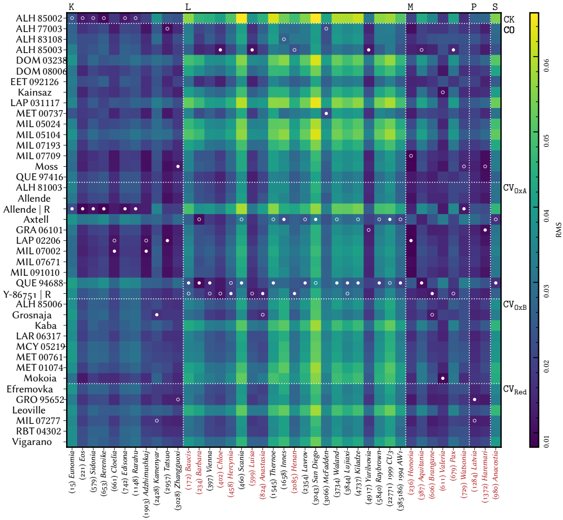
Figure 14.6: Root mean square differences between CV, CO chondrites and K-, L-types and Barbarians. White, filled circles give the best matching meteorite for each asteroid, open circles indicate the second-best match. Asteroids with red labels are Barbarians.
