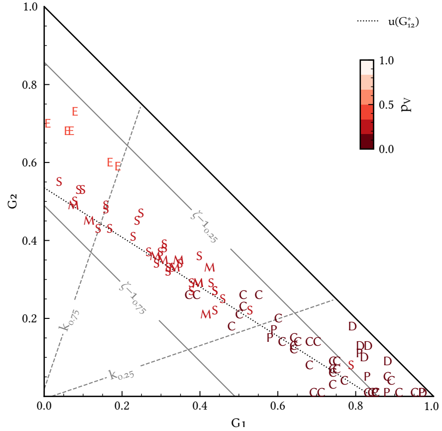
Figure 2.4: The G_1 , G_2 parameter space related to the photometric slope, opposition effect, and taxonomic classes. The dashed lines show 25- and 75-percentiles of the photometric slope k . As the slope is negative, the phase curve becomes steeper towards the smaller percentiles. The solid lines give the size of the opposition effect \zeta - 1 , again for the 25- and 75-percentiles. Further shown are the coefficients of targeted phase curves presented in Shevchenko et al. (2016), where the position of the G_1 , G_2 -parameters is indicated by the taxonomic class of the respective asteroid.
