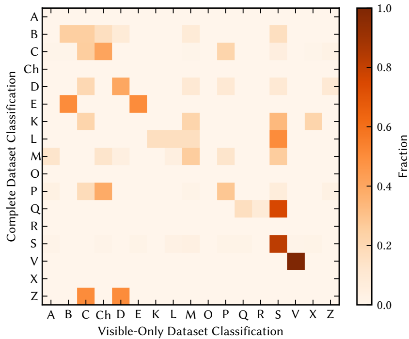
Figure 12.4: Comparison of the classifications of 328 samples of 267 individual asteroids resulting from visible-only spectra with 81.4% observed albedos to the classifications of the same asteroids resulting from the complete sample classifications. Note that the sample sizes per row differ: the intersection of asteroids present in both datasets gives 2 samples classified as E using complete samples as well as 2 samples classified as Z, while there are 140 samples entering the calculation in the row of S-types. No A-, O-, or X-types are present in both samples.
