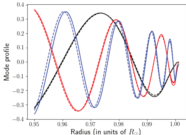
Fig. 3. Eigenfunction \Psi(r) of several radial acoustic modes (black: n = 10 ( \nu_0 = 1.580 mHz); red: n = 20 ( \nu_0 = 2.912 mHz); blue: n = 30 ( \nu_0 = 4.267 mHz)) as computed by our model (solid lines), and calculated using the ADIPLS code (dashed lines). The radial axis is zoomed to show only the outermost region. The eigenfunctions have been normalised so that their maximum over the entire solar interior equals 1.
