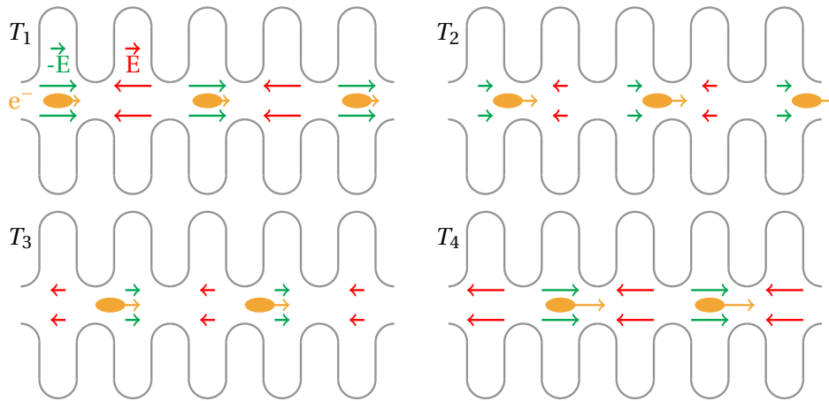
Figure 1.7: Sketch of relativistic electron beam propagation inside an RF section for different time : T_1 < T_2 < T_3 < T_4 .
