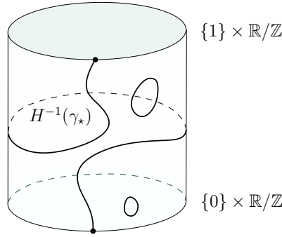
FIGURE 4.3 – Proof of Lemma 4.4.3. The path linking (0, [0]) \in \{0\} \times \mathbb{R}/\mathbb{Z} to (1, [0]) is the image of F .
