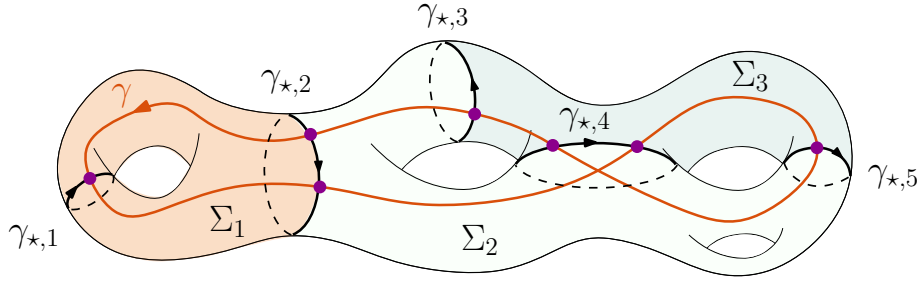
FIGURE 2.2 – A closed geodesic \gamma on \Sigma . Here we have r = 5 , q = 3 , and \omega(\gamma) \sim (u, v) where u = (1, 2, 4, 5, 4, 3, 2) and v = (1, 1, 2, 3, 2, 3, 2) (the starting point of \gamma is the red arrow).
