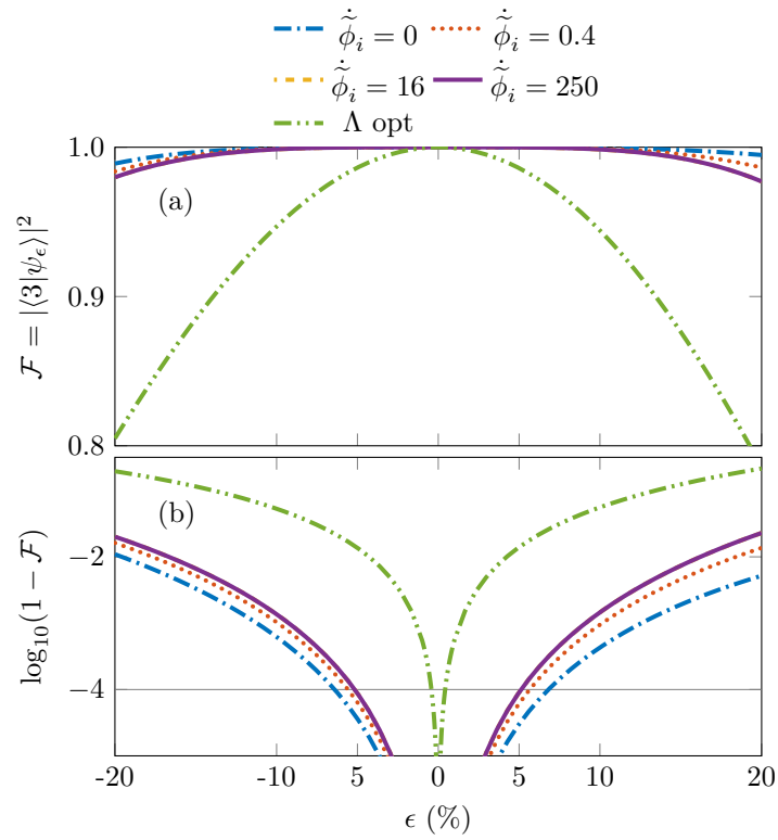
Figure 5.3: Fidelity (a) and logarithm base 10 of the infidelity (b), for the selected optima highlighted in Fig. 5.1 (with trajectories and control fields in Fig. 5.1) with numeric data summarized in Table 5.1, and for the \Lambda transfer optimized with no constraints of robustness, with respect to the pulse area scaling error \epsilon . The thin horizontal gray line denotes the ultrahigh-fidelity benchmark of 10^{-4} infidelity.
