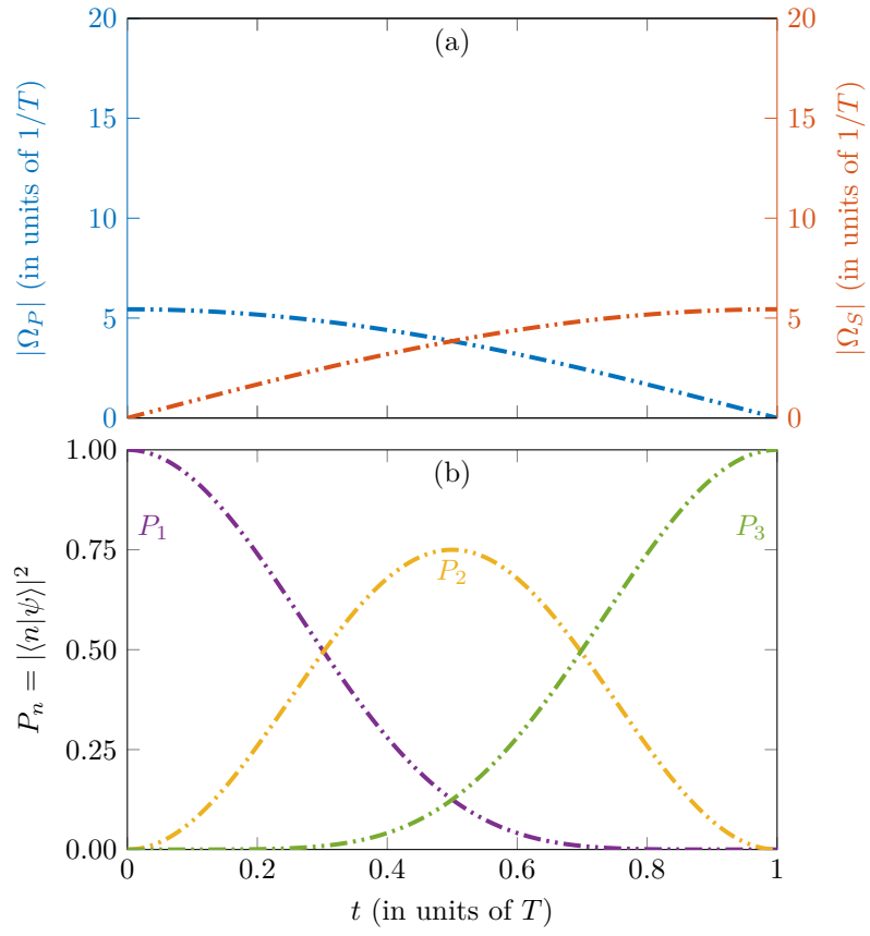
Figure 5.4: Fields and populations vs time for the unconstrained optimum \Lambda transfer. Numerical parameters details are summarized in Table 5.1.
