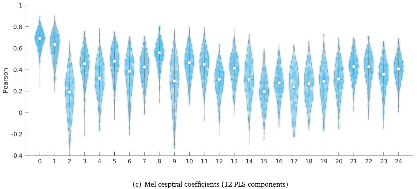
Fig. 4.9.: Decoding of acoustic features of speech with PLS regression from EC61 dataset. PLS regressions with 12 and 18 components were trained to predict mel cepstral coefficients and F0 from neural features. Statistical significance of decoding with 12 vs 18 components was assessed by a Wilcoxon signed-rank test. (a) Correlations of decoded mel cepstrum with matching ground truth using 12 and 18 PLS components (median correlations r_{12} = 0.35 , r_{18} = 0.36 , p = 3.3e^{-35} ). (b) Correlations of decoded F0 with matching ground truth using 12 and 18 PLS components (median correlations r_{12} = 0.51 , r_{18} = 0.49 , p = 3.0e^{-29} ). (c) Correlations of individual mel cepstral coefficients predicted with the 12 components PLS. n.s.: p > 0.05 , *: p < 0.05 , **: p < 0.01 , ***: p < 0.001
