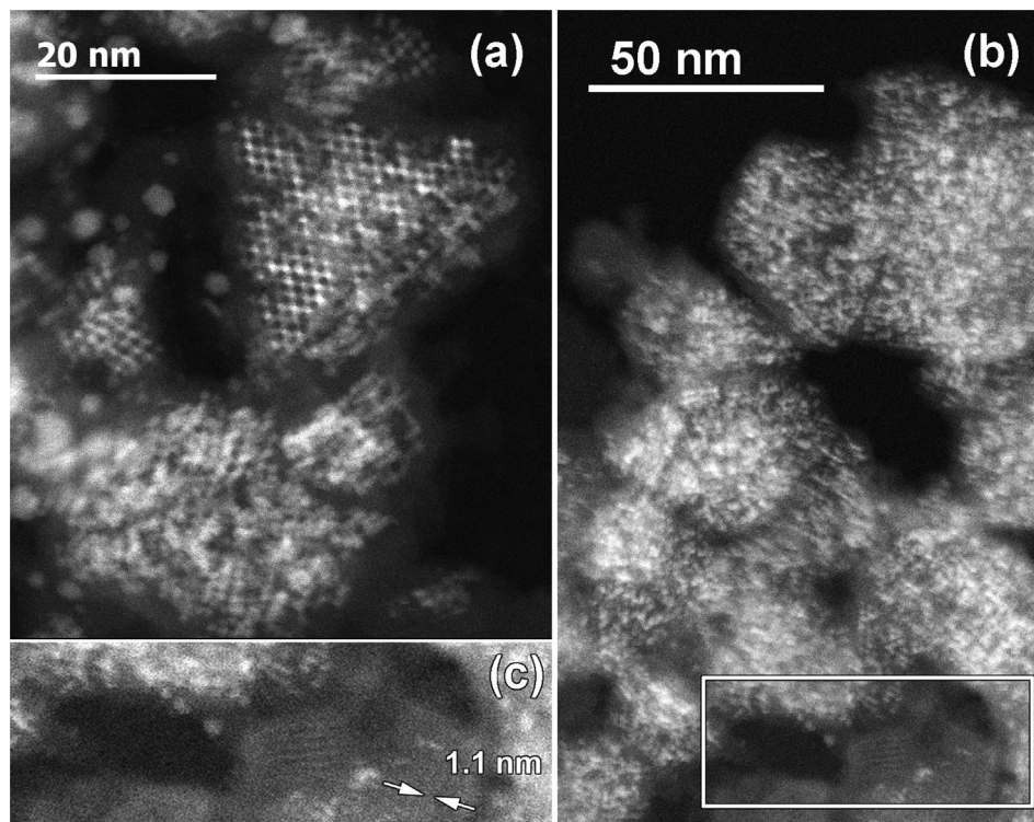
Fig. 2. (a) HAADF-STEM images of Ag@ZX-V nanoparticle close to [0 0 1] zone axis. Triangle shape and Ag filled with an evident hexagonal arrangement of the channels. (b) HAADF-STEM image of Ag@ZX-V in the presence of non-loaded FAU nanoparticle marked by a white rectangle. The contrast is very low due to the presence only relatively light elements in zeolite (Si, O). (c) Enlargement image of selected in (b) non-loaded FAU nanoparticle with resolved lattice planes.
