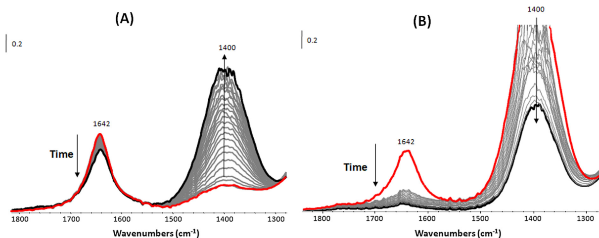
Fig. 8. IR spectra of Ag@ZX-V sample recorded during the SCR-NH 3 reaction at (A) RT and (B) T = 150 °C under visible irradiation (photo-assisted SCR-NH 3 ). Reaction conditions: 7 spectres/min; m cat = 20 mg; Lamp Xe; λ > 390 nm; irradiance = 110 mW/cm 2 ; T = 25 °C; gas mixture: 150 ppm of NO x , 150 ppm of NH 3 , 667 ppm of CO, 5% CO 2 , 10% O 2 , 50 ppm of HC and 2% of water; Total flow = 31 cc min -1 .
