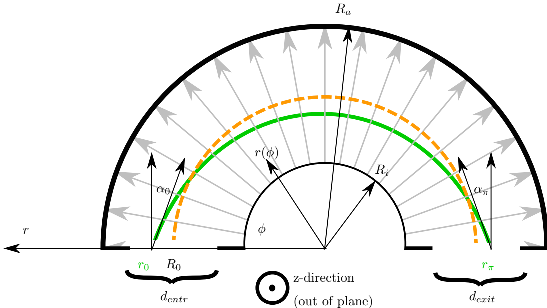
FIGURE 2.5 – Schematic cross-section through a hemispherical analyzer along the dispersive (r, \phi) plane. The grey lines indicate the direction of the electric field. The outer wall is of radius R_a whereas the inner wall is of radius R_i set at a higher electrostatic potential. An electron enters within the slit width d_{entr} at position r_0 under entrance angle \alpha_0 ( \beta_0 , out-of-plane, not shown), follows the schematic trajectory in green (not exact) and leaves at position r_\pi at exit angle \alpha_\pi ( \beta_\pi , not shown) within the slit width d_{exit} . Taken and adapted from [157]
