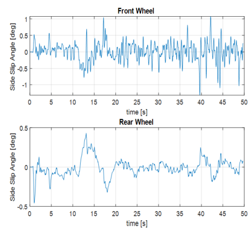
Figure 2.8. Side slip angle for the front and rear wheel.
