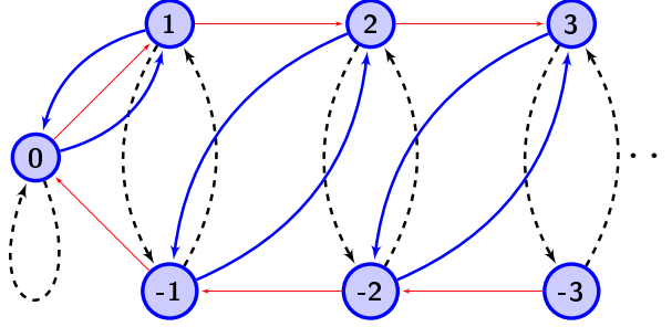
FIGURE 1. (A portion of the) Schreier graph of D_\infty for the subgroup \{e, x\} with x (dashed, black), y (blue) and a (thin, red). We will consider it with the generating set \{x, y\} (without the red lines)
