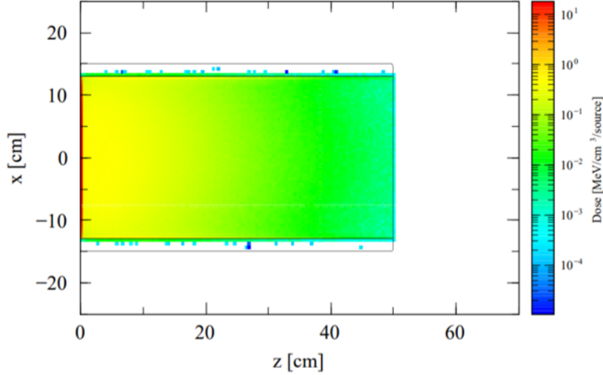
Figure 4.7: Energy deposition of ^{133}\text{Xe} in the detector per volume.
