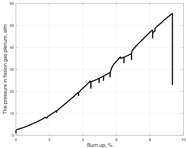
Figure 4.3: The pressure in fission gas plenum in operating condition.
