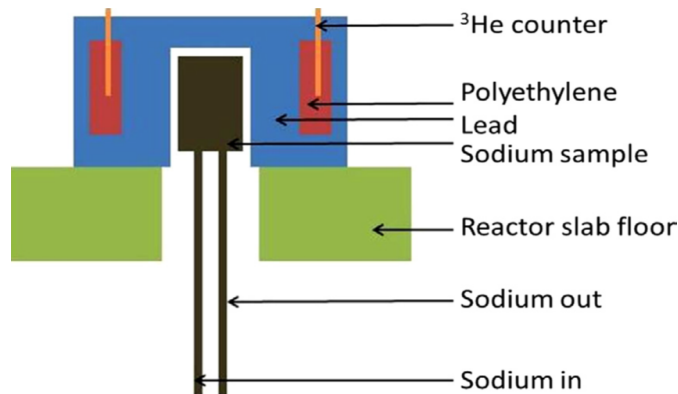
Figure 2.8: DND system schematic view [115].
