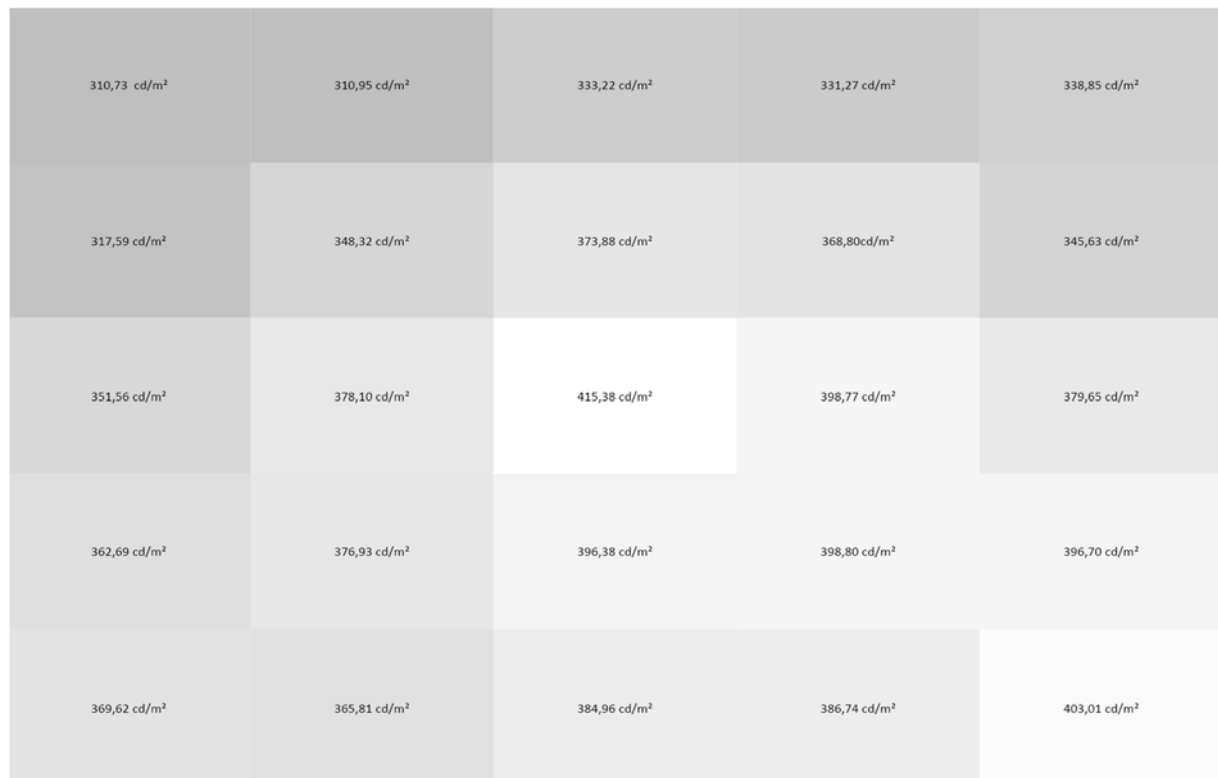
Figure 34. Visualization of the measured luminance differences at 100% for Display 1.
