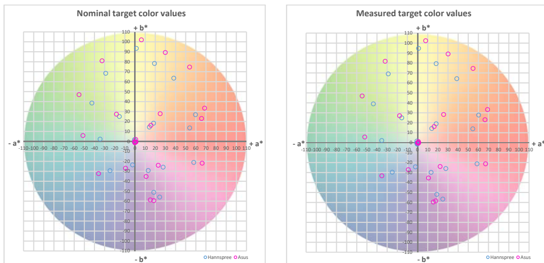
Figure 78. Plot of color locations of the nominal color values (left) and the averaged spectral values (right) for displays 1 and 2 in the a^*b^* plane (CIE Lab 1976).
