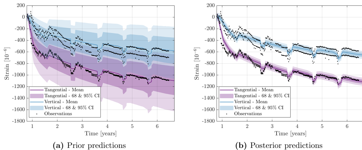
Figure 4.34: Prior and posterior strain predictions after updating at VD3 test.
