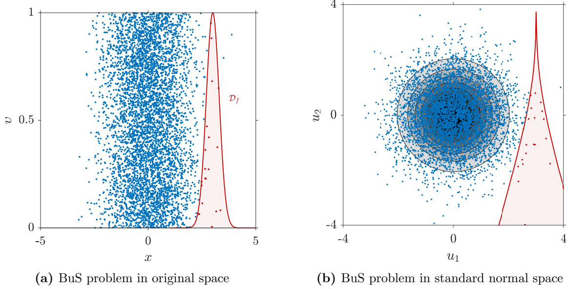
Figure 2.2: BuS in standard normal space: illustration in the case presented in Fig. 2.1.
