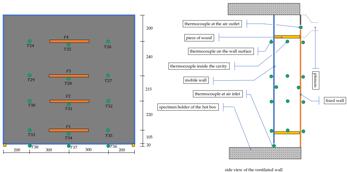
Figure 2.19 Instrumentation du mur mobile.
