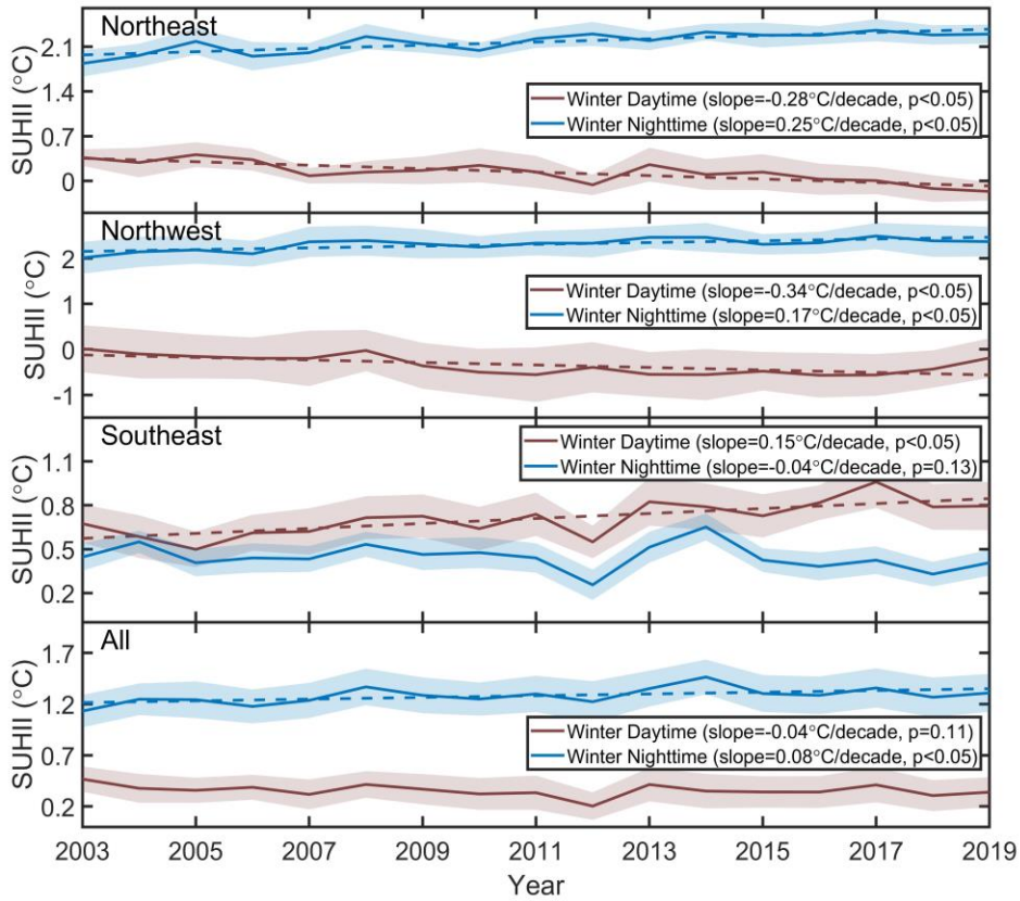
Figure 5.14 Inter-annual variations of winter daytime and nighttime SUHII for 34 China cities in different regions over the period 2003-2019. The solid line depicts the mean value of each year, and its standard errors are in shaded patch. The Sen's slope is calculated at 95% significant interval. The variations with significant trends are delineated in dashed line.
