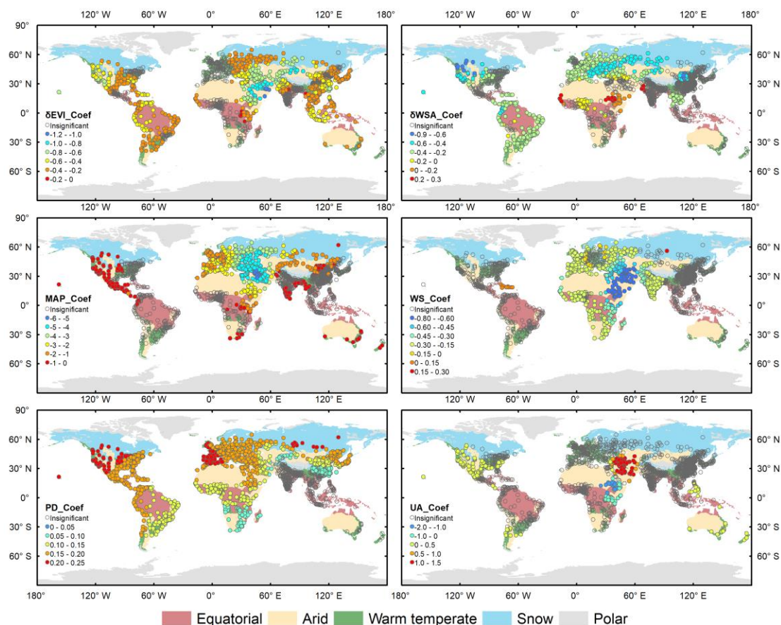
Figure 4.9 The spatial variation of coefficients of multi-independents for summer nighttime SUHII.
