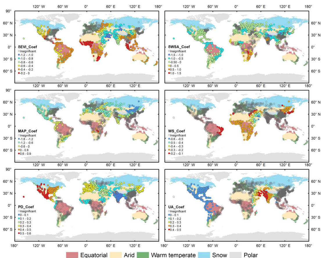
Figure 4.7 The spatial variation of coefficients of multi-independents for annual nighttime SUHII.
