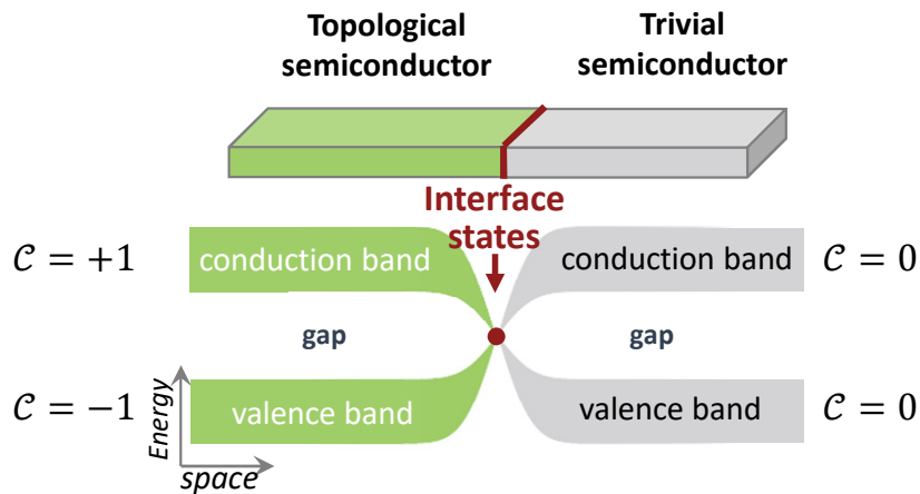
Figure 1.2: Formation of states in the gap at the interface of two materials whose bands possess different topological invariants.
