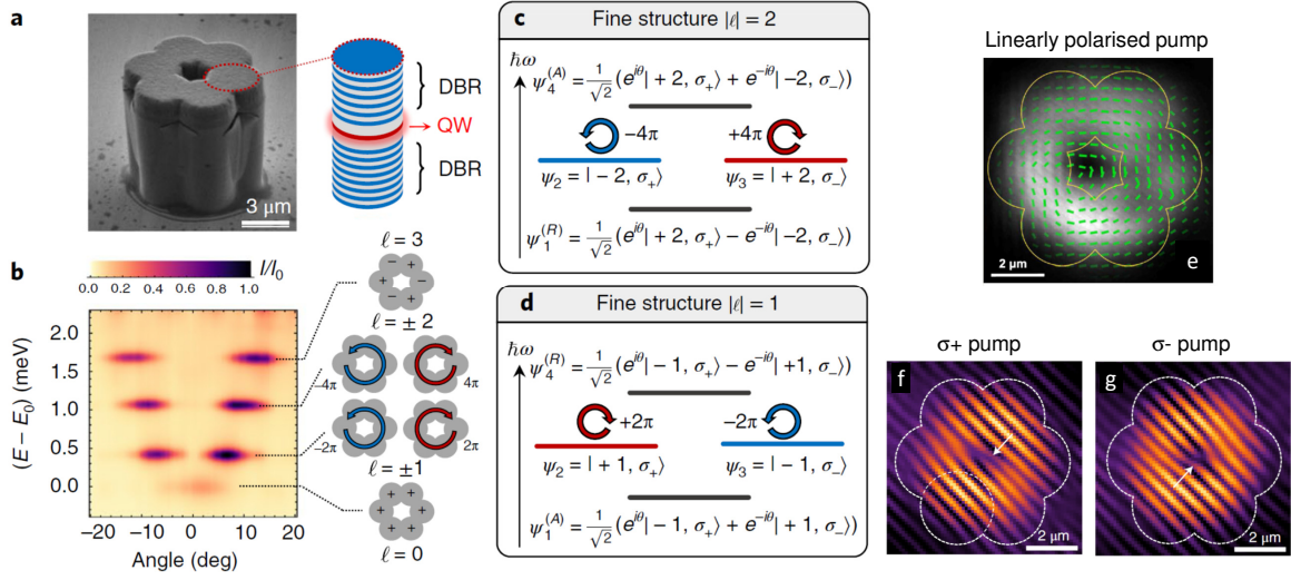
Figure 2.2: (a) Scanning electron microscope image of a hexagonal molecule of coupled polariton micropillars. (b) Energy and angle resolved photoluminescence of the lowest energy molecular modes and orbital scheme of the eigenmodes in the absence of spin-orbit coupling. E_0 = 1469.7 meV. (c) Fine structure of the \ell = \pm 2 manifold. (d) Fine structure of the \ell = \pm 1 manifold. \theta = 2\pi/6 . (e) Real space image of the emission from the lasing mode \psi_1 of the \ell = \pm 1 manifold under linear polarised pumping. Green segments show the measured direction of linear polarisation. (f)-(g) Emission of the lasing mode in modes \psi_2 and \psi_3 of the \ell = \pm 1 manifold under circularly polarised \sigma_+ and \sigma_- pumping, respectively. The observable fringes arise from the interference between the emission and a reference beam of the exact same frequency. They allow evidencing the orbital chirality of the modes via the presence of a phase dislocation at its center. (a)-(d) and (f)-(g) are extracted from Ref. [115] and measured in a microcavity with an InGaAs quantum well. (e) is extracted from Ref. [108] and measured in a microcavity with 12 GaAs quantum wells.
