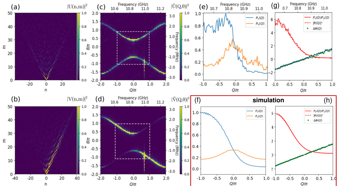
Figure 5.3: (a)-(b) Spatio-temporal dynamics measured in the u and v rings for 50/50 beamsplitter and \varphi_m = 0 for excitation in the v ring with a single pulse. (c)-(d) Band structure computed from the Fourier transform of (a) and (b). The dashed rectangle displays the first Brillouin zone. (e) Measured amplitude square of the eigenvectors in each ring as a function of the quasi-momentum for the upper band. (f) Same as in (e) extracted from the simulations of Eq. 5.1. (g) Red line: measured ratio of the amplitude square v(k)/u(k) in the upper band. Green line: measured relative phase \phi(u(k)) - \phi(v(k)) in the upper band. (h) Ratio of amplitudes and phase difference in the upper band computed from simulations of Eq. 5.1. Adapted from Ref. [205].
