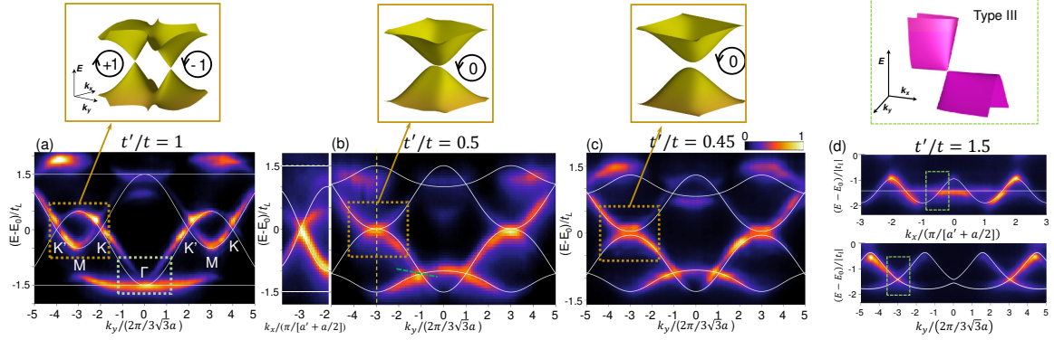
Figure 4.3: (a)-(c) Measured dispersion of the bulk p bands for different values of the engineered strain when t' is reduced. In all images, k_x = 2\pi/(a' + a/2) , where a and a' are the unstrained and strained interpillar distances shown in Fig. 4.1(a). The orange rectangle shows the merging of Dirac cones and gap opening (see calculated tight binding bands in the upper panels). In (b) and (c) the strain results in the emergence of tilted Dirac cones in the lowest two bands. (d) Measured dispersions for t' > t (upper panel: k_y = -2\pi/(\sqrt{3}a) , lower panel k_x = -0.5 \times 3\pi/(3a) ). Both dispersions cross at the type-III Dirac point highlighted in the dashed green box. The upper inset shows the tight-binding dispersion of the type-III Dirac cone. Adapted from Ref. [182].
