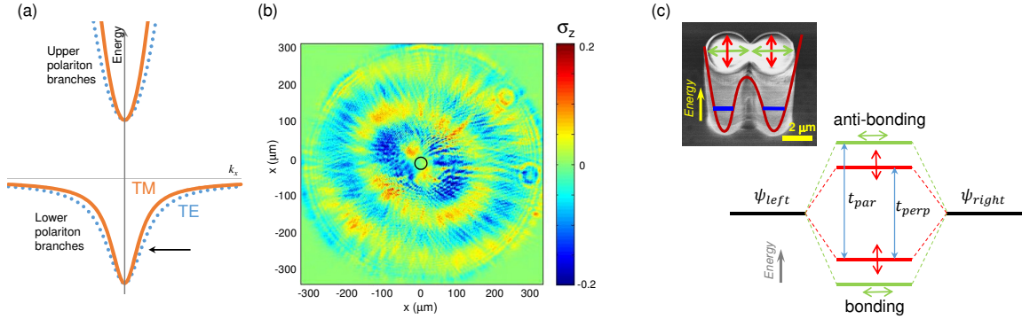
Figure 2.1: (a) Computed polariton dispersion of a planar microcavity as a function of k_x for k_y = 0 including the TE-TM linear polarisation splitting. (b) Measured degree of circular polarisation \sigma_z of a polariton condensate expanding from an injection area marked by a circle at (x, y) = (0, 0) . The condensate is formed under non resonant excitation with a linearly polarised laser. Due to interactions with the reservoir, the condensate energy is 2 meV above the bottom of the lower polariton band. At the excitation point the condensate is linearly polarised. The polarisation precesses when propagating due to the presence of the TE-TM splitting, resulting in "waves" of circular polarisation. (c) Scheme of the effect of TE-TM splitting on a polariton molecule: the effective hopping is different for linear polarisations parallel (green arrows) and perpendicular (red arrows) to the link between the pillars.
