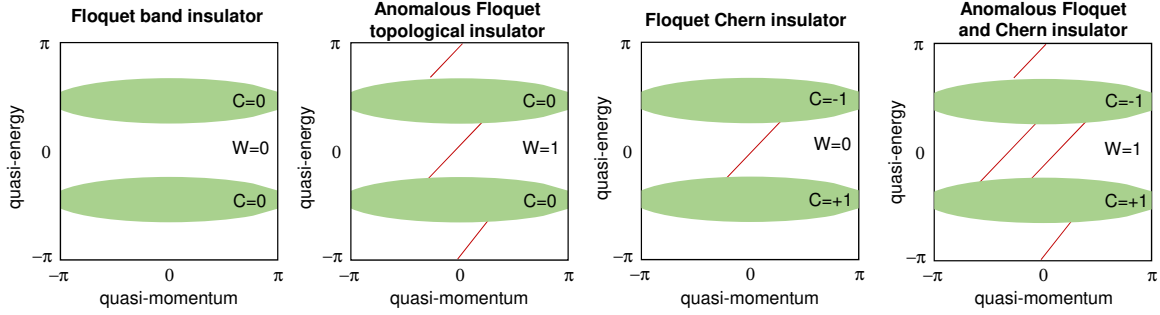
Figure 5.1: Examples of two-dimensional two band systems with Floquet-Bloch periodicity. Due to the periodic time modulation of the system the top and bottom parts of the quasi-energy spectrum fold into each other. Bands are represented in green, gaps in white and edge states in red. C indicates the Chern number of the bands and W the Floquet winding number of the middle gap.
