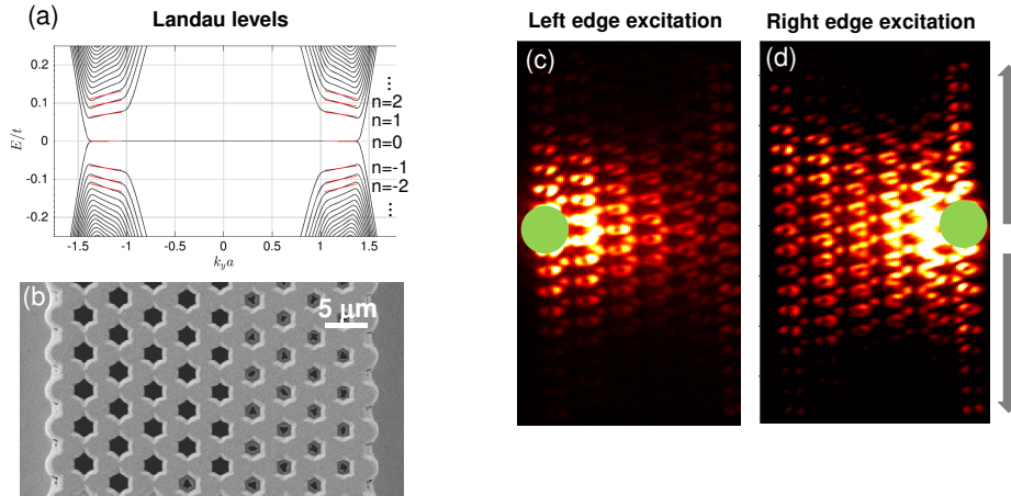
Figure 4.4: (a) Calculated energy bands of a ribbon presenting a linear gradient of hoppings along the x direction using the tight-binding method [189]. (b) Scanning electron microscope image of a polariton lattice implementing a linear gradient of hoppings in the x direction. (c), (d) Photoluminescence at the energy of the propagating edge states in between the n = 0 and n = -1 Landau levels of the p bands. When exciting the right edge, propagation along two helical edge modes is observed (d). Edge propagation is absent in the left edge (c). From Ref [190].
