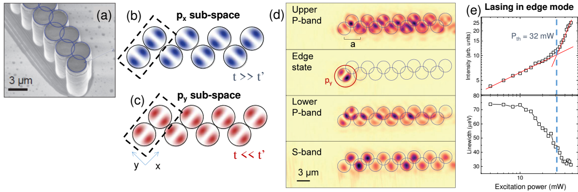
Figure 3.3: p -orbital SSH lattice. (a) A zigzag lattice of coupled micropillars. (b)-(c) Representation of the sub-spaces made of p_x and p_y orbitals. (d) Measured spatially resolved emission at the energies of the top of the s band, top of the lower SSH p -orbital band, topological edge mode in the middle of the gap, top of the upper SSH p -orbital band. (e) Integrated intensity and linewidth of the topological edge mode as a function of excitation power. The lasing threshold is at 32 mW. Adapted from Ref. [31].
