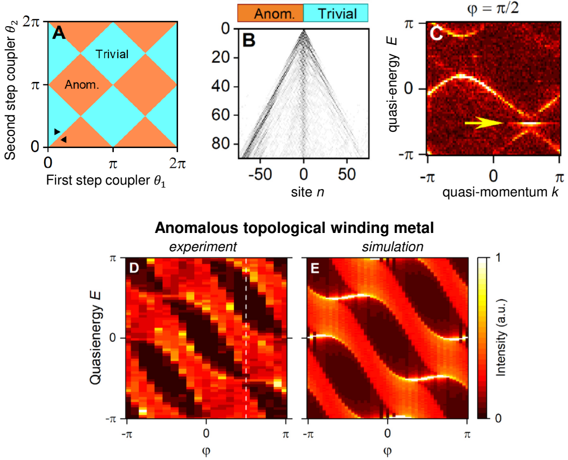
Figure 5.5: (a) Phase diagram of Floquet topological phases as a function of the splitting parameter in the first ( \theta_1 ) and second ( \theta_2 ) steps. (b) Measured spatiotemporal dynamics when injecting a single pulse at the interface between two one-dimensional lattices with different splitting parameters at the two steps, for c_1 = 1 , c_2 = -3 and \varphi = \pi/2 . The splitting parameters are marked with triangles in (a). Localisation of light at the interface unveils the presence of a localised state. (c) Fourier transform of the heterodyned emission shown in (b). The presence of an interface can be identified in one of the gaps (yellow arrow). (d) Measured full band diagram as a function of \varphi . (e) Band diagram from simulations of Eqs. 5.1. Adapted from Ref. [205].
