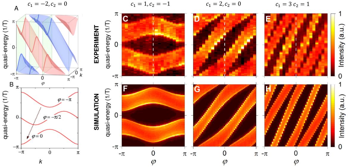
Figure 5.4: (a) Analytically computed two-dimensional band dispersion of a Floquet winding metal. (b) Band dispersions of the red band in (a) for selected values of \varphi . (c)-(e) Measured band dispersions as a function of \varphi for different windings related to the different values of c_1 and c_2 . (f)-(h) Band dispersions obtained from the simulation of the time evolution equations. Adapted from Ref. [205].
