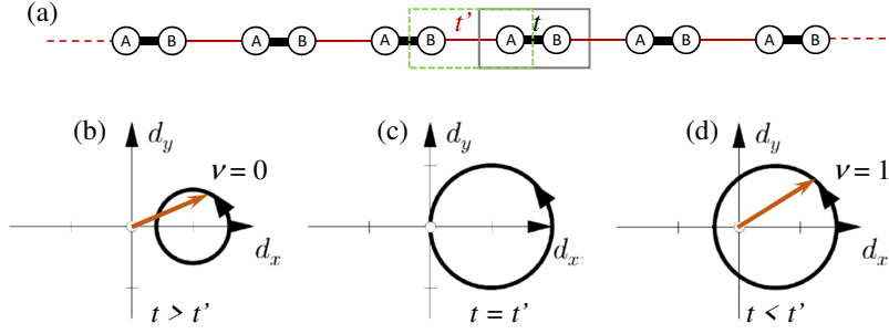
Figure 3.1: (a) Scheme of a lattice of coupled resonators with staggered hoppings t and t' . The two possible choices of unit cell are shown in solid and dashed squares. (b)-(d) Representation of the vector \mathbf{d}(k) in the x-y plane and the closed trajectory it follows when k is scanned between -\pi and \pi for different values of the staggered hoppings.
