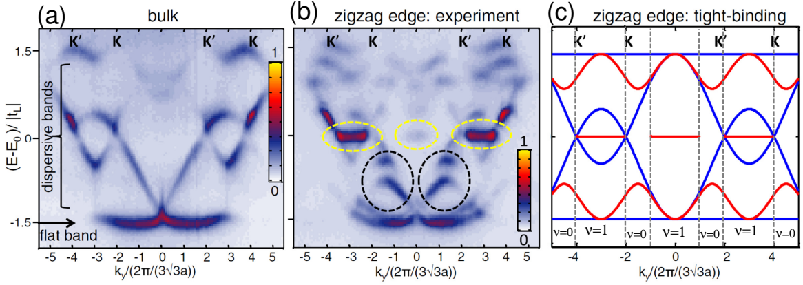
Figure 4.2: (a), (b) Measured photoluminescence dispersion of the p bands as a function of k_y for k_x = 4\pi/(3a) when exciting the bulk of the lattice (a) and the zigzag edge (b). (c) Calculated bands from the tight binding Hamiltonian of a ribbon. Blue lines are bulk modes while red lines are modes localised at the edges [163].
