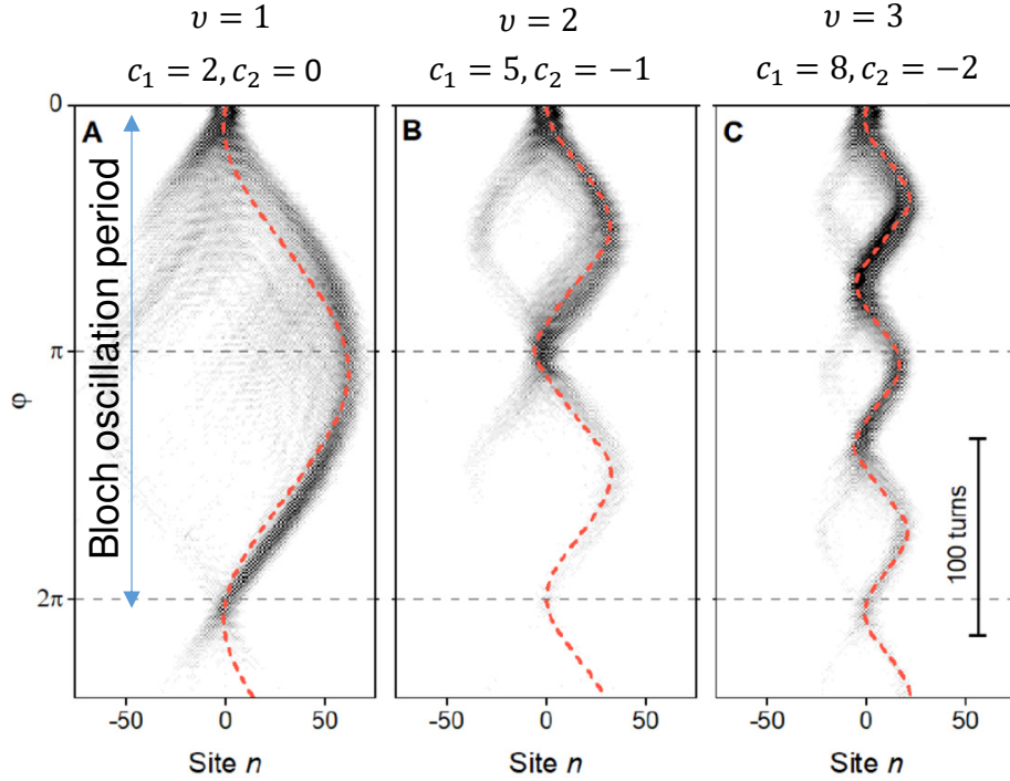
Figure 5.6: (a)-(c) Measured Bloch oscillations when injecting a wavepacket at k = 0 in the upper band and \varphi being linearly increased (left axis). The three panels correspond to three different band windings, mentioned on top of each panel. From Ref. [205].
