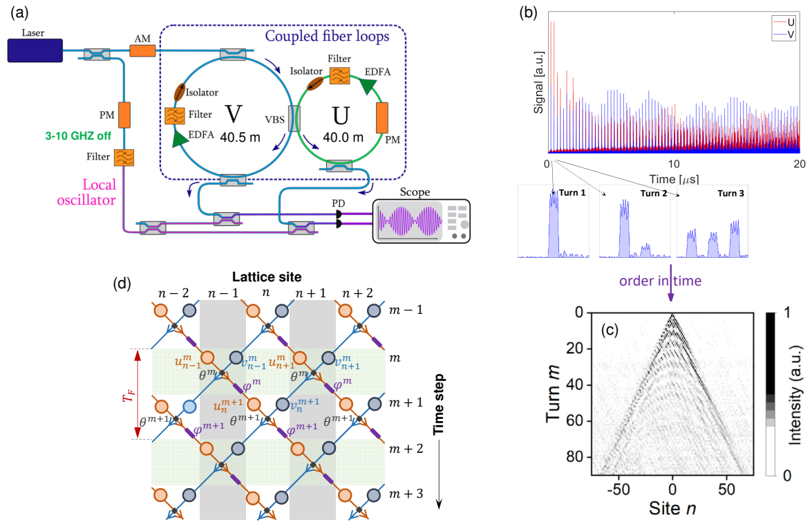
Figure 5.2: (a) Sketch of the two coupled rings setup. AM is amplitude modulator, PM is phase modulator, EDFA is Erbium doped fiber amplifier, VBS is variable beamsplitter and PD is photodiode. (b) Measured train of pulses in the u and v rings (red and blue, respectively) after excitation with a single pulse in the v ring. The inset shows the pulses in the v ring at time positions corresponding to the first three round trips. The oscillations on top of the pulses arise from the interference with the local oscillator. (c) Reconstructed spatiotemporal dynamics in the u ring when stacking the dynamics of each round trip in consecutive lines. (d) One-dimensional lattice subject to coherent split steps to which the dynamics in the double ring systems can be mapped.
