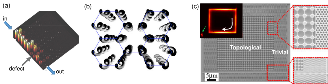
Figure 1.3: Examples of different photonic structures with topological properties. (a) Lattice of coupled ring resonators in Si implemented by the group of M. Hafezi [20]. The imaginary couplings around a plaquette emulate a gauge field resulting in directional edge transport around corners and defects. (b) Sketch of a honeycomb lattice of twisted coupled waveguides that implement the Haldane model for propagating photons, first realised by M. Rechtsman, A. Szameit, M. Segev and coworkers [21]. (c) Topological laser at 1.5\mu\text{m} realised in a photonic crystal with a gyromagnetic material, by the group of B. Kanté [22]. The upper left inset displays the measured light emission, located at the edges between the trivial and topological lattices. Chirality of the emission is demonstrated by the fact that the output waveguide in the lower part of the photonic crystal shows emission mainly in the left region (green arrow).
